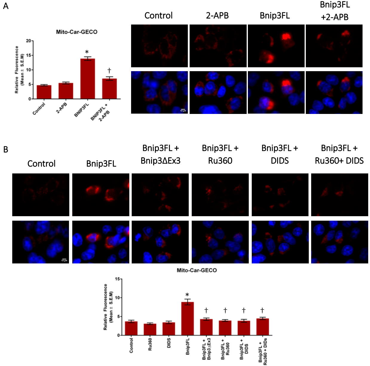
Figure 2 – Bnip3FL-mediated calcium signals require ER and mitochondrial calcium channels
