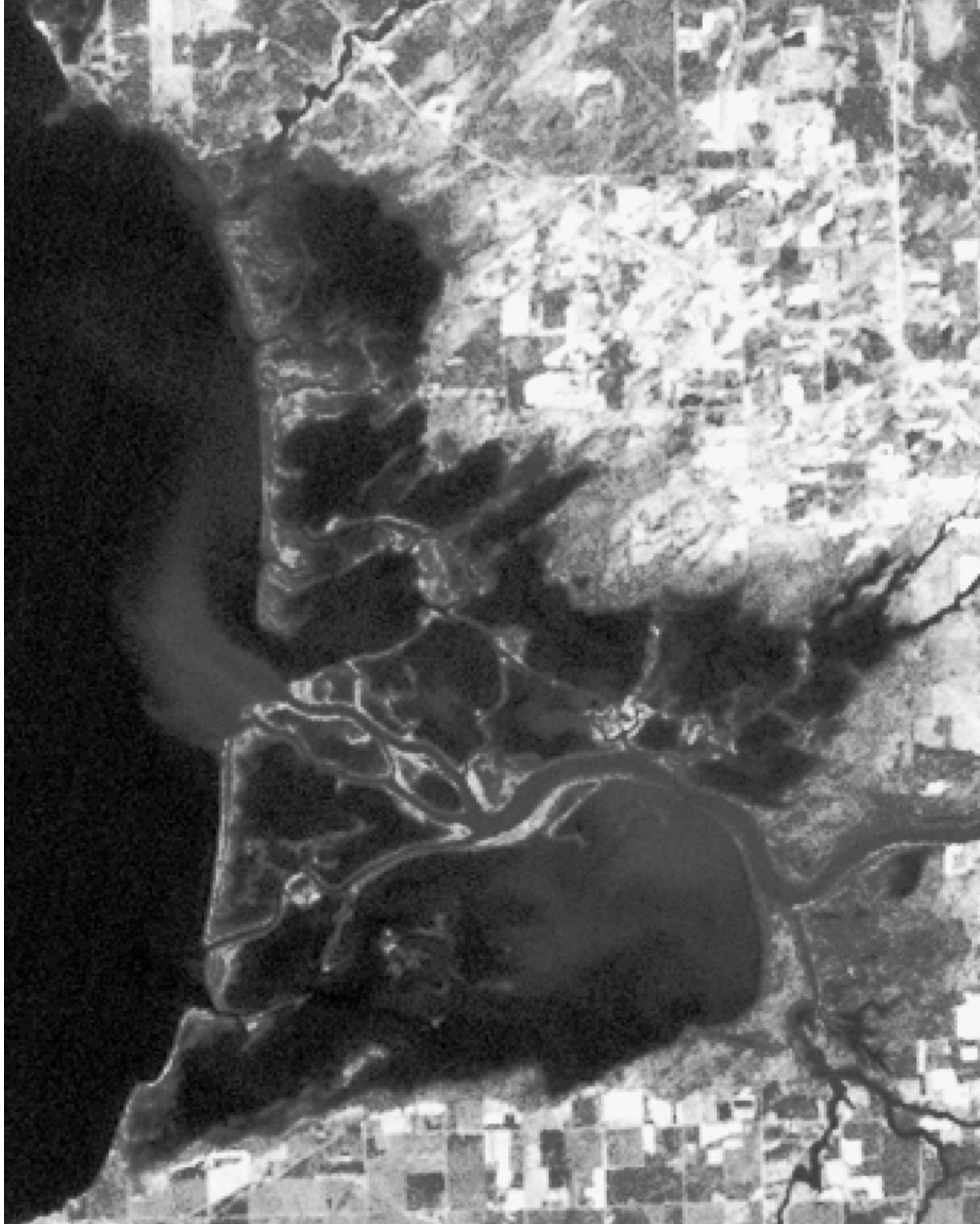
Figure 14. Landsat-7 satellite image of Netley-Libau Marsh, 28 July 1999. The selected band (6H, 60 m ground resolution) shows differences in surface temperature. A light gray, warm-water plume extending through Netley Cut into the darker gray, cooler water of Netley Lake is clearly visible, as is water flowing into Lake Winnipeg from the Red River's main and east channels. Source: Manitoba Lands Inventory (mli.gov.mb.ca), 2004.
