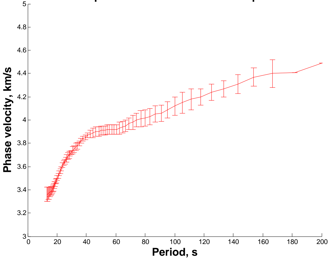
Dispersion curve for DLBC FNBB pair
