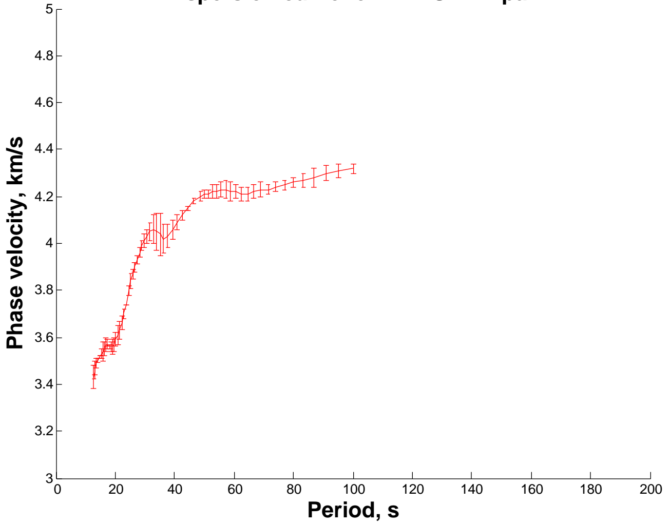
Dispersion curve for INK SMPN pair
