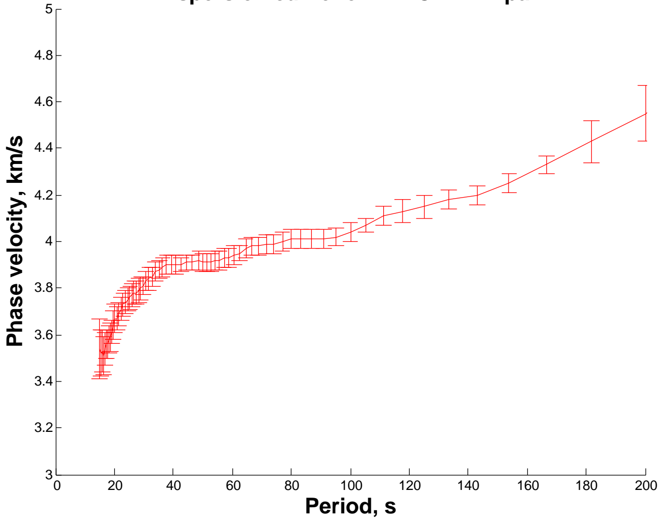
Dispersion curve for PLBC FNBB pair
