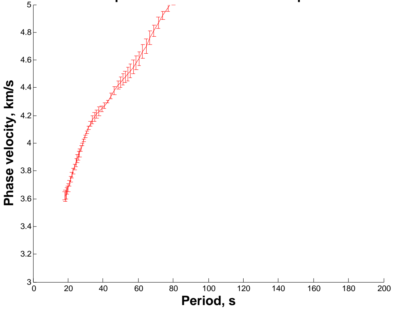
Dispersion curve for PNT PRDA pair
