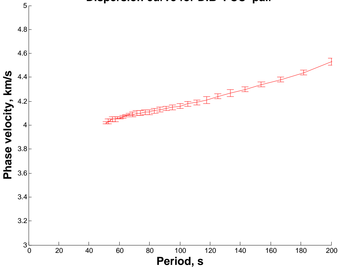
Dispersion curve for DIB FCC pair
