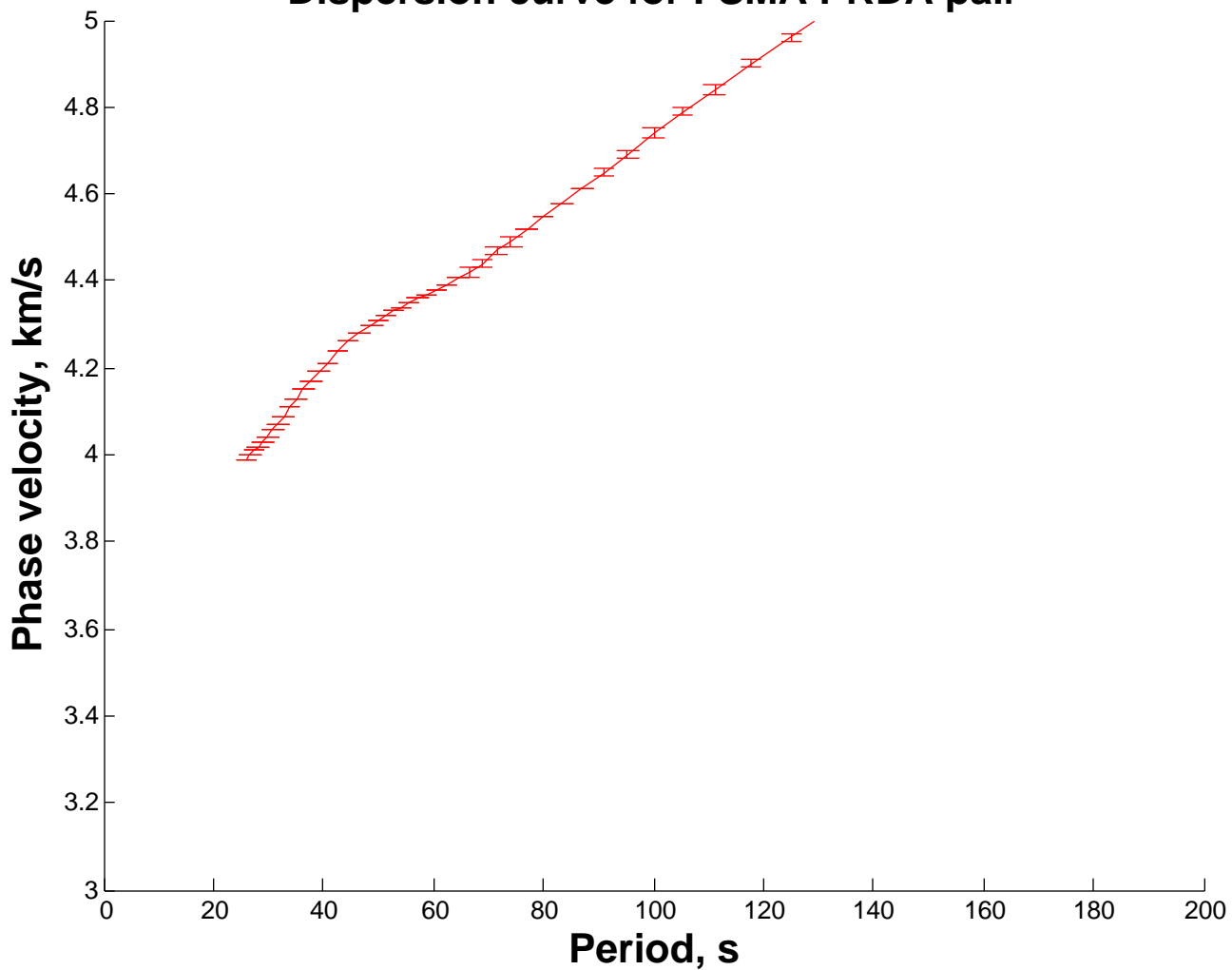
Dispersion curve for FSMA PRDA pair
