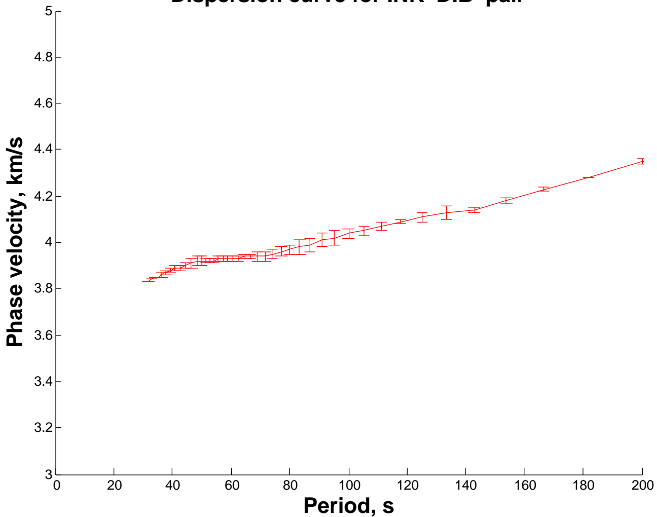
Dispersion curve for INK DIB pair
