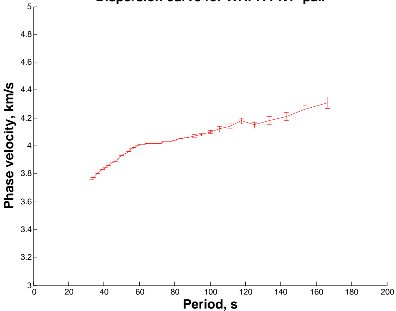
Dispersion curve for WAPA PNT pair
