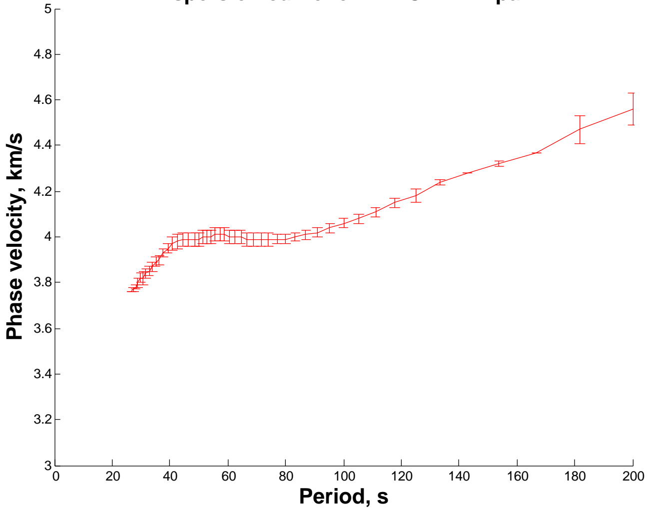
Dispersion curve for PLBC DHRN pair
