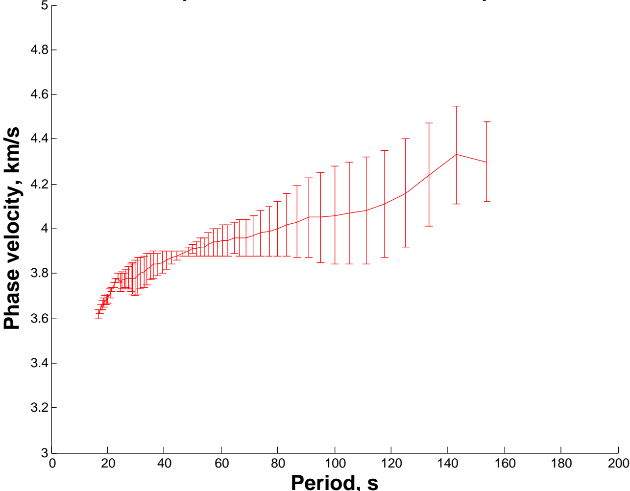
Dispersion curve for BMBC VGZ pair
