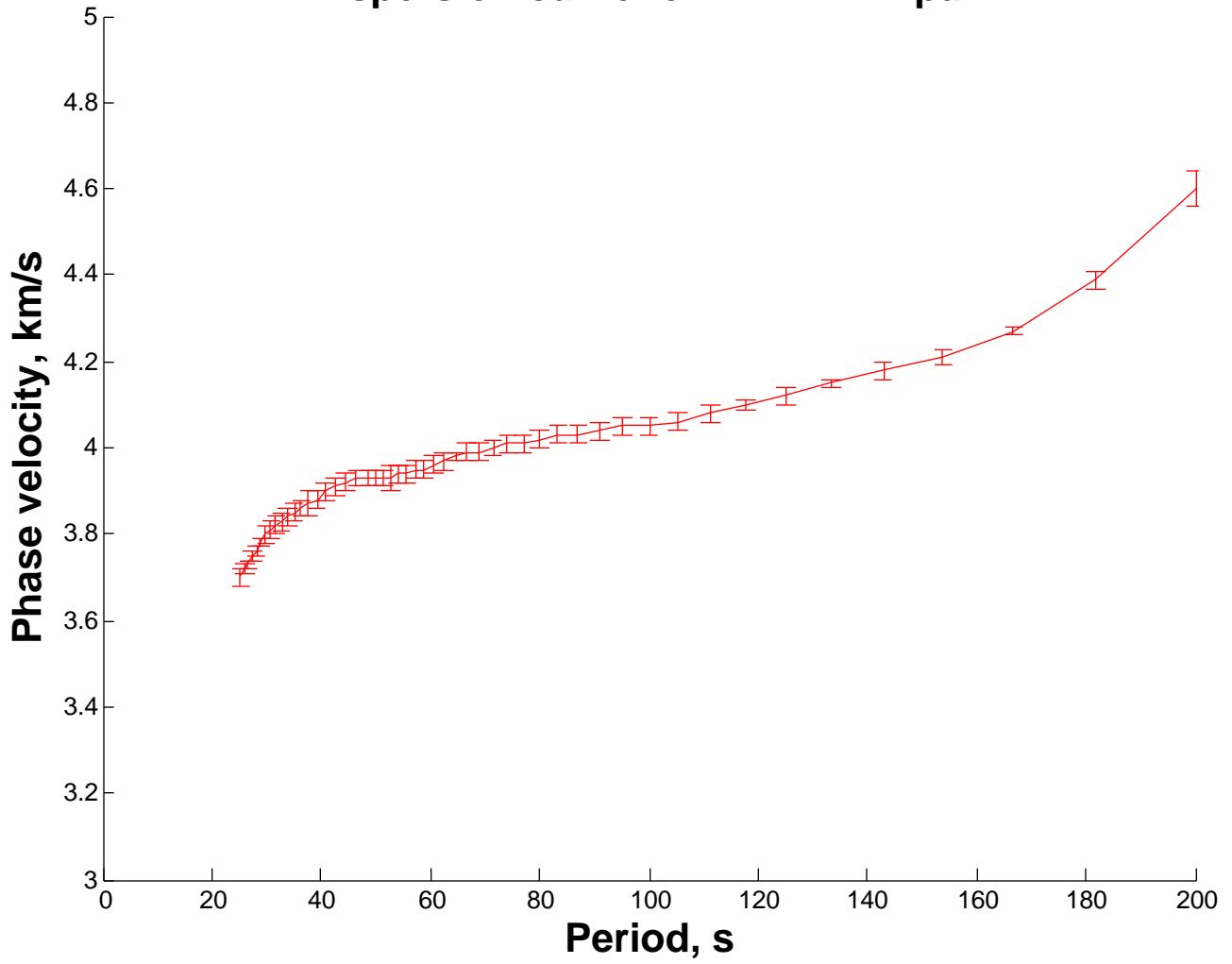
Dispersion curve for DIB EDM pair
