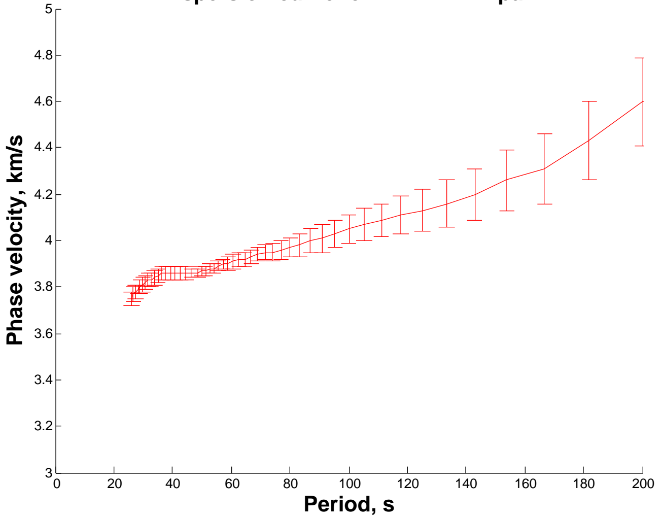
Dispersion curve for DAWY DIB pair
