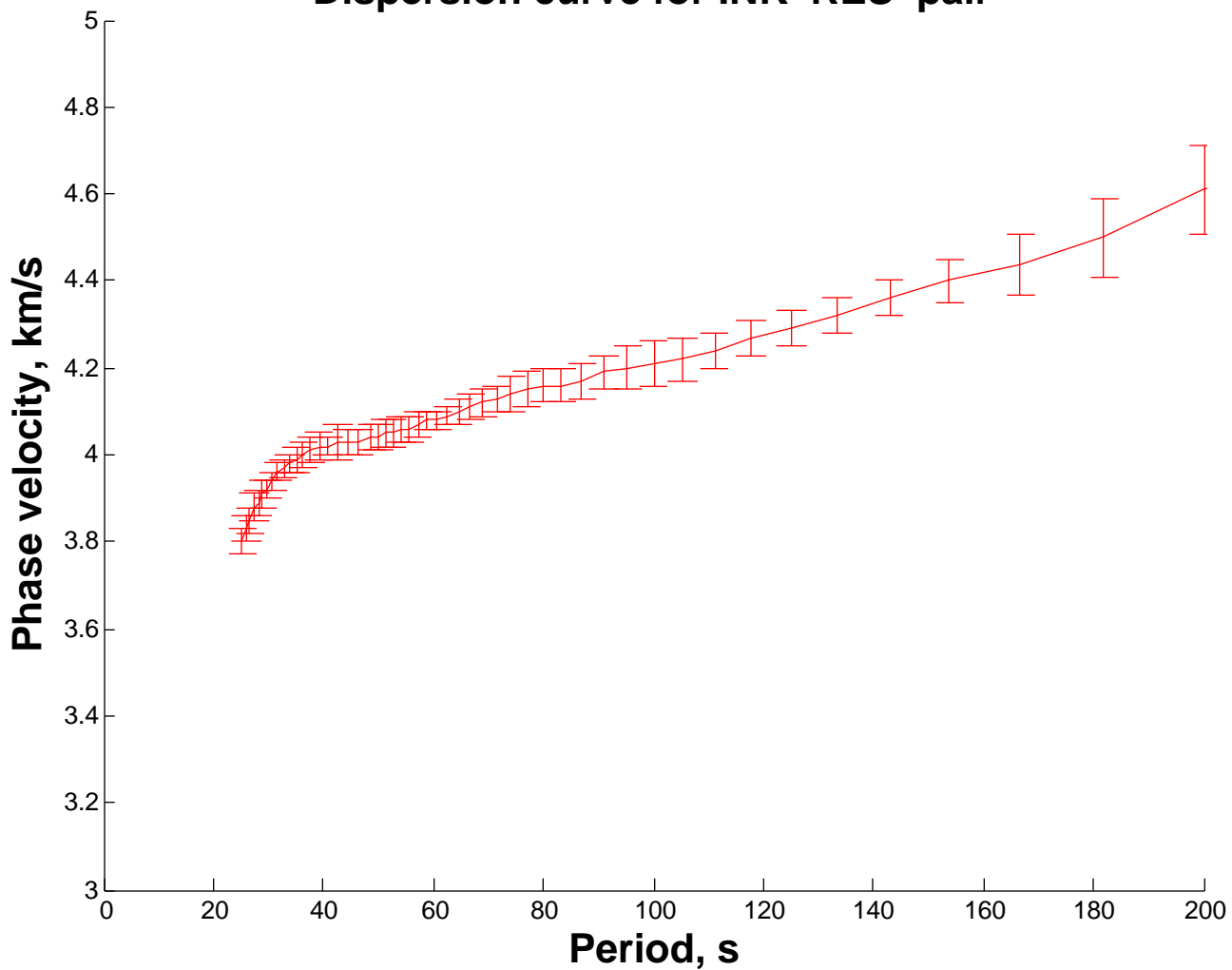
Dispersion curve for INK RES pair
