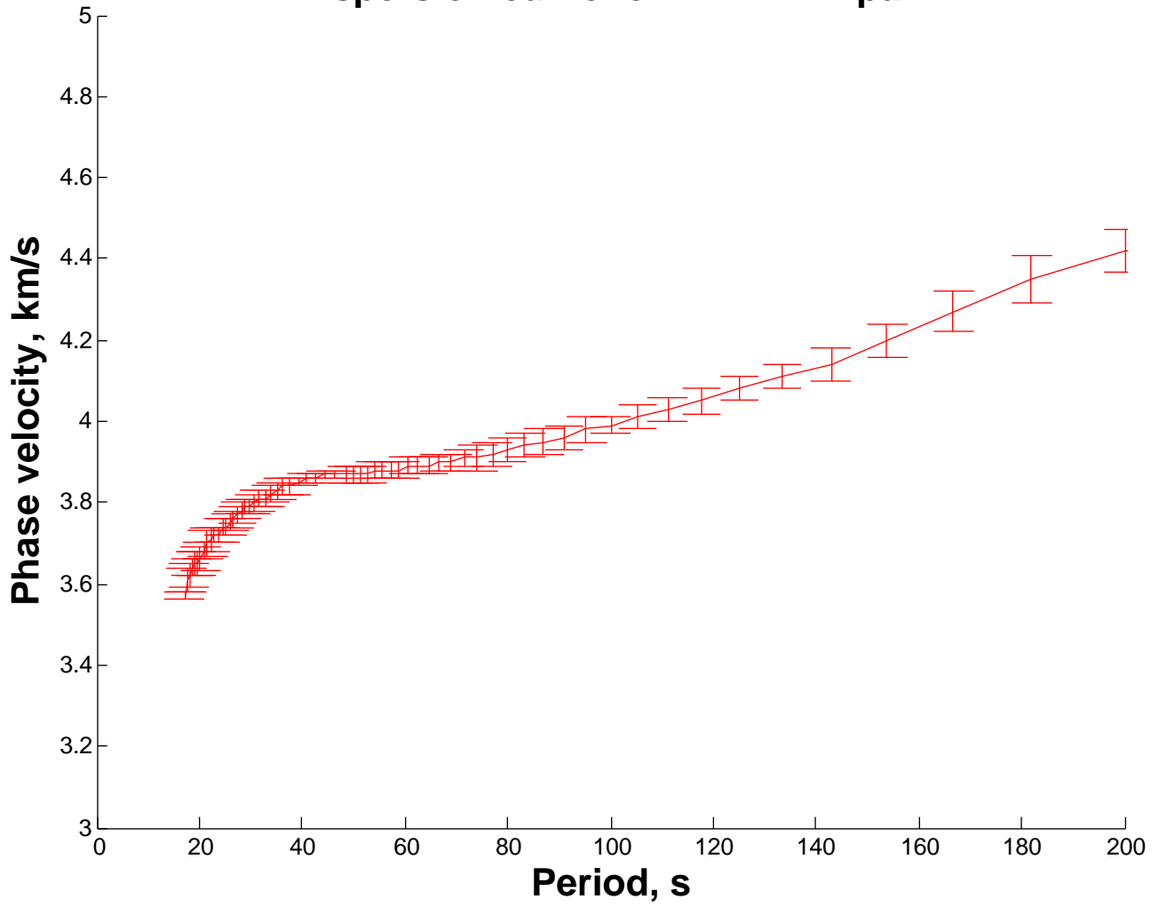
Dispersion curve for DIB PNT pair
