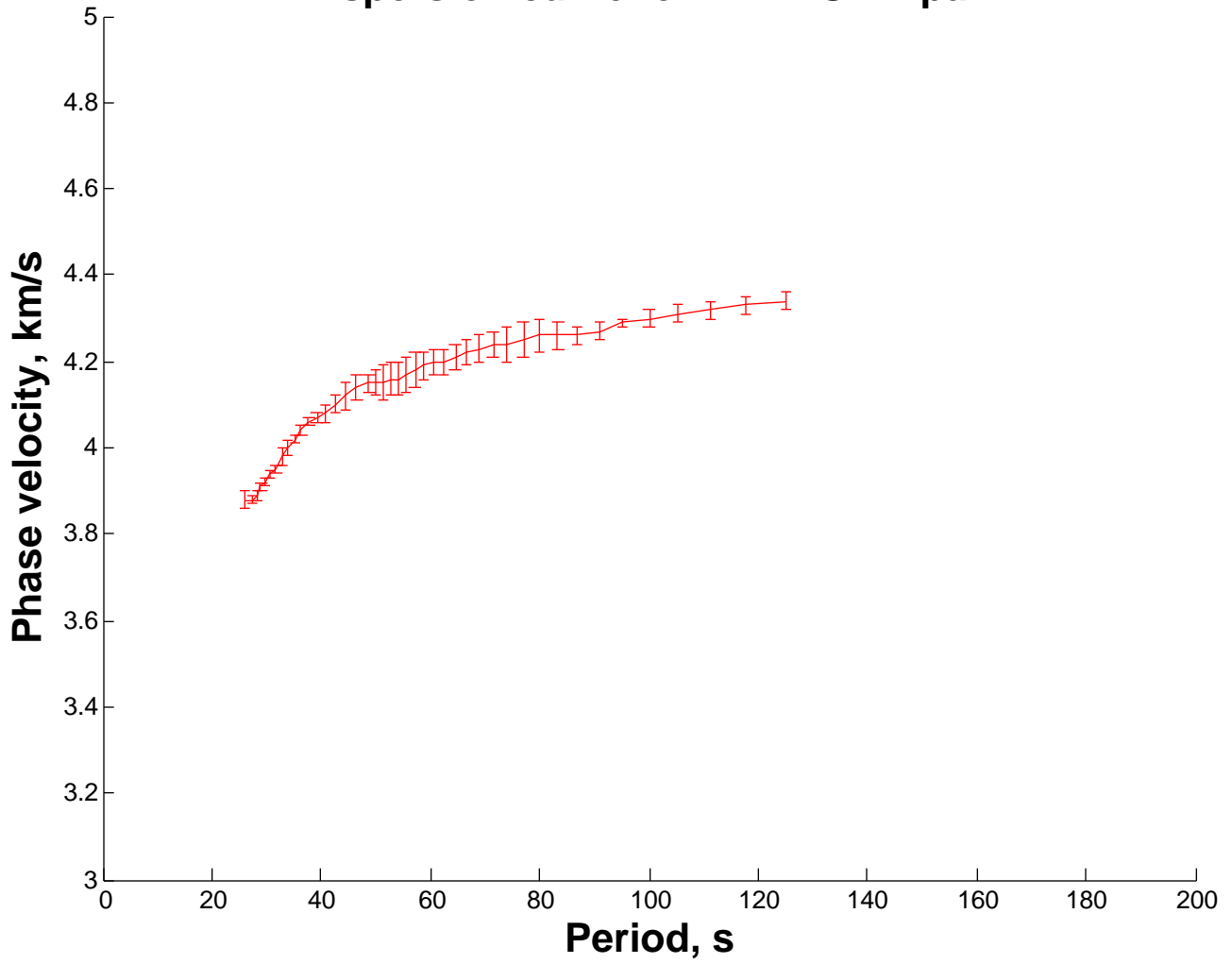
Dispersion curve for INK FSMA pair
