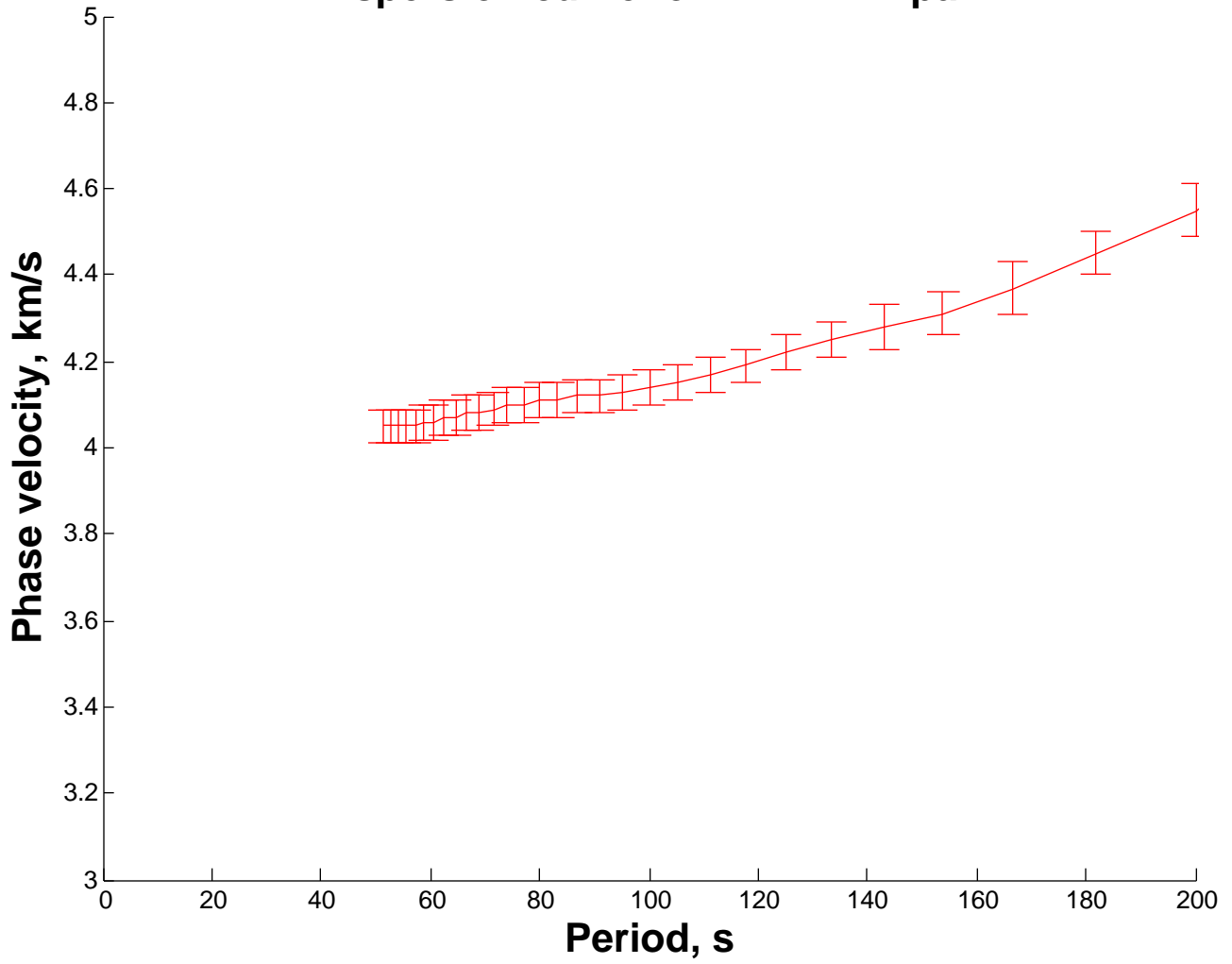
Dispersion curve for INK PNT pair
