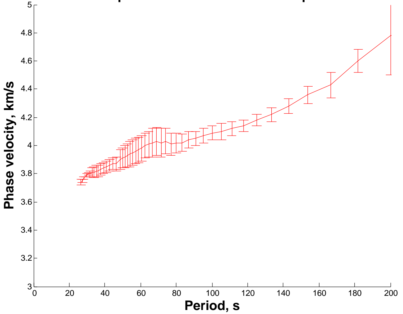
Dispersion curve for PNT PLBC pair
