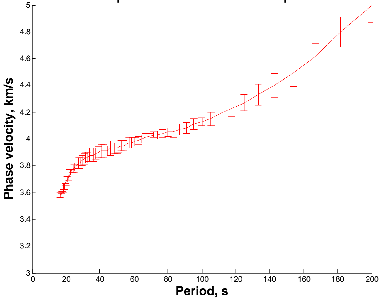
Dispersion curve for DIB VGZ pair
