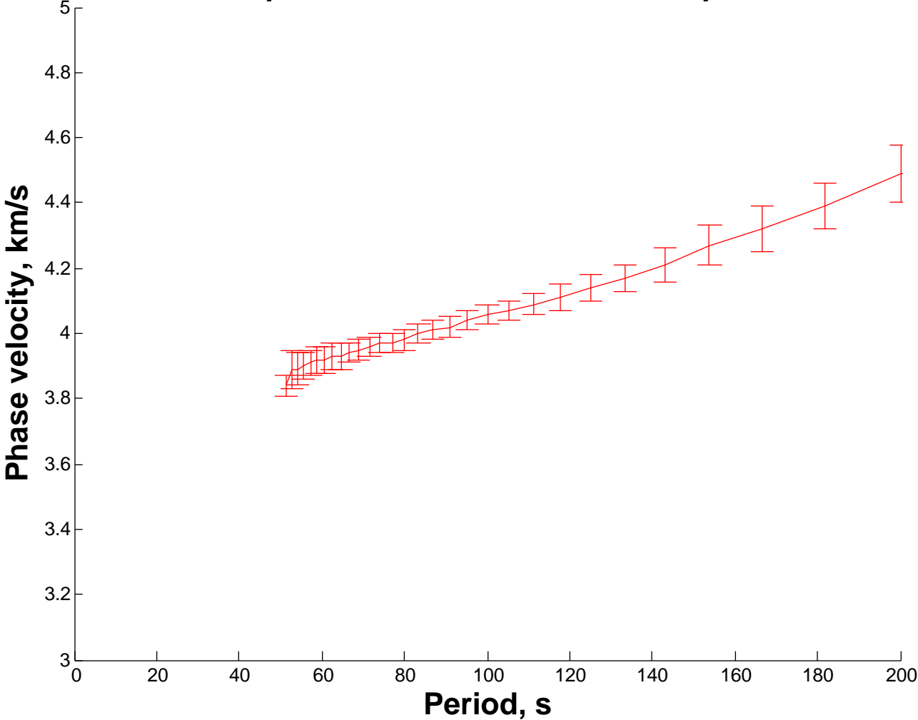
Dispersion curve for PNT DAWY pair
