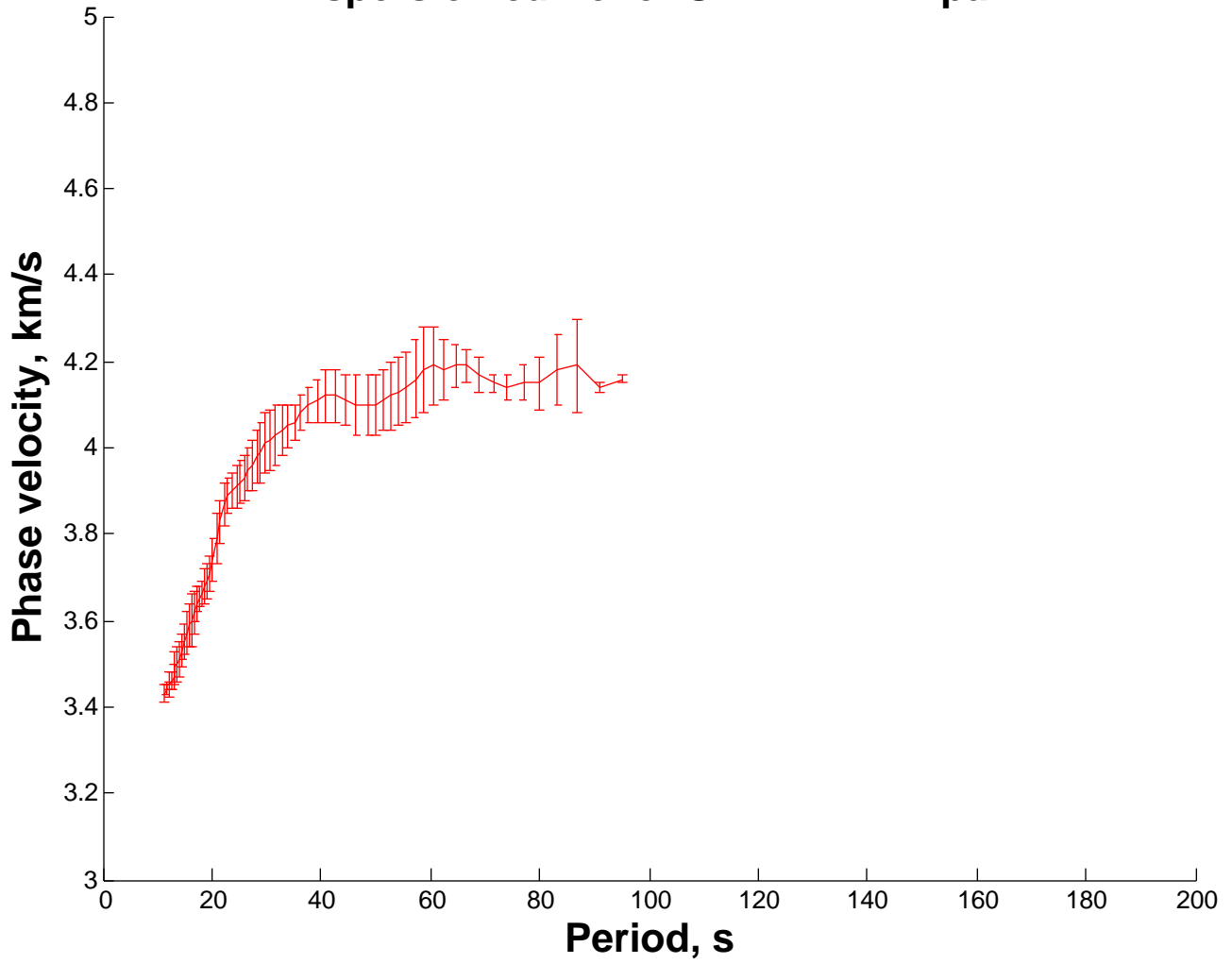
Dispersion curve for SMPN DHRN pair
