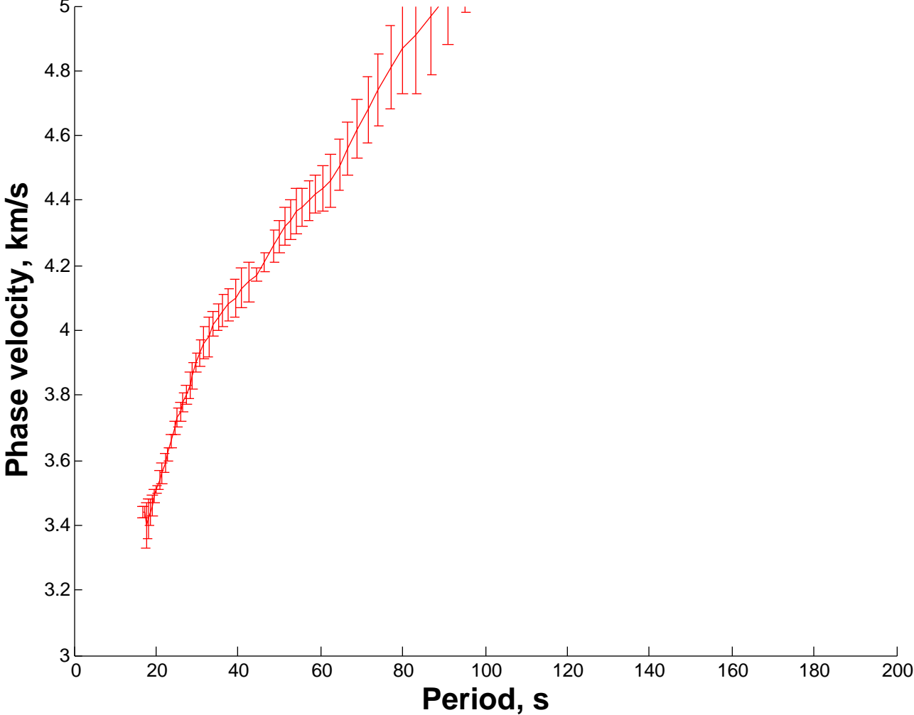
Dispersion curve for VGZ PNT pair
