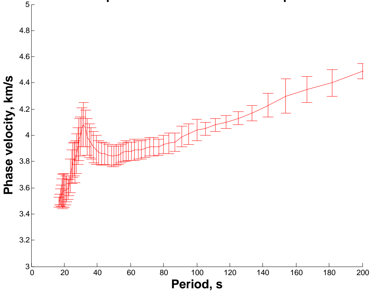
Dispersion curve for PLBC DLBC pair
