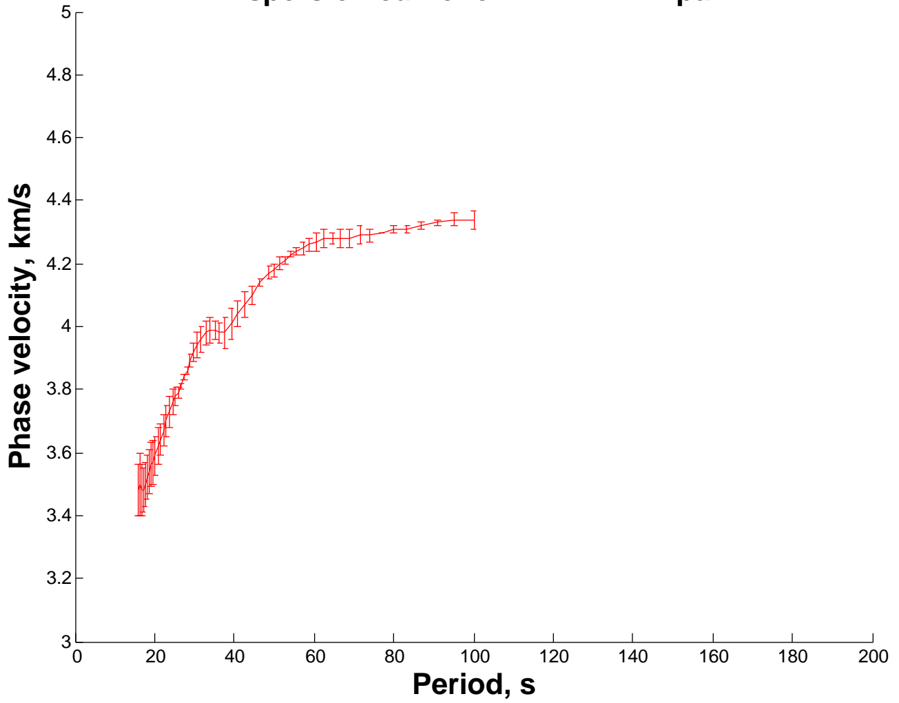
Dispersion curve for DAWY INK pair
