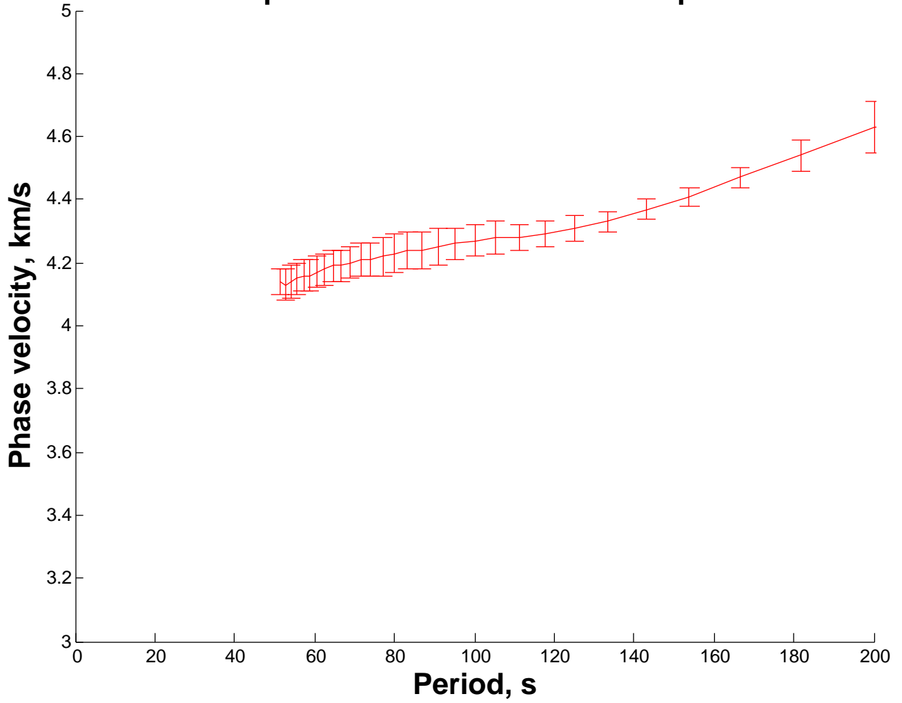
Dispersion curve for MBC EDM pair
