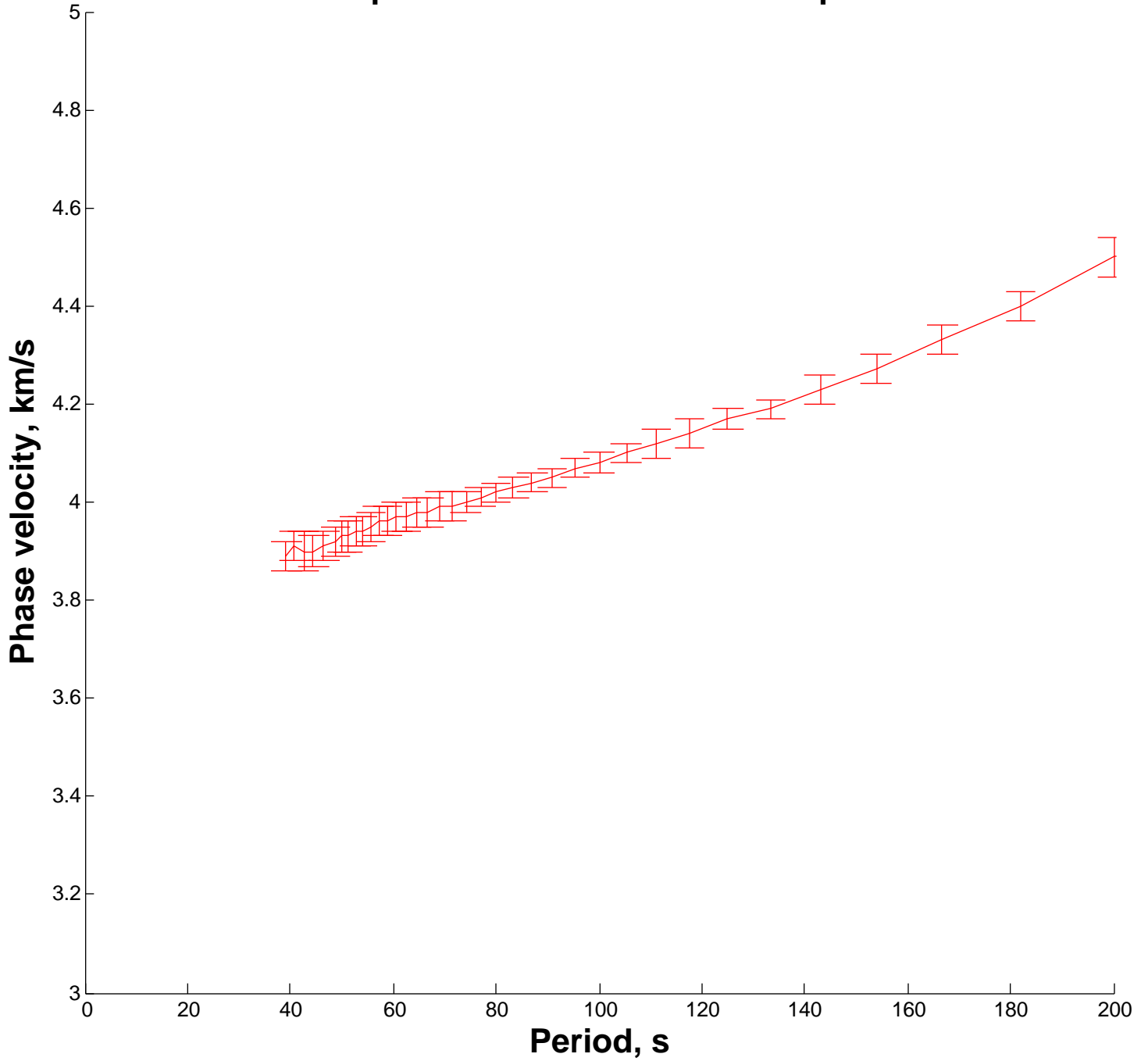
Dispersion curve for BBB INK pair
