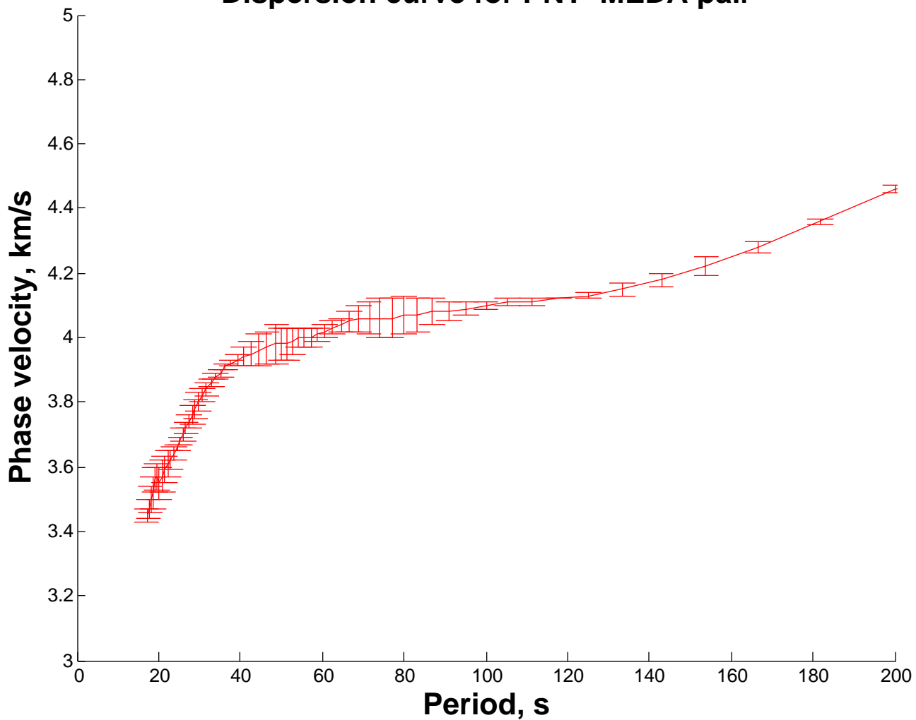
Dispersion curve for PNT MEDA pair
