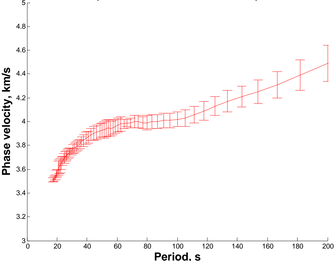
Dispersion curve for BMBC PNT pair
