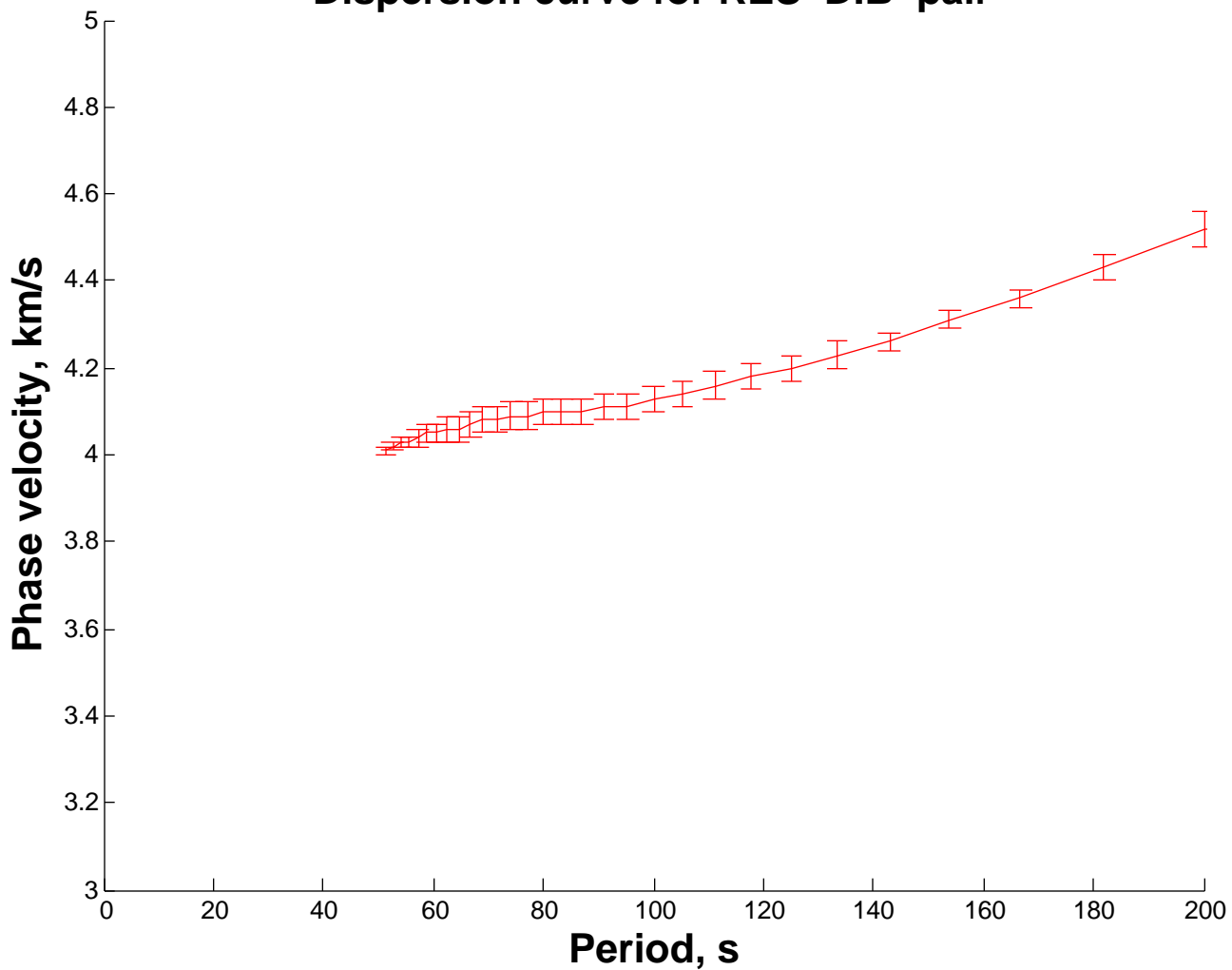
Dispersion curve for RES DIB pair
