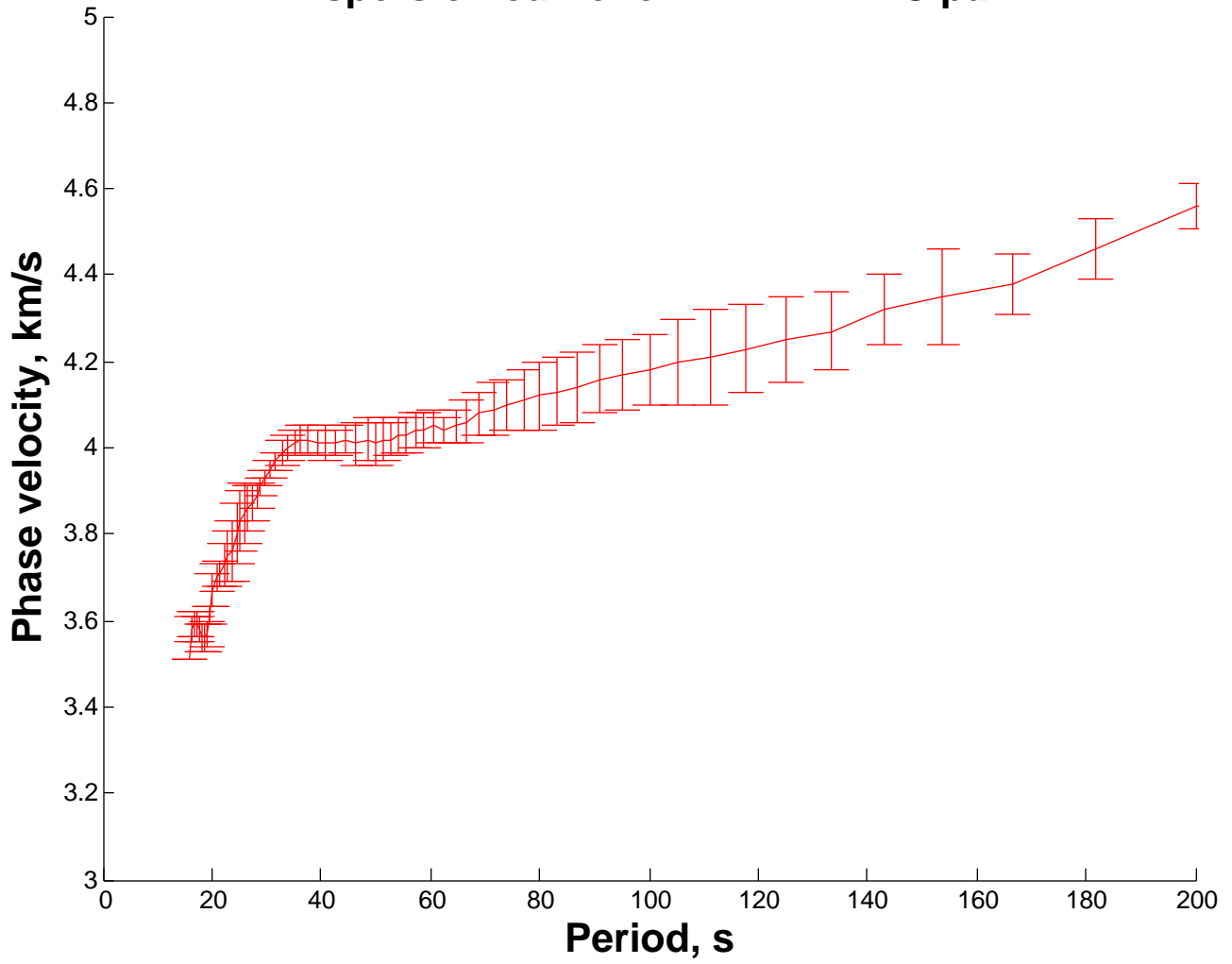
Dispersion curve for FNBB BMBC pair
