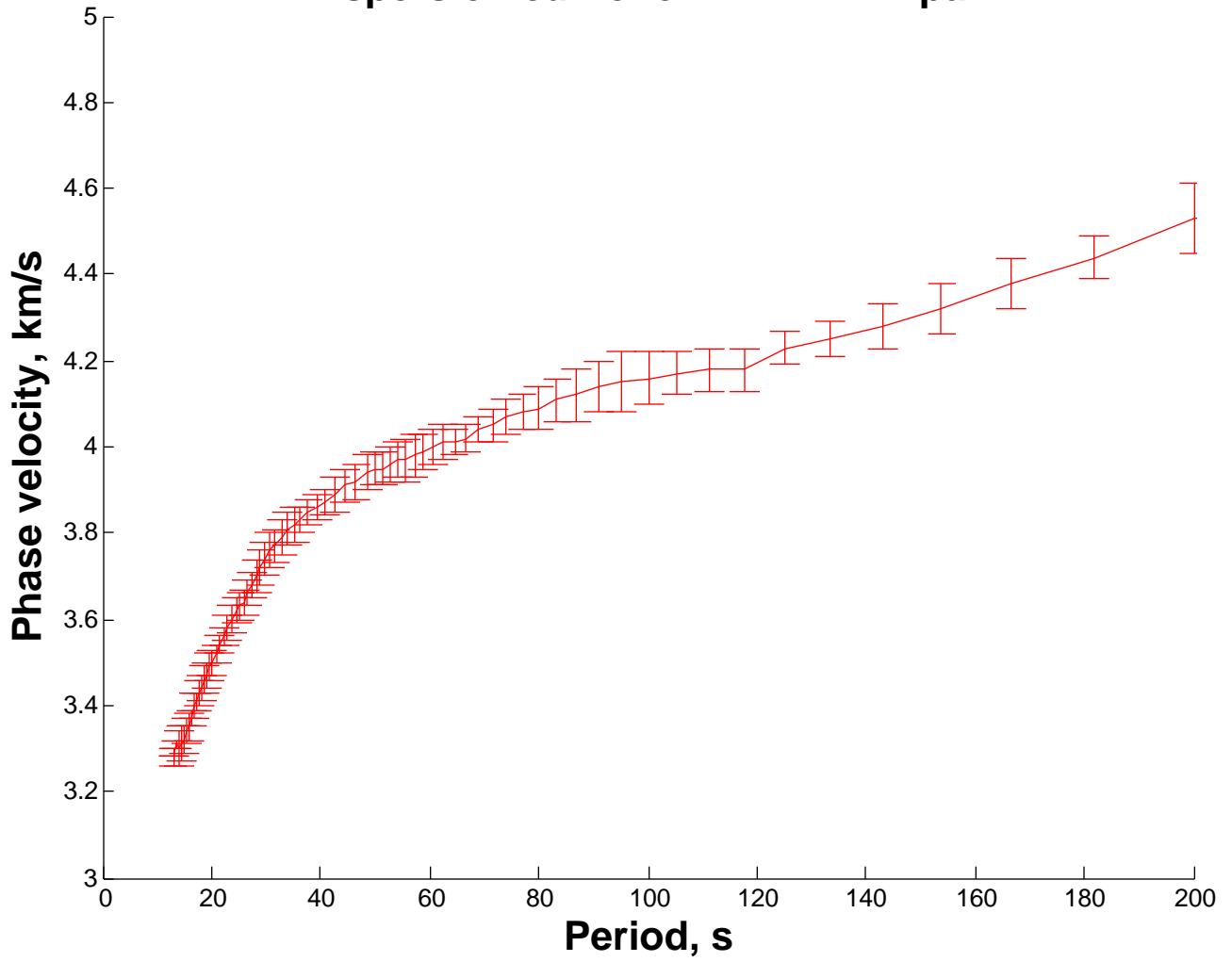
Dispersion curve for PNT EDM pair
