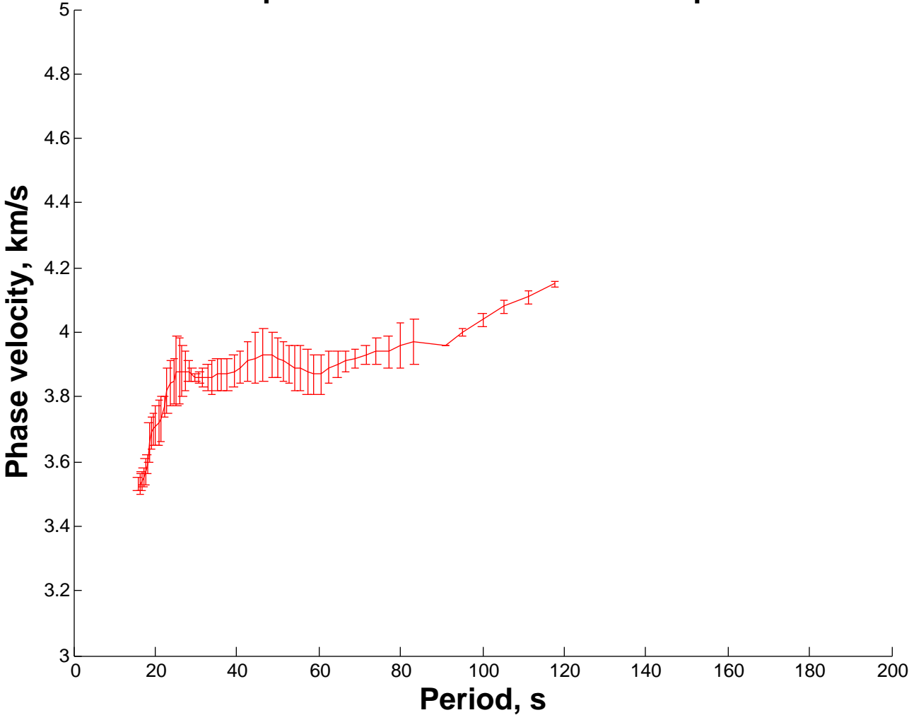
Dispersion curve for RUBB PHC pair
