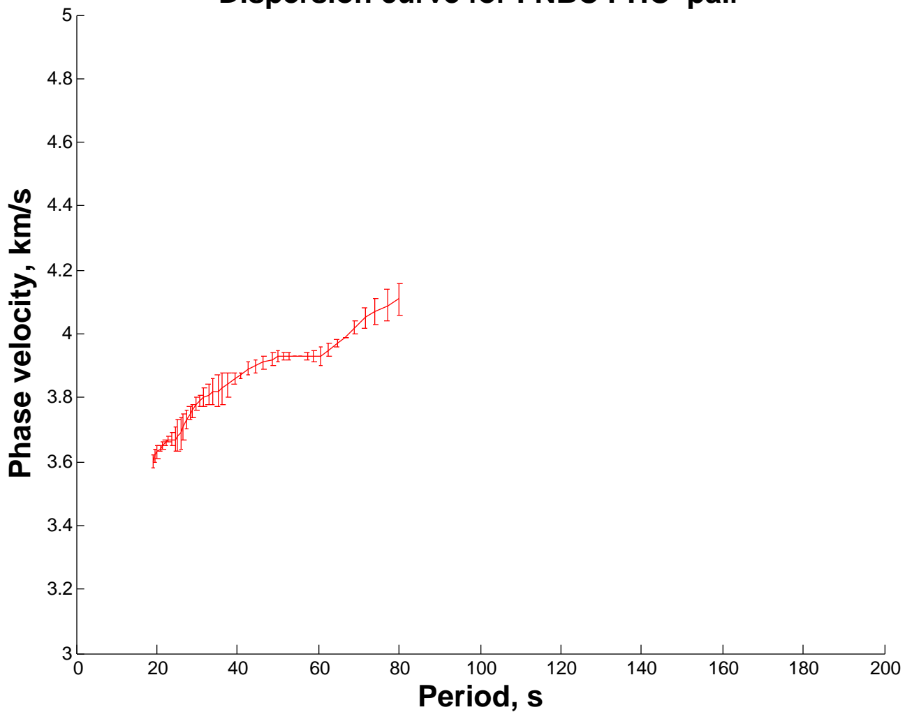
Dispersion curve for FNBC PHC pair
