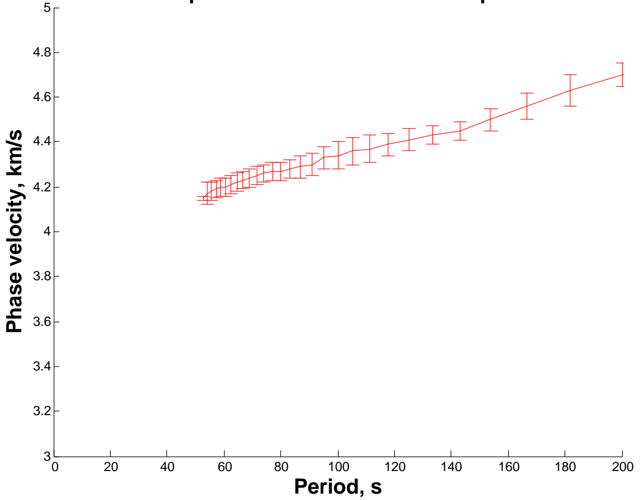
Dispersion curve for MBC FCC pair
