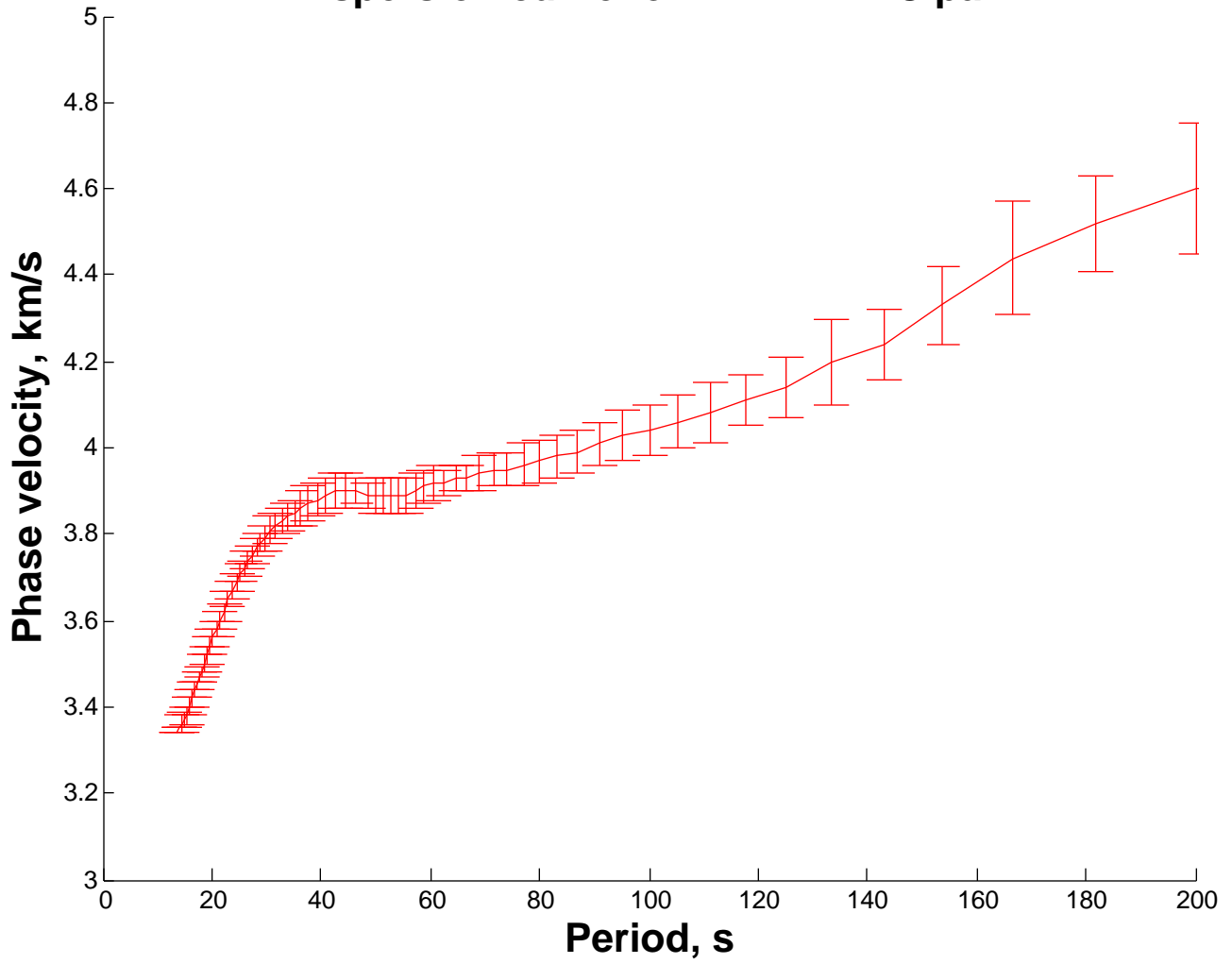
Dispersion curve for BBB BMBC pair
