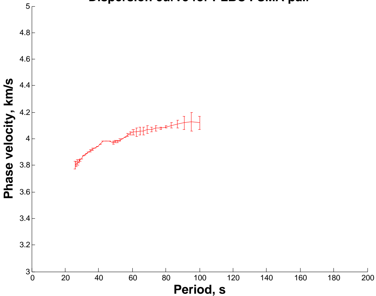
Dispersion curve for PLBC FSMA pair
