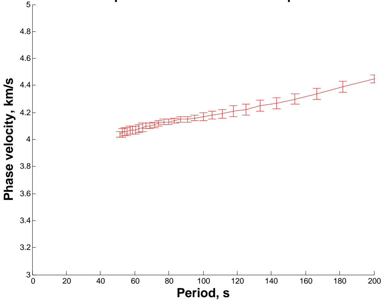
Dispersion curve for RES PHC pair
