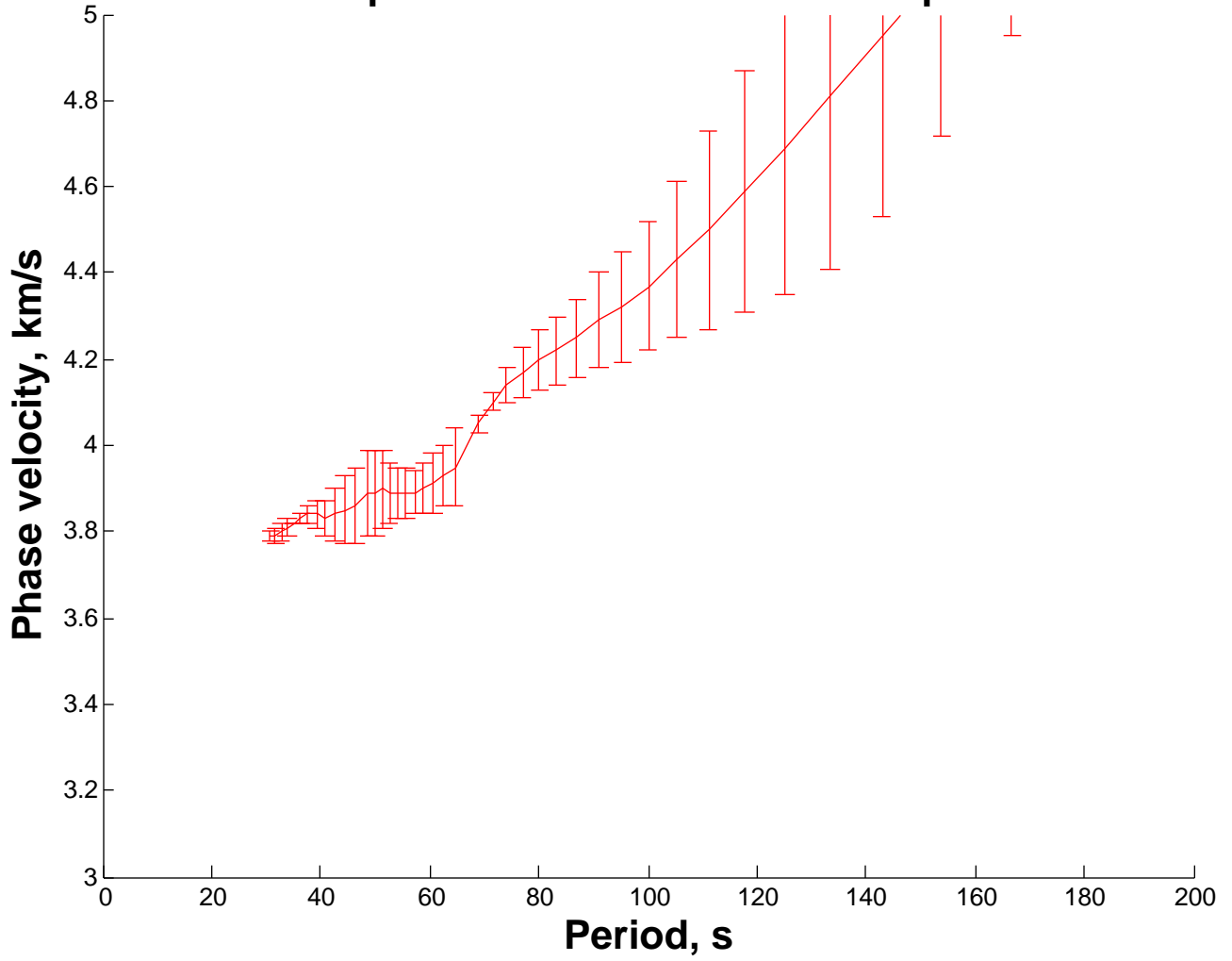
Dispersion curve for BBB VGZ pair
