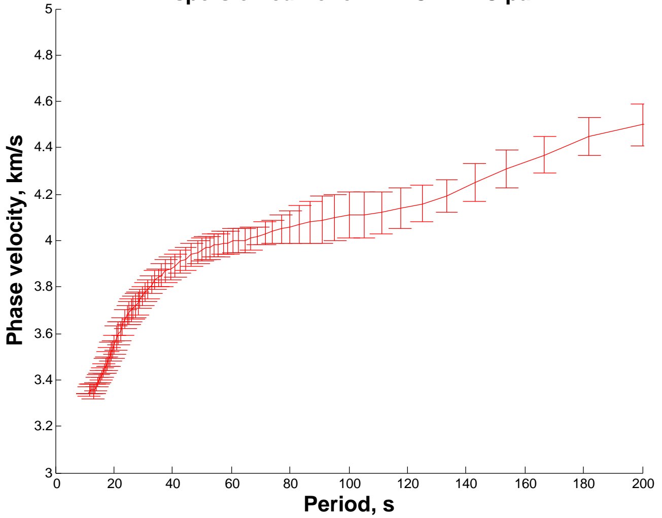
Dispersion curve for DLBC BMBC pair
