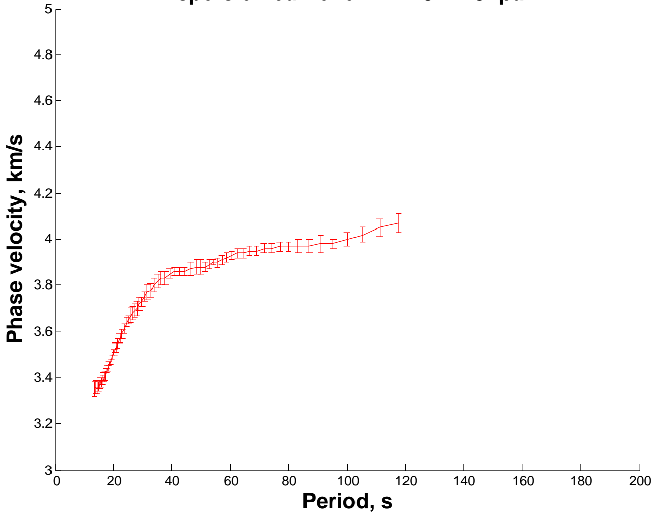
Dispersion curve for BMBC PHC pair
