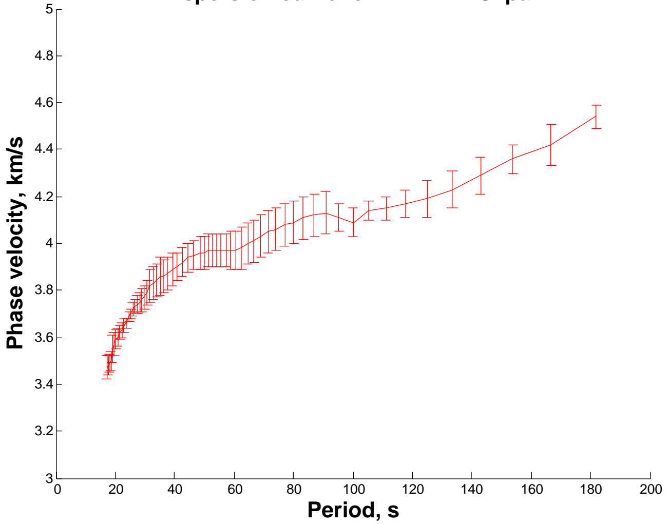
Dispersion curve for FNBB PHC pair
