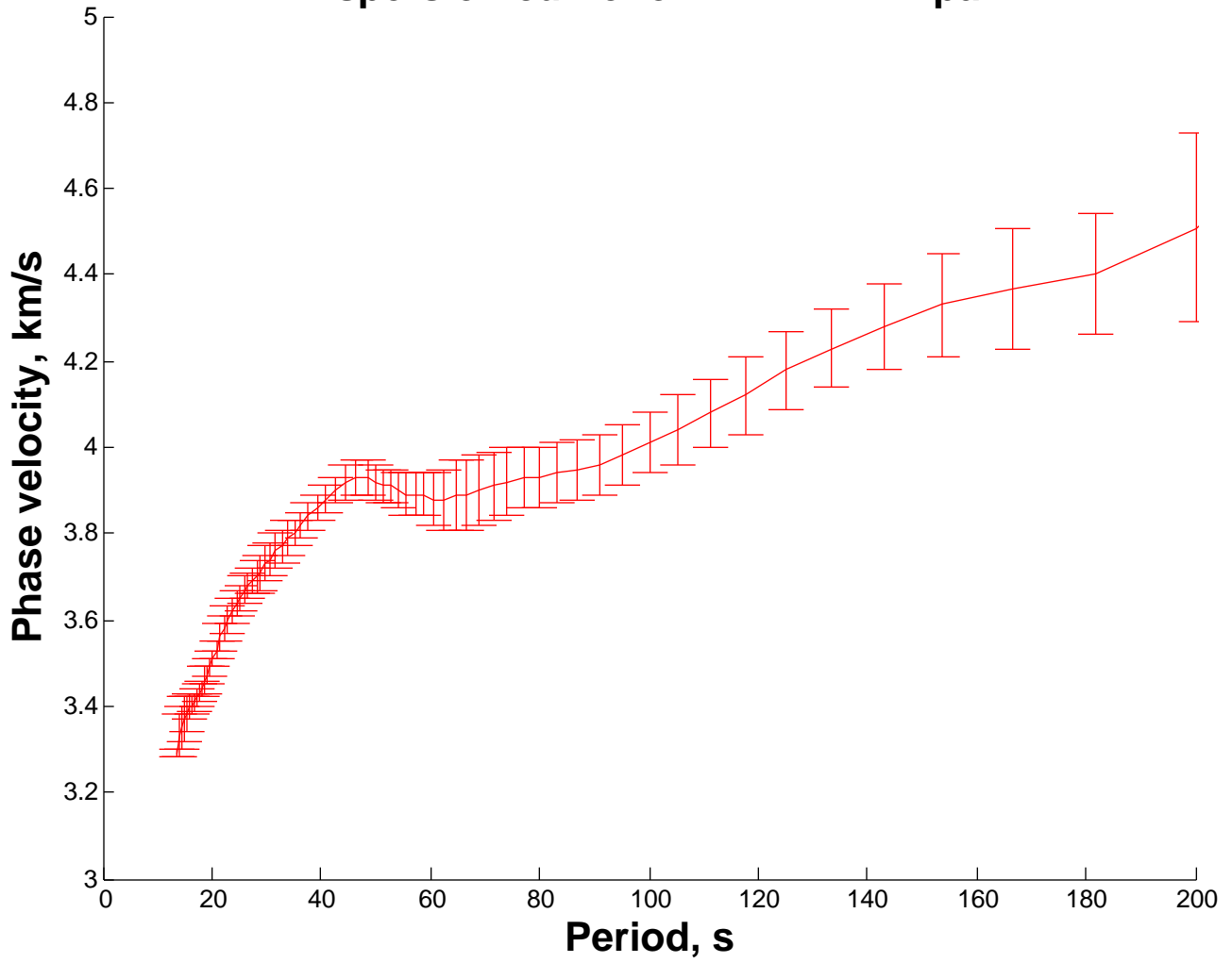
Dispersion curve for PNT WALA pair
