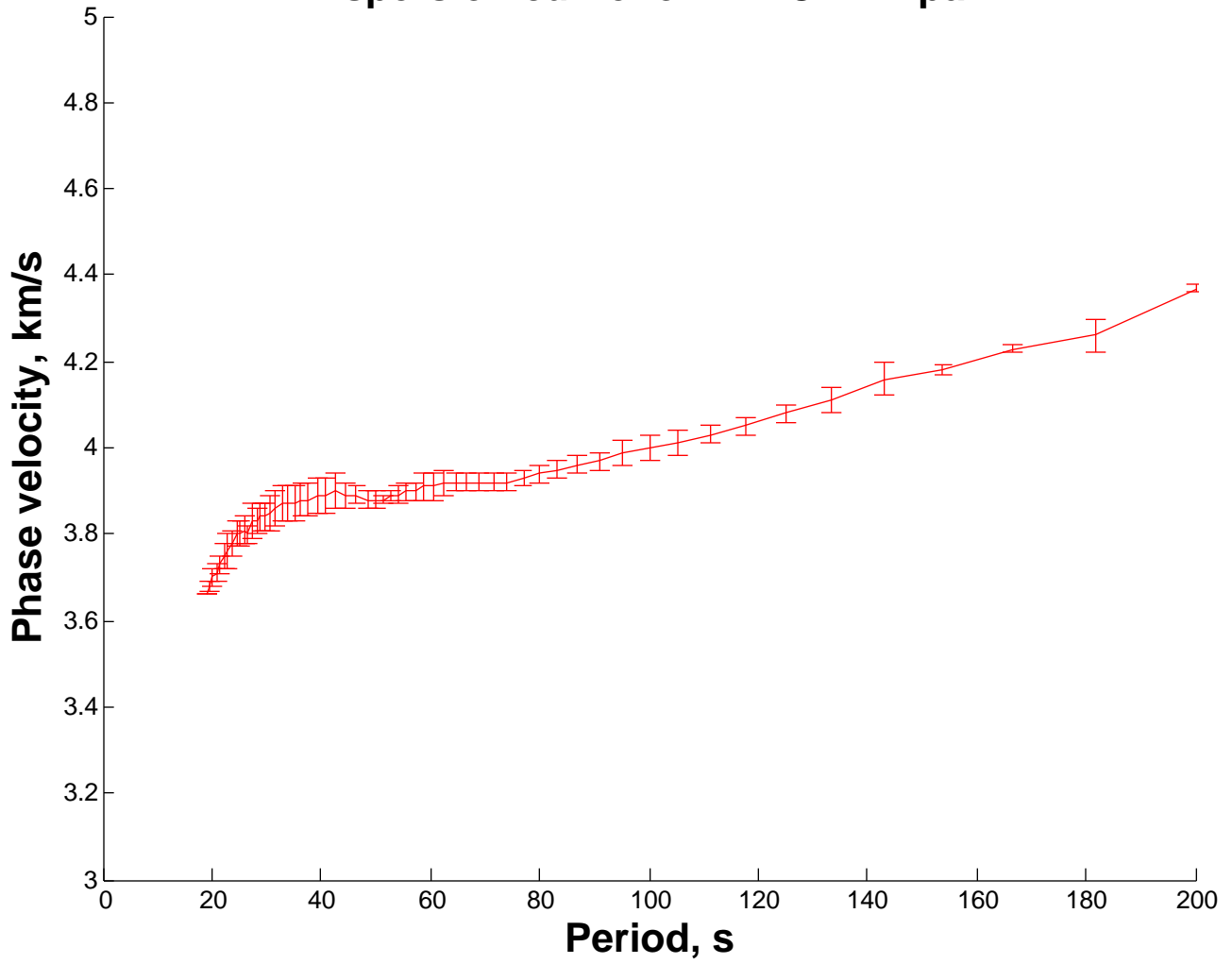
Dispersion curve for PLBC DIB pair
