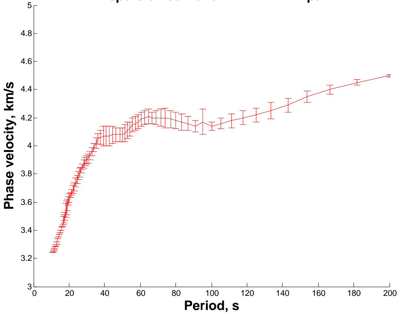
Dispersion curve for EDM WAPA pair
