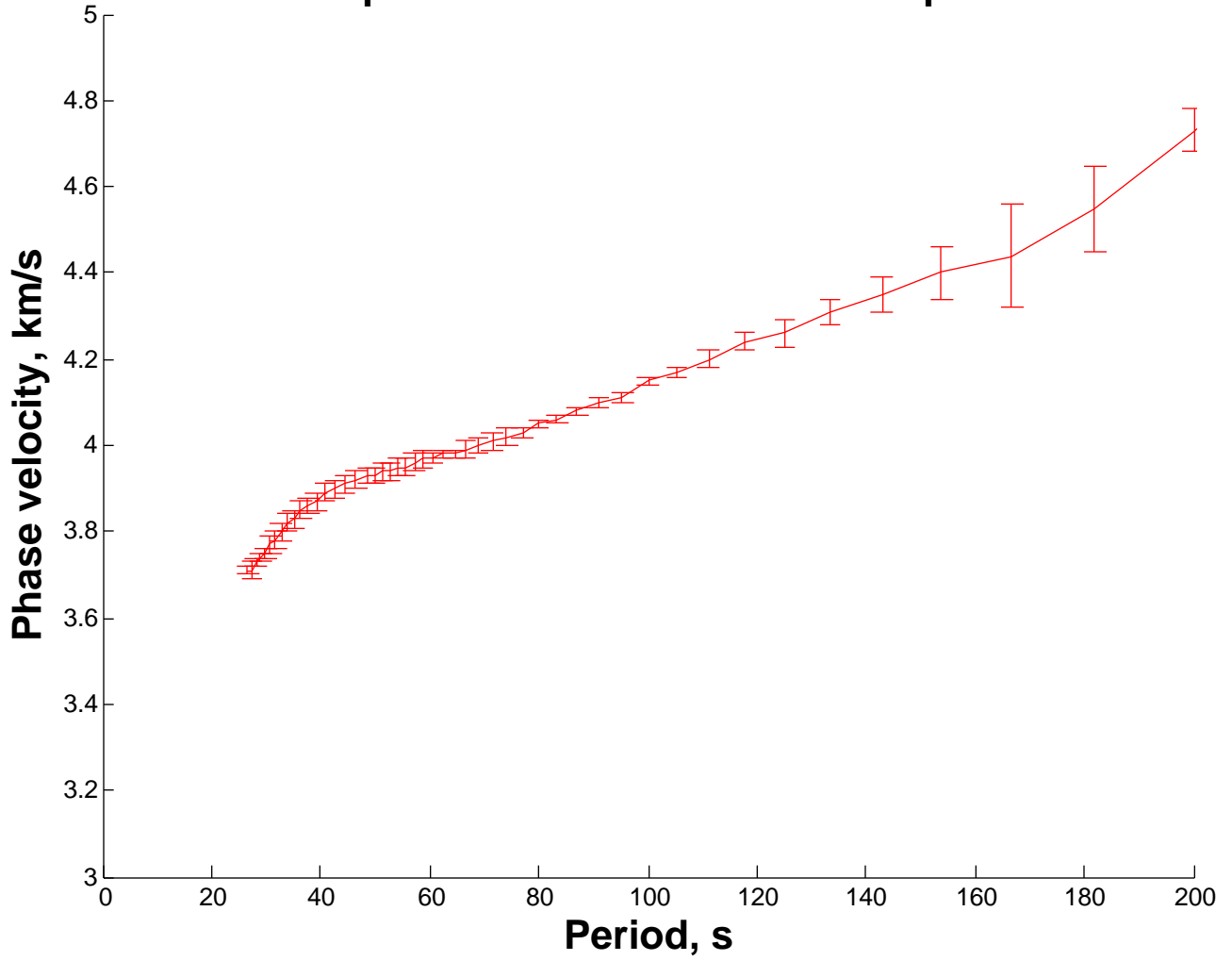
Dispersion curve for DIB MEDA pair
