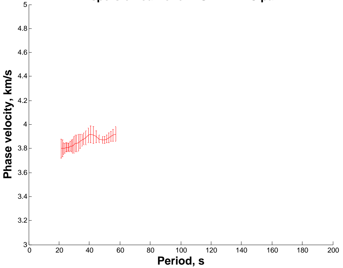
Dispersion curve for RUBB PLBC pair
