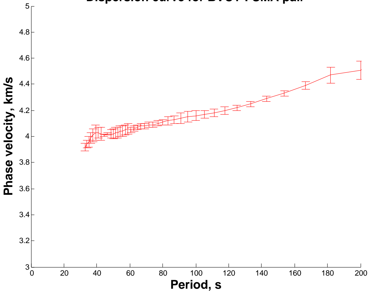
Dispersion curve for BVCY FSMA pair
