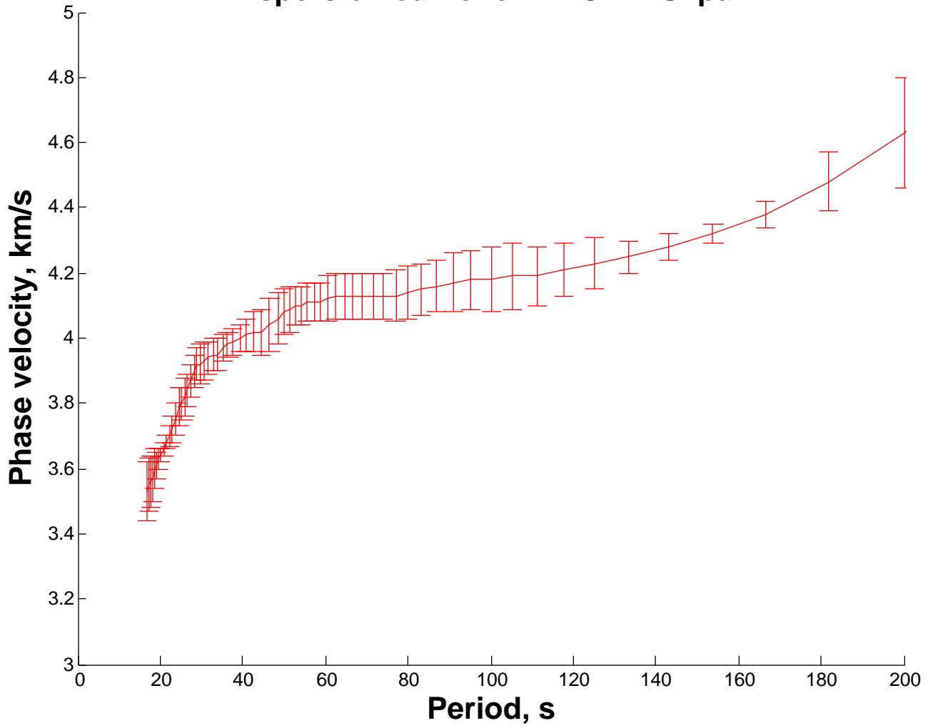
Dispersion curve for MBC RES pair
