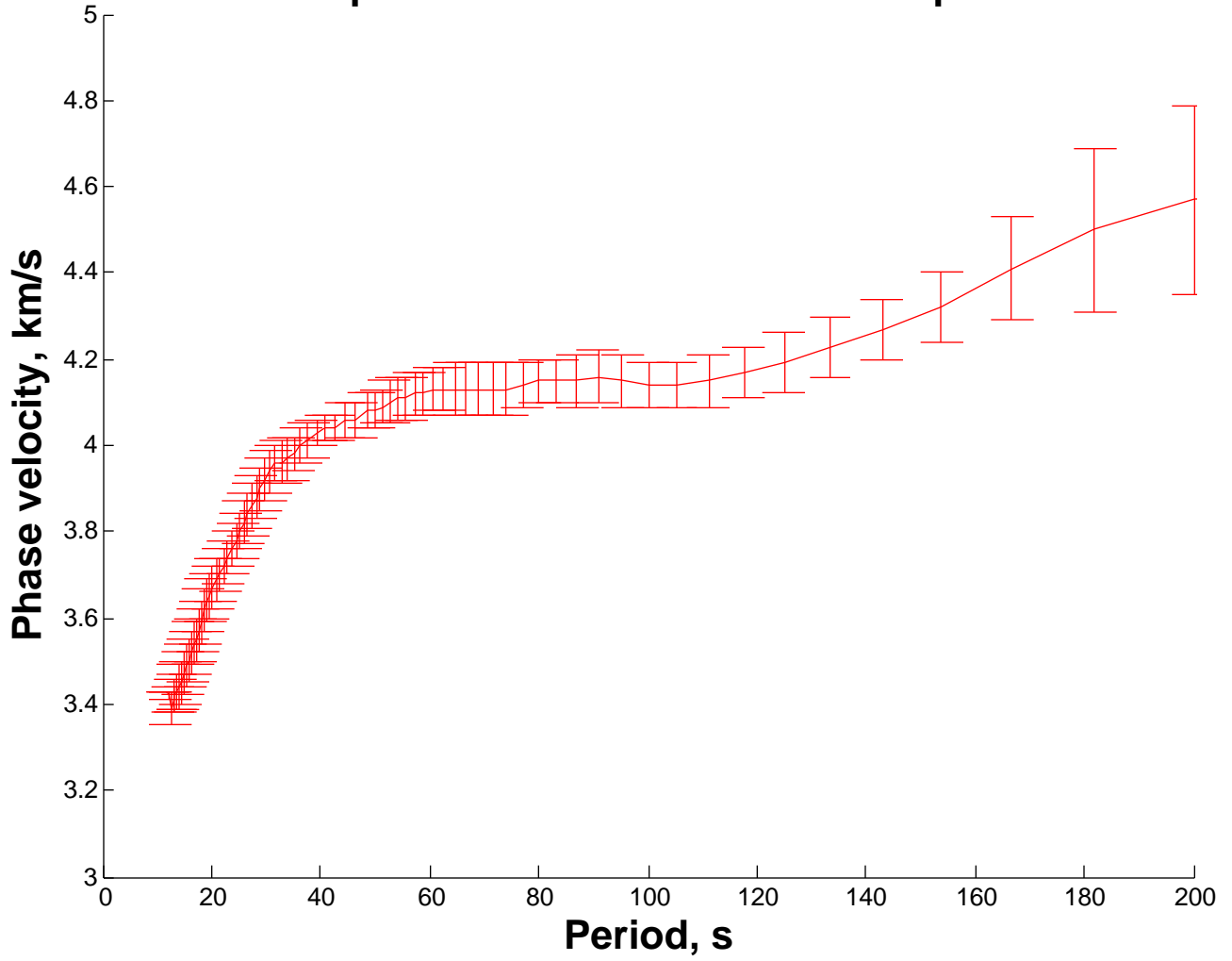
Dispersion curve for BMBC EDM pair
