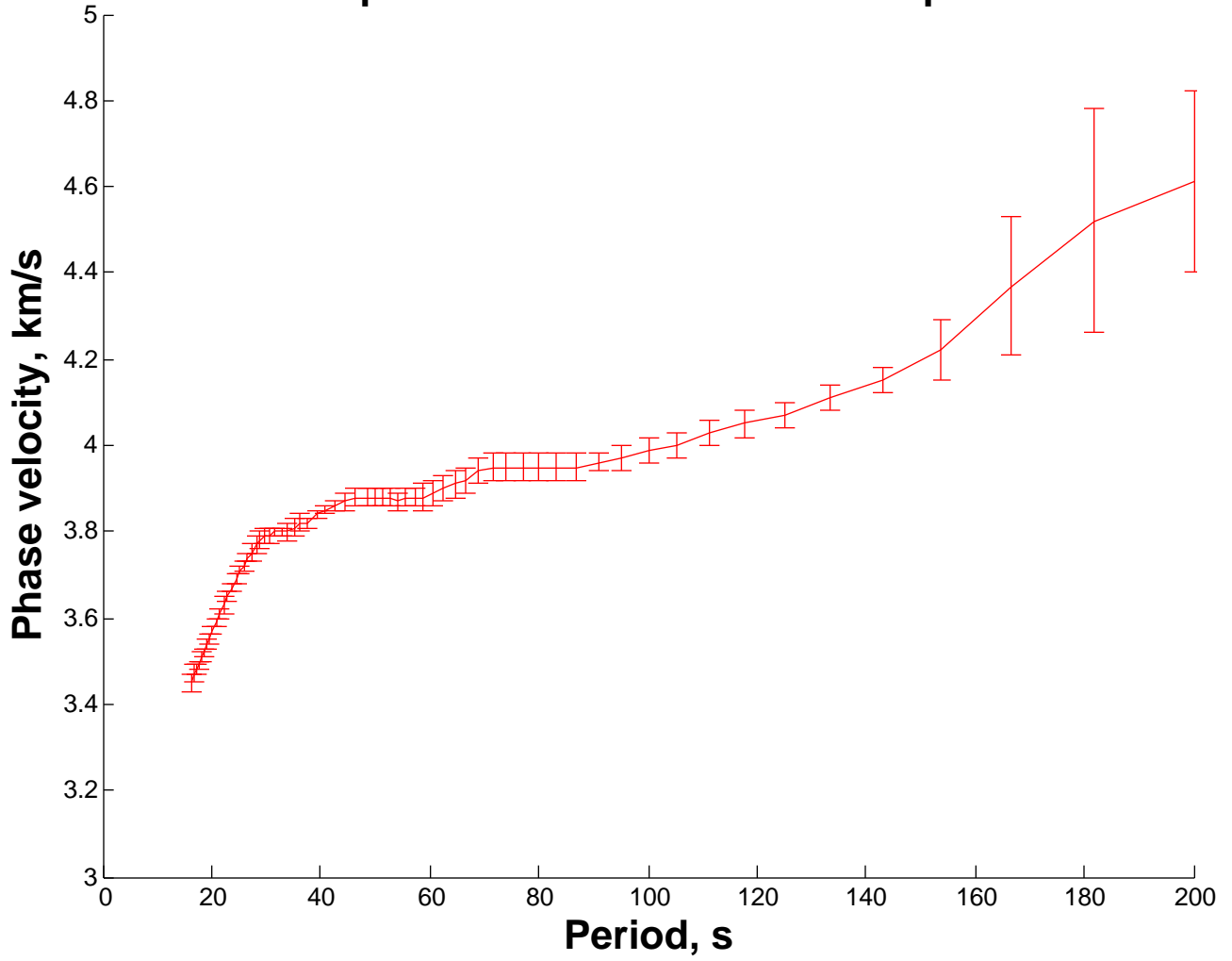
Dispersion curve for DIB BMBC pair
