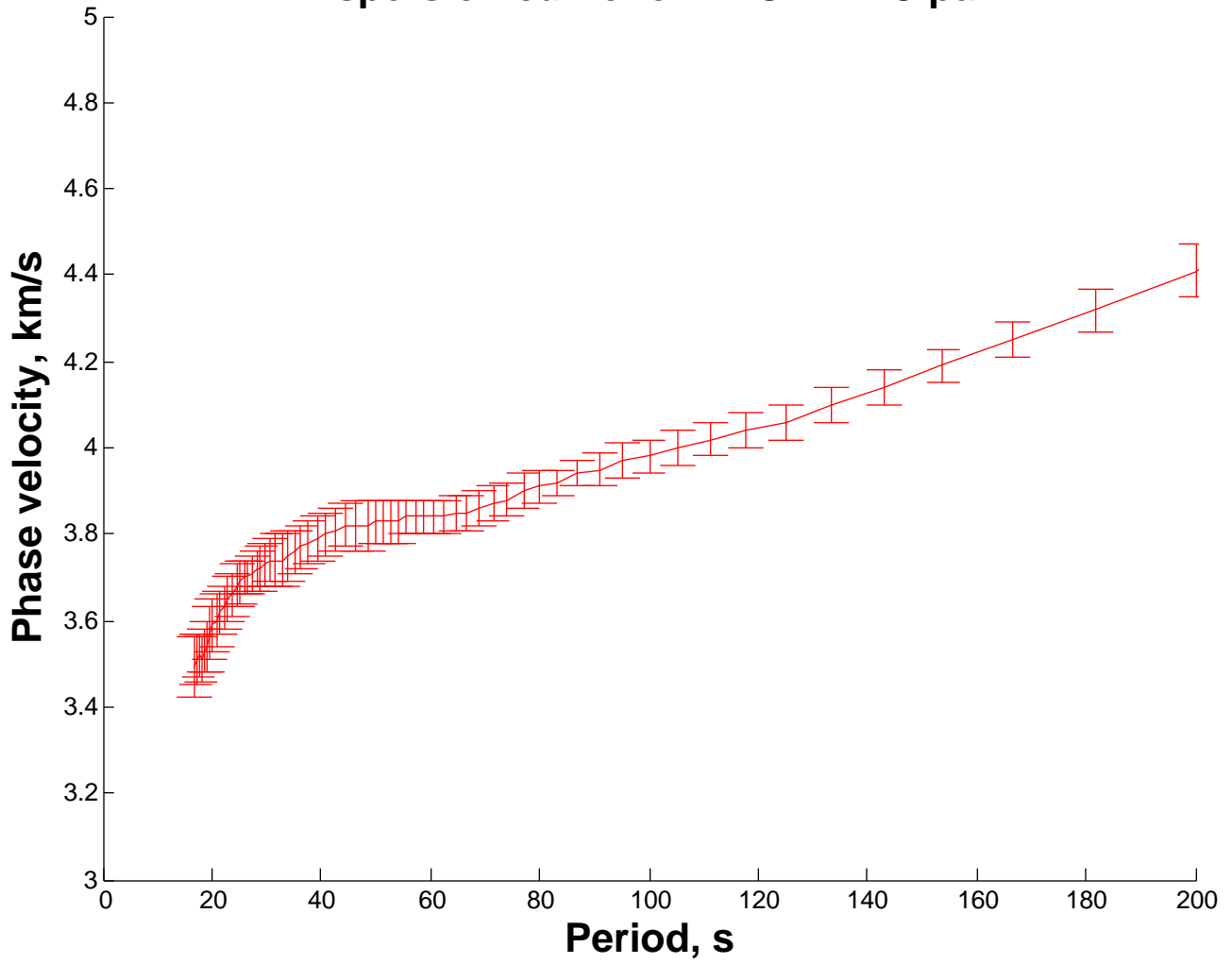
Dispersion curve for PHC DLBC pair
