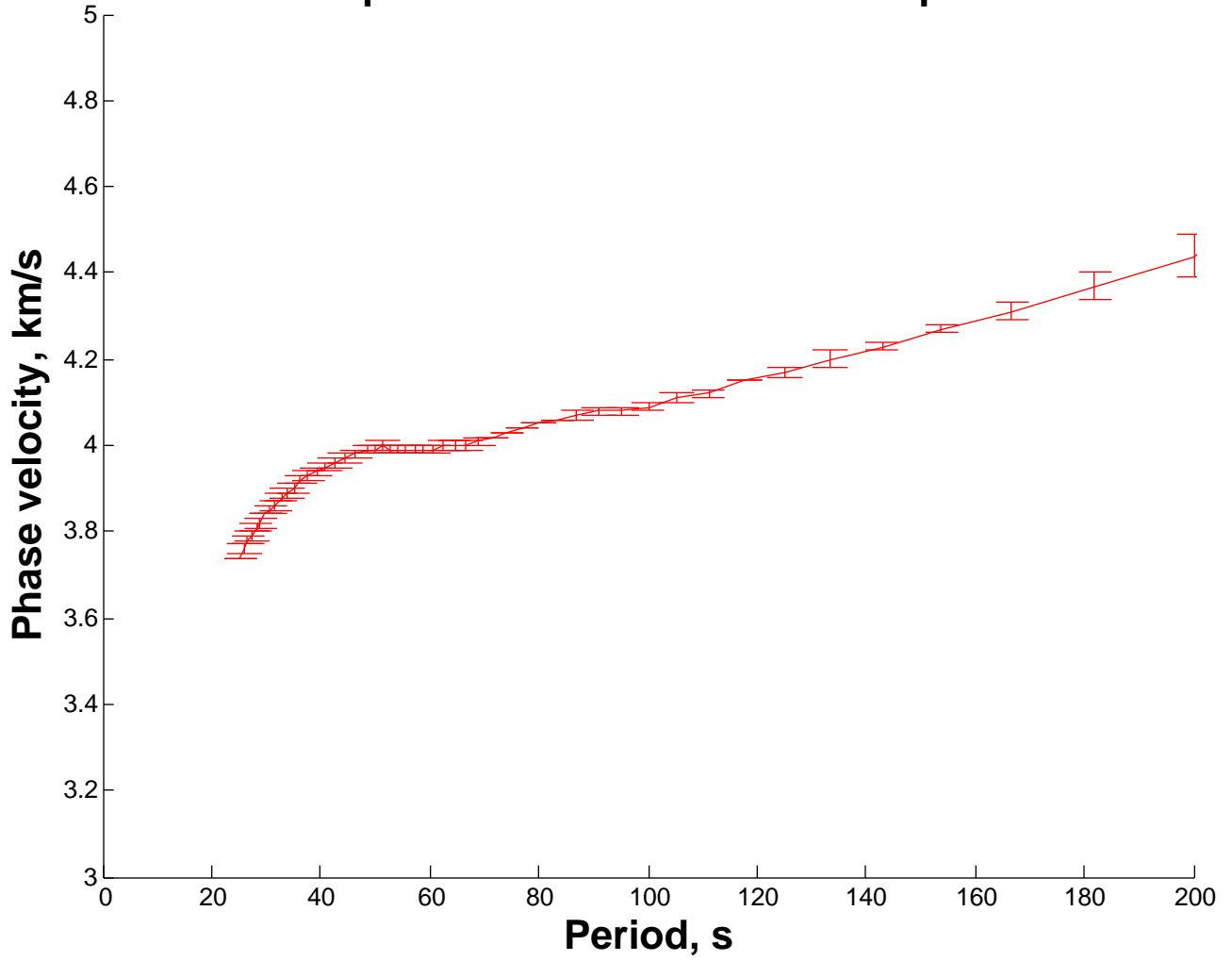
Dispersion curve for DIB FSMA pair
