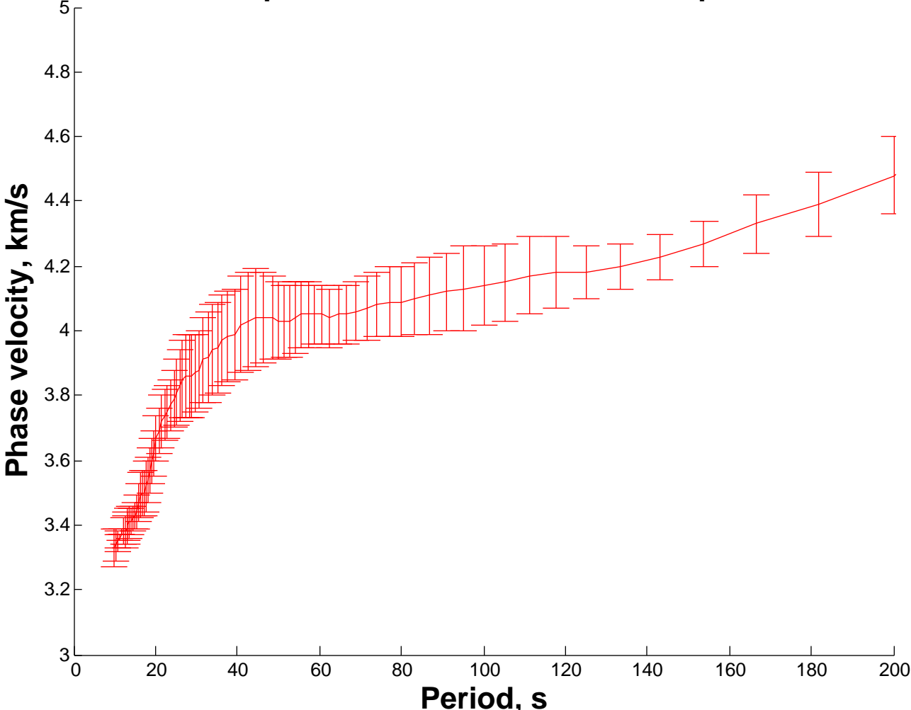
Dispersion curve for WHY DLBC pair
