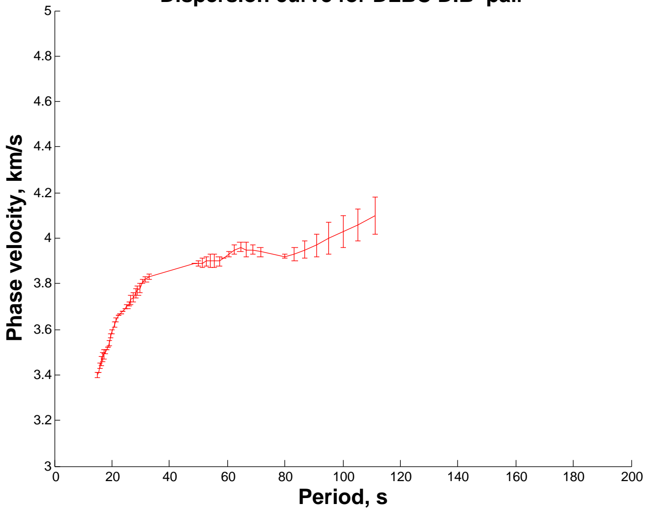
Dispersion curve for DLBC DIB pair
