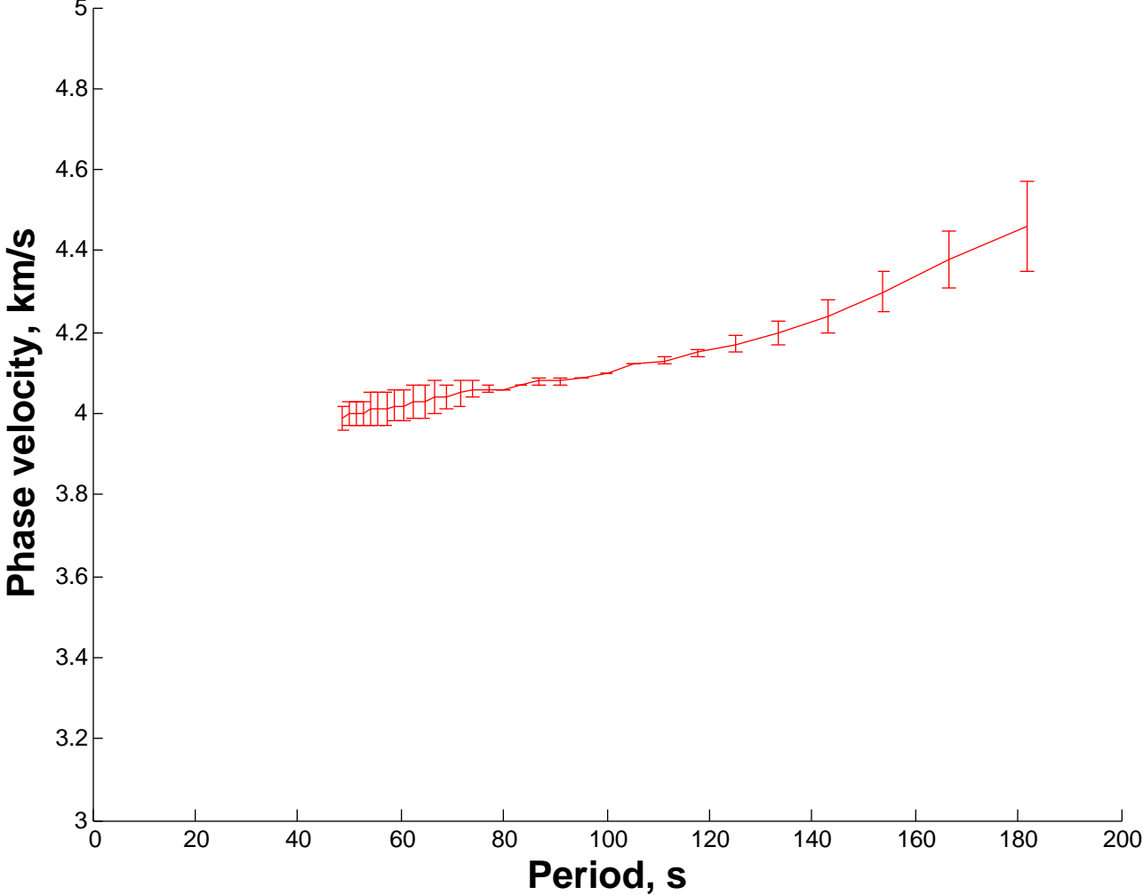
Dispersion curve for DHRN PHC pair
