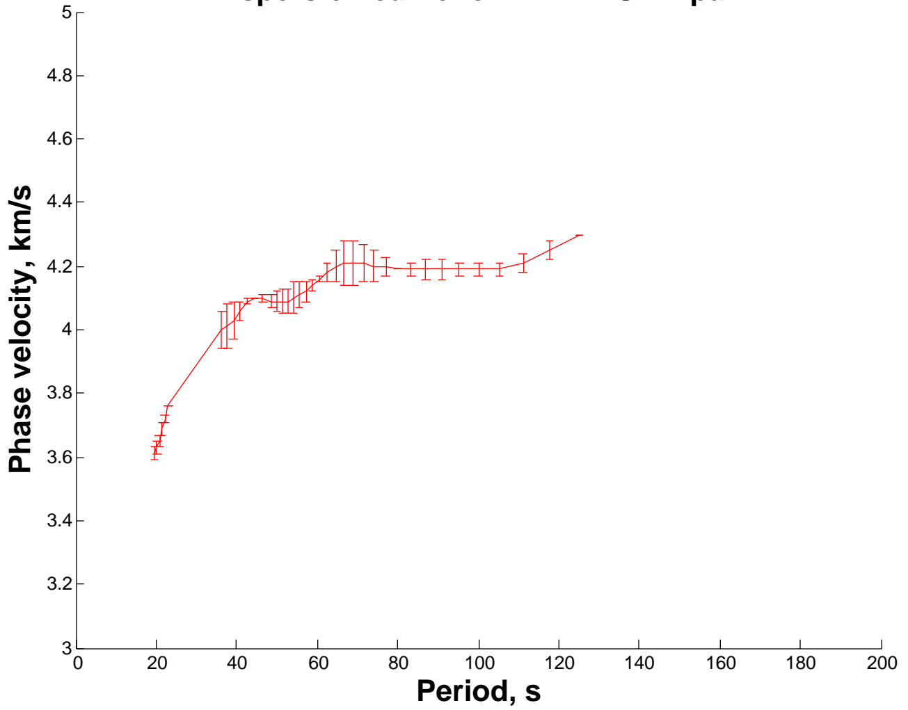
Dispersion curve for FNBB FSMA pair
