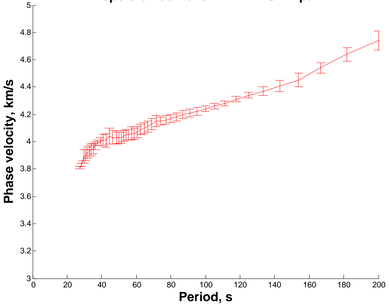
Dispersion curve for DAWY FSMA pair
