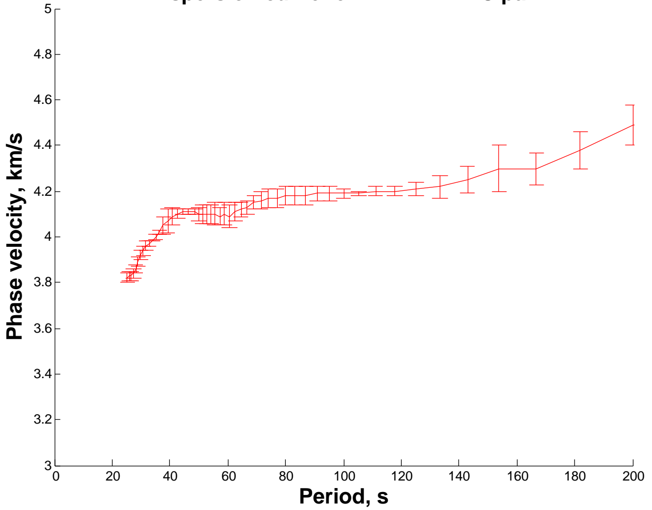
Dispersion curve for WALA BMBC pair
