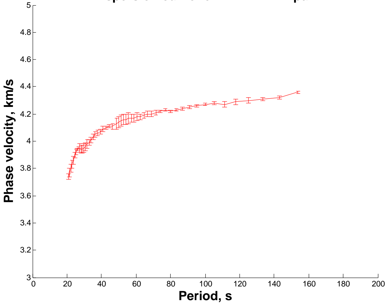
Dispersion curve for DHRN HILA pair
