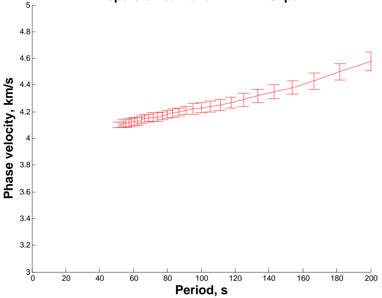
Dispersion curve for PNT RES pair
