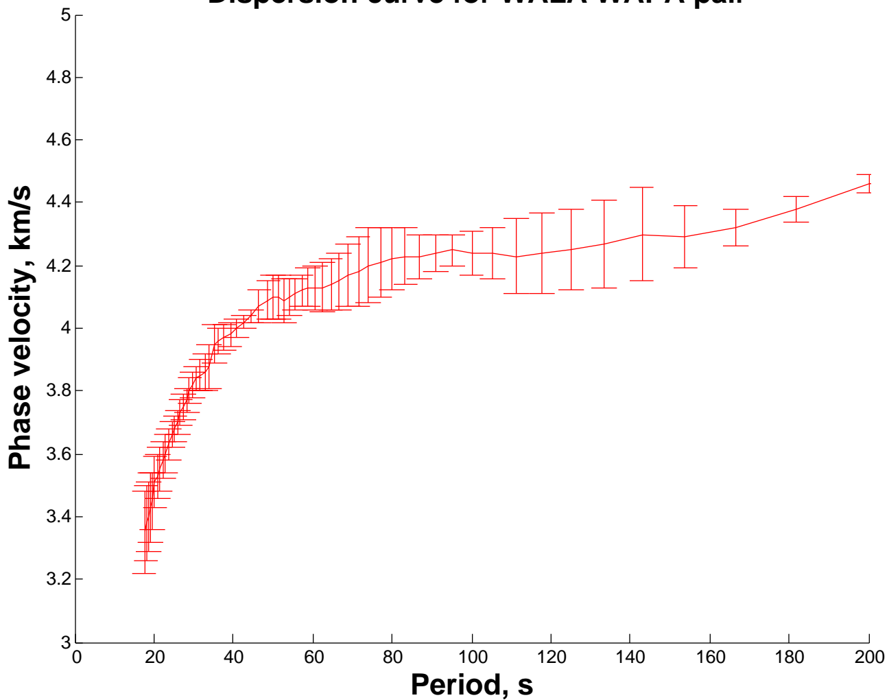
Dispersion curve for WALA WAPA pair
