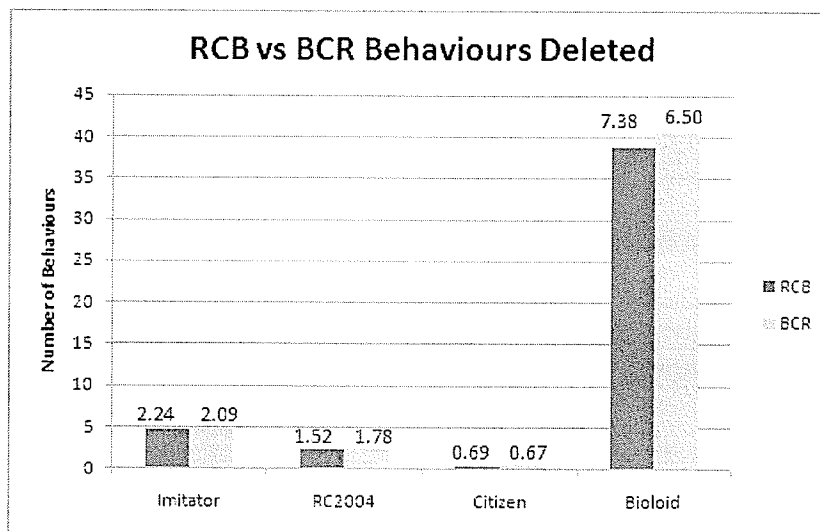
Figure 4.8: The number of behaviours deleted, comparing RCB and BCR demonstrator orderings. Corresponding standard deviations are given at the top of each bar.
