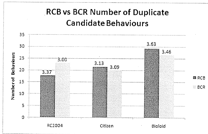
Figure 4.11: The number of candidate behaviours not moved to the forward model representing the imitator, because they were already there, comparing RCB and BCR demonstrator orderings. Corresponding standard deviations are given at the top of each bar.
