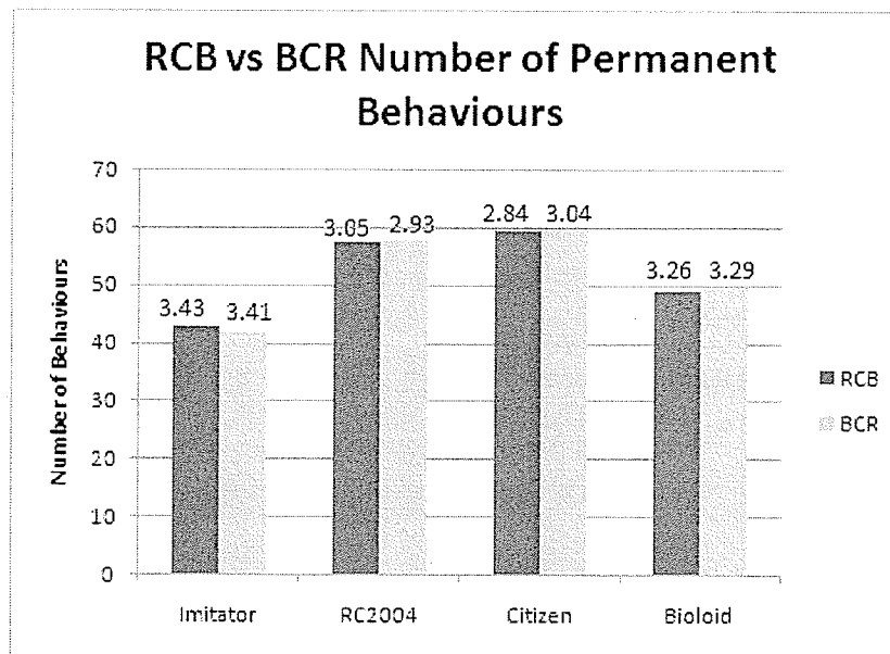
Figure 4.9: The number of permanent behaviours in each forward model, comparing RCB and BCR demonstrator orderings. Corresponding standard deviations are given at the top of each bar.
