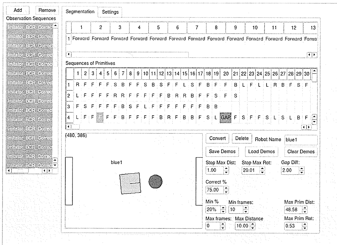
Figure A.4: The application that converts demonstrations into sequences of primitive symbols.
