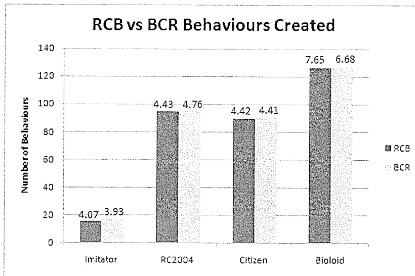
Figure 4.7: The number of behaviours created, comparing RCB and BCR demonstrator orderings. Corresponding standard deviations are given at the top of each bar.
