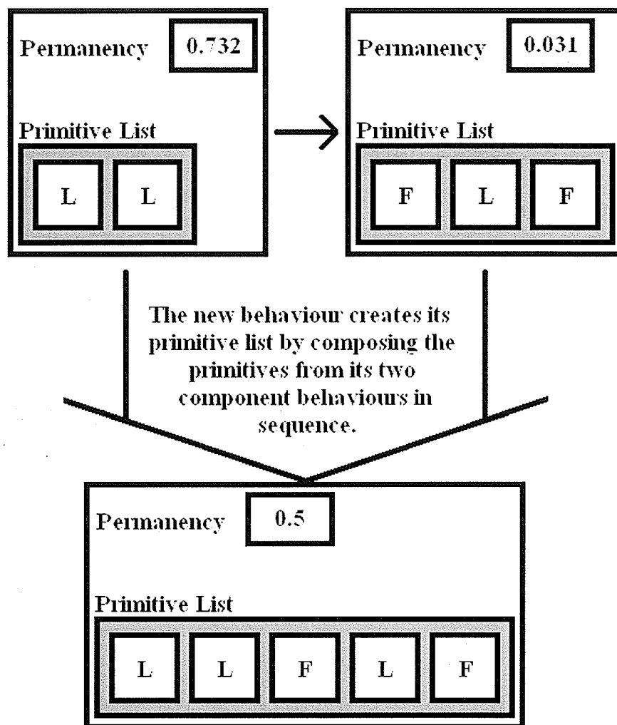
Figure 3.13: The creation of the LLFLF behaviour from the LL and FLF behaviours.
