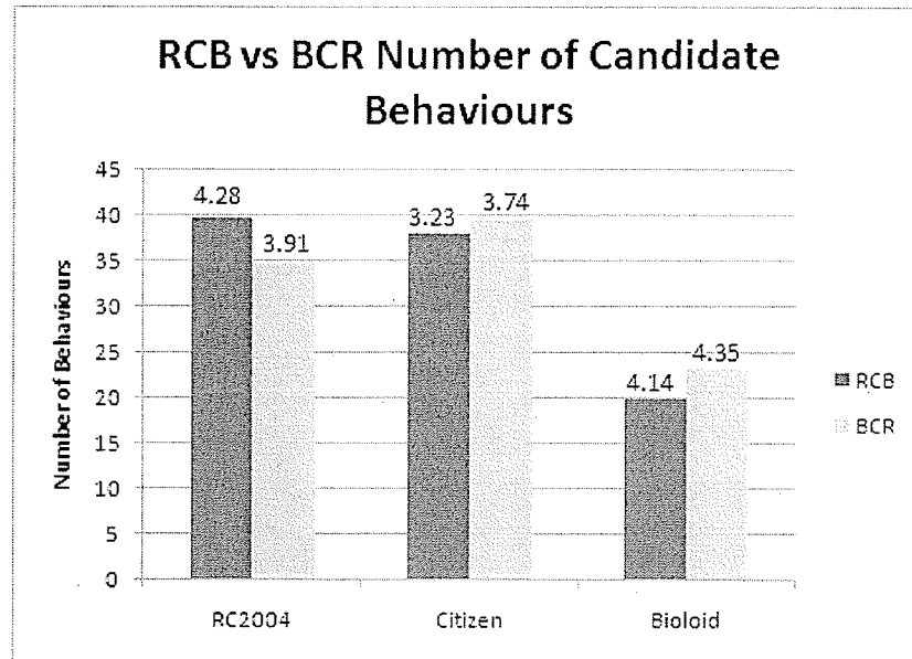
Figure 4.10: The number of candidate behaviours moved to the forward model representing the imitator, comparing RCB and BCR demonstrator orderings. Corresponding standard deviations are given at the top of each bar.
