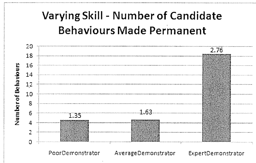
Figure 4.24: The number of candidate behaviours that earned permanency after being moved to the forward model representing the imitator. Corresponding standard deviations are given at the top of each bar.
