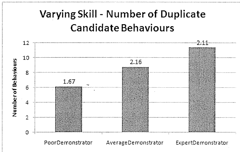
Figure 4.23: The number of candidate behaviours not moved to the forward model representing the imitator because they were already there. Corresponding standard deviations are given at the top of each bar.
