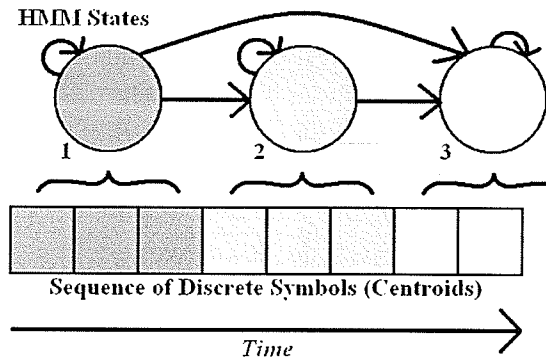
Figure 3.11: Sequences of discrete observation symbols (centroids) from the training data are separated into segments based on when they occur in the sequence.
