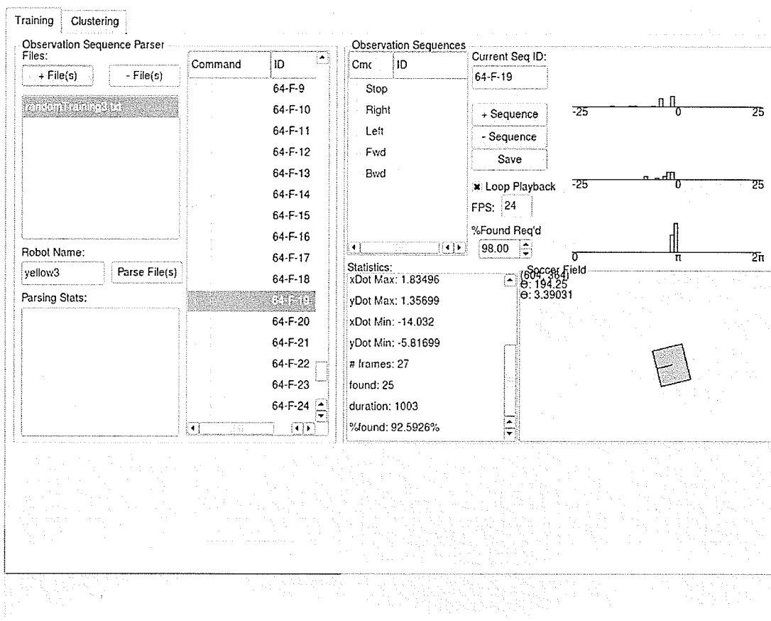
Figure A.1: The application used to sort primitive training data.
