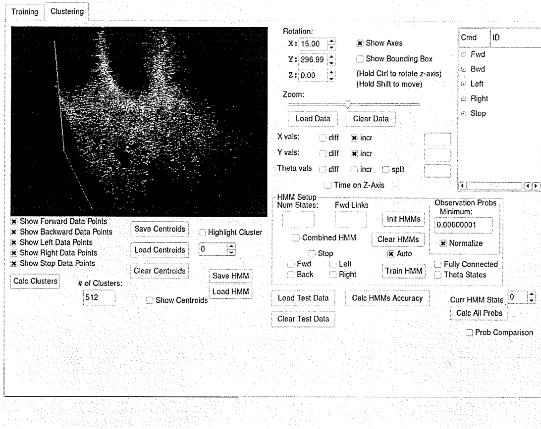
Figure A.2: The application that is used to cluster visual data points and use them to train Hidden Markov Models.
