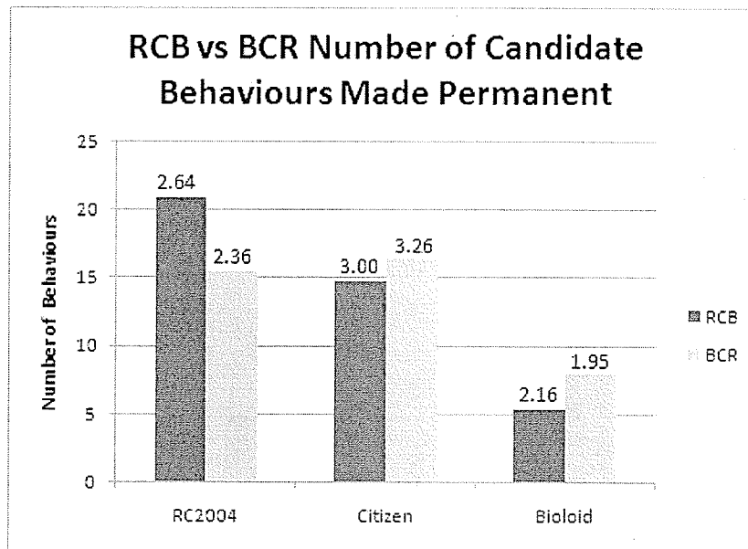
Figure 4.12: The number of candidate behaviours that earned permanency after being moved to the forward model representing the imitator, comparing RCB and BCR demonstrator orderings. Corresponding standard deviations are given at the top of each bar.
