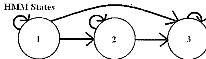
Figure 3.10: An example of an HMM with the left-right topology with two forward links.
