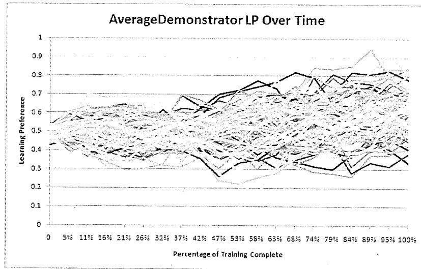
Figure 4.27: The change in LP over time for the AverageDemonstrator.
