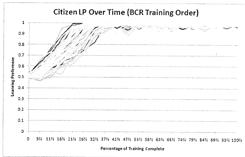
Figure 4.16: The change in LP over time for the Citizen demonstrator (BCR ordering).
