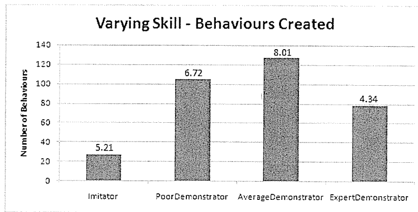
Figure 4.19: The number of behaviours created. Corresponding standard deviations are given at the top of each bar.
