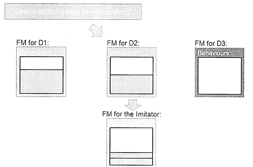
Figure 1.3: Demonstrations from demonstrator 2 are used to train the forward model representing demonstrator 2. Frequently occurring candidate behaviours are moved to the forward model representing the imitator.
