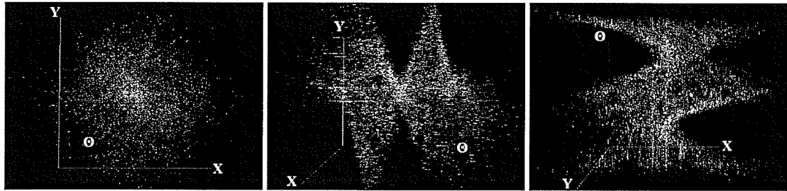
Figure 3.6: The positional visual sequence processing method, shown for all data points from all primitive training sequences. Left to right: front view, side view, top view.
