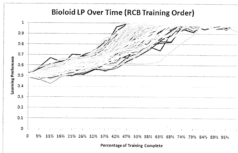
Figure 4.17: The change in LP over time for the Bioid demonstrator (RCB ordering).
