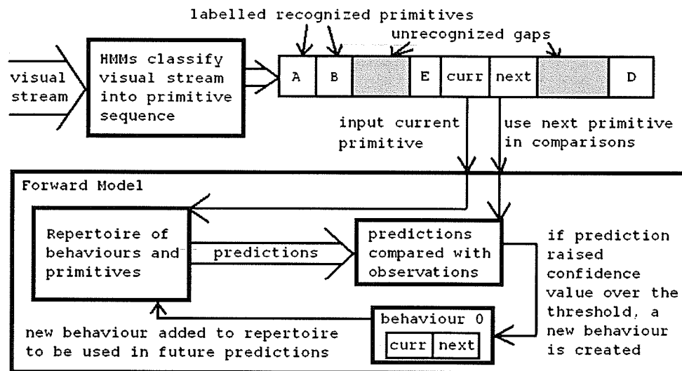
Figure 3.16: Imitation Learning Architecture
