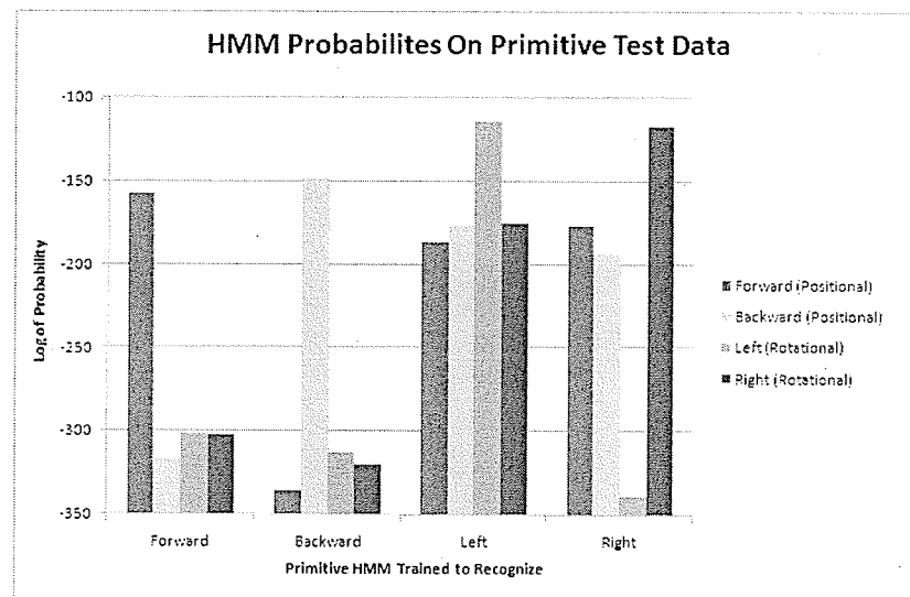
Figure 4.5: The average probabilities for each HMM type on the primitive test data.
