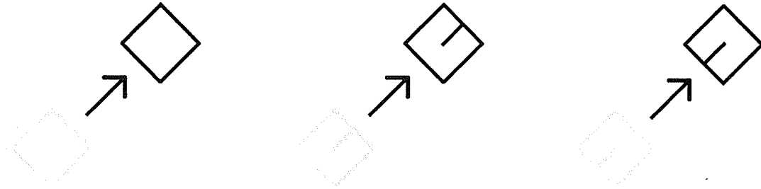
Figure 3.5: Difficulty distinguishing the difference between forward and backward motion. Without absolute \theta , the left image could represent either a forward (middle) or backward (right) primitive.
