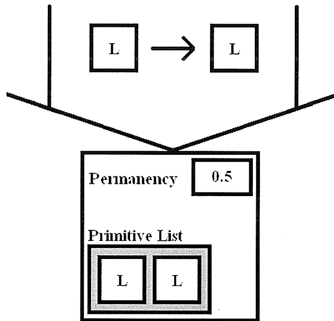
Figure 3.12: A new behaviour is created to encompass two left primitives occurring in sequence.
