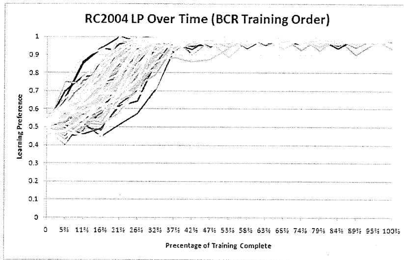
Figure 4.14: The change in LP over time for the RC2004 demonstrator (BCR ordering).
