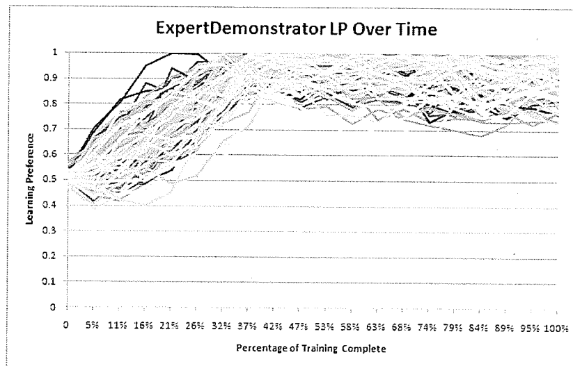
Figure 4.28: The change in LP over time for the ExpertDemonstrator.
