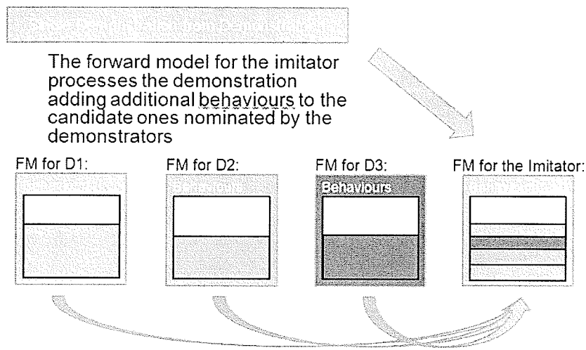
Figure 1.5: In the final phase of training, all demonstrations are first passed to the demonstrator models to elicit any candidate behaviour nominations before the forward model for the imitator processes the demonstration.
