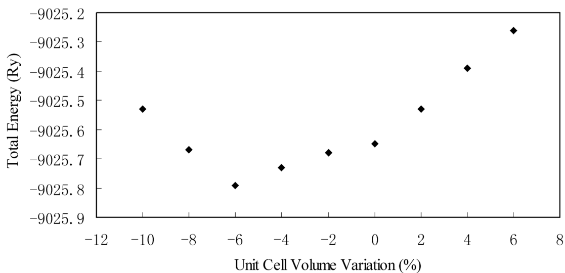
Figure 3. Structural energy (Ry) as a function of cell volume change (%) for ulexite
