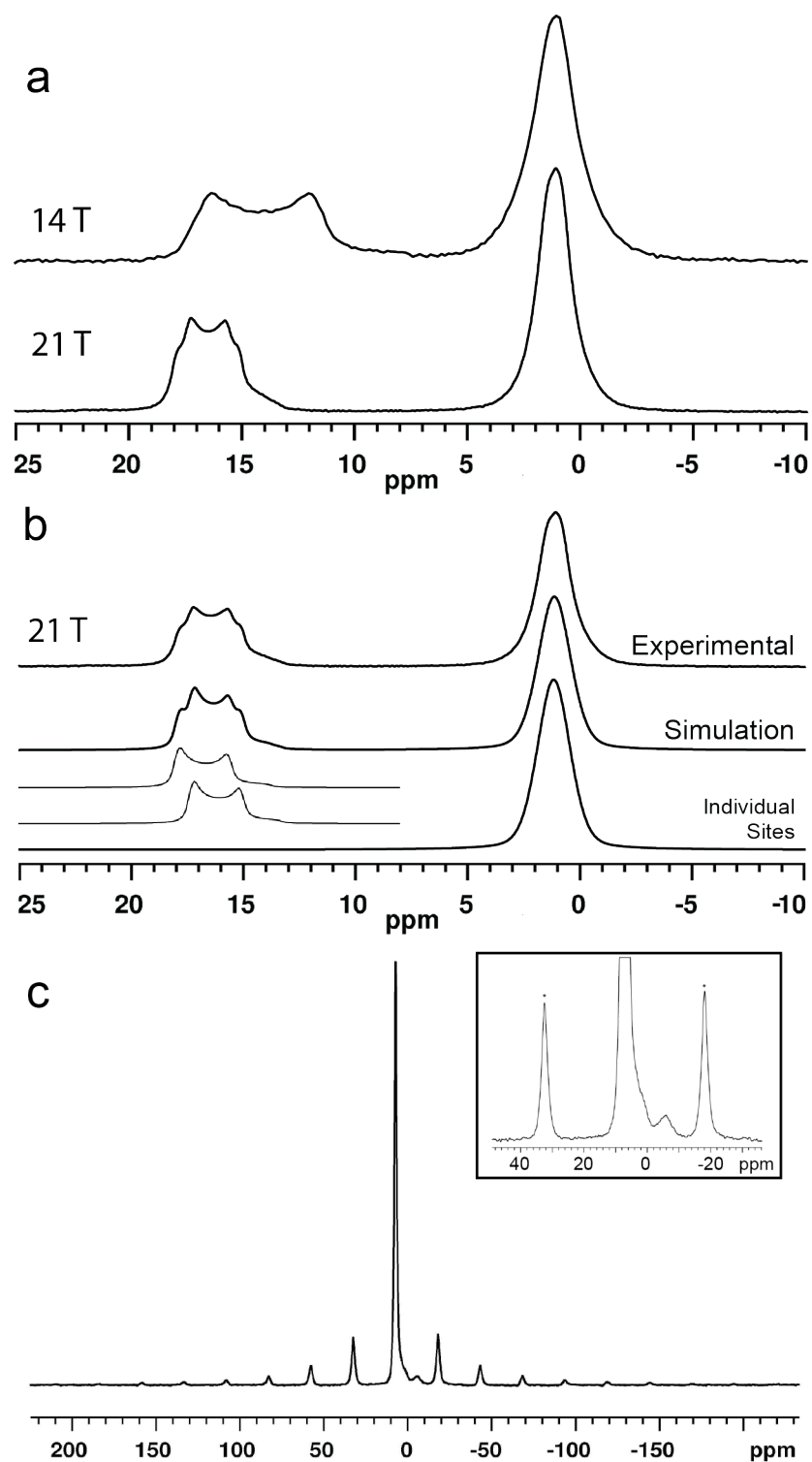
Figure 2. (a) ^{11}\text{B} MAS NMR spectra of ulexite at 14.1 T and 21.1 T; (b) lineshape fitted to the 21.1 T data; (c) ^{23}\text{Na} MAS NMR (14.1 T) spectrum of ulexite. Inset is a 10x increase in vertical scale illustrating a small impurity resonance at -6 ppm (spinning sidebands are identified by asterisks).
