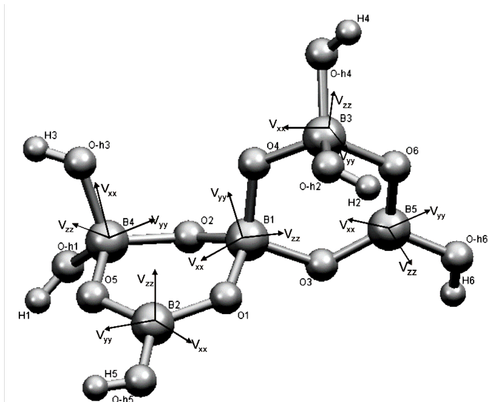
Figure 1. Fundamental building block of ulexite, with boron EFG tensor orientations
