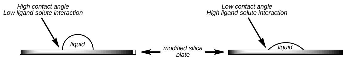
Figure 1.4.3.4: Schematic of liquid-surface contact angles.
