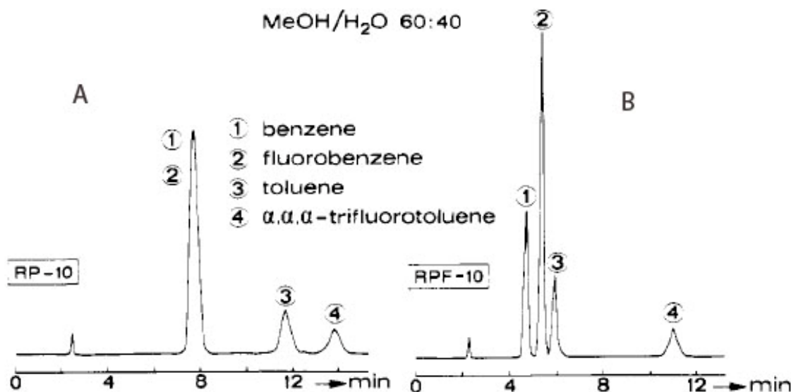
Figure 1.4.3.2: Comparison of retention times for fluorinated and non-fluorinated benzenes on alkyl (RP-10, A) and fluorocarbon (RPF-10, B) bonded phases. 137
