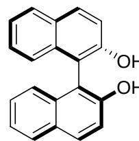
S -BINOL
