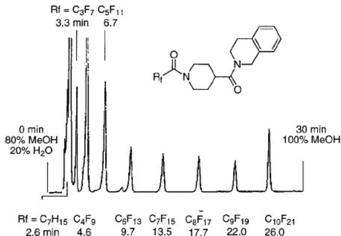
Figure 1.4.3.3: Separation of materials by fluorine content using fluorosilica gel 130
