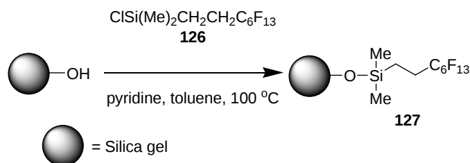
Scheme 1.4.3.1: Formation of fluorosilane reverse phase silica gel.
