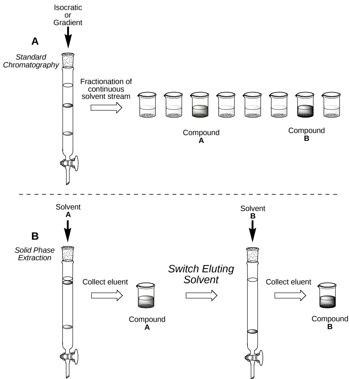
Figure 1.4.3.1: Comparison of chromatography and solid phase extraction.
