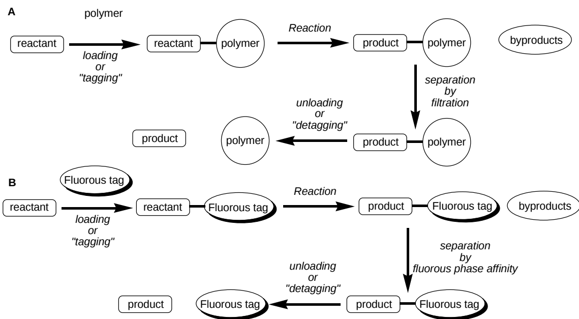
Figure 1.4.1.1: Schematic of polymer-supported and fluorous-supported methods.
