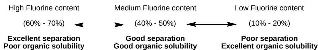
Figure 1.4.2.1: Balance between fluororous and organic solubility.
