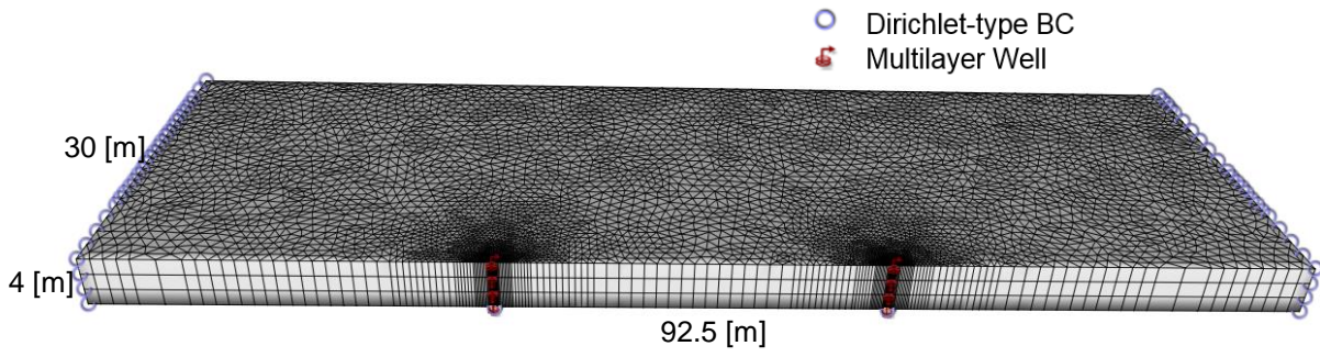
Fig. 4 Schematic representation of the numerical 3 layer model including boundary conditions
