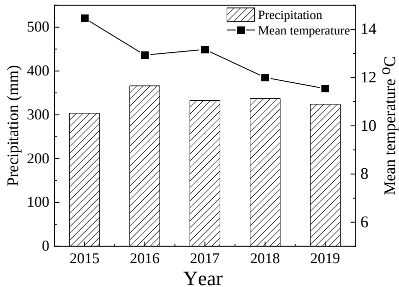
Figure 2. 1 Growing season (May to October) precipitation and mean growing season temperature during 2015-2019 at the borrow pit at Cold Lake, Alberta, Canada.
