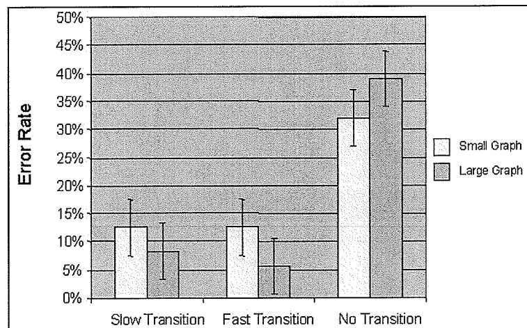
Figure 14 – Experiment 1: Average Error Rates by transition style and graph size
