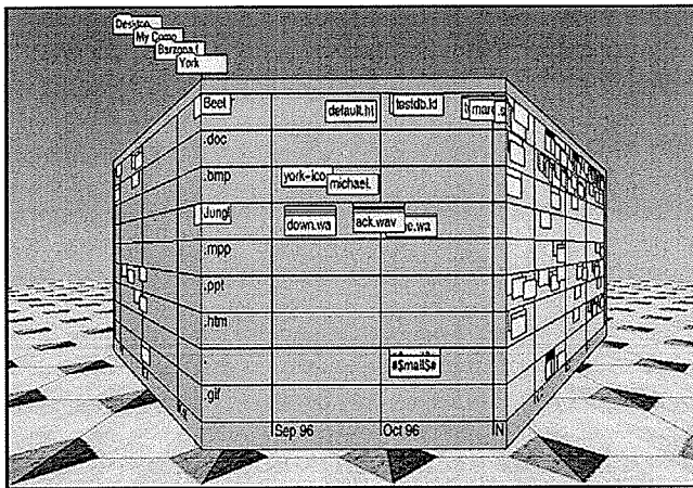
(a) Perspective Wall
