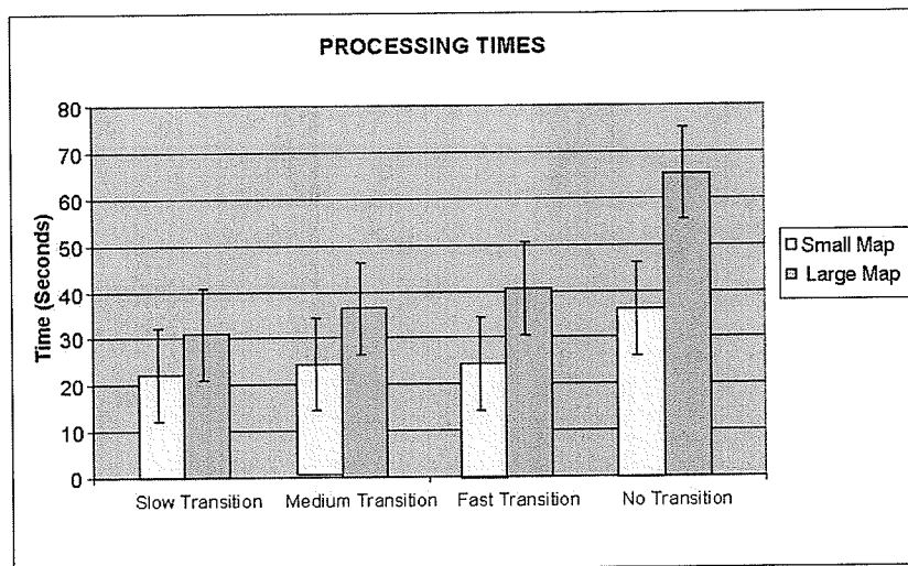
Figure 29 – Experiment 4: Task Processing Times by transition style and map size
