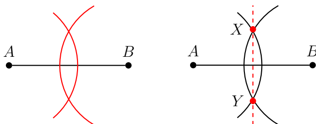
Figure 1.23: Constructing perpendicular bisector of AB
