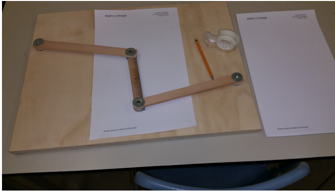
Figure 1.37: Watt's linkage, pencil goes in hole in central bar, DSG 2016
