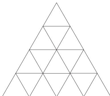
Figure 1.41: Count the triangles; n = 4
