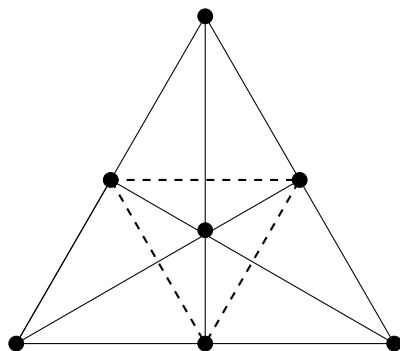
Figure 15.3: The Kelly–Moser configuration with Gallai lines dashed
