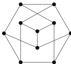
Figure 24.12: The Petersen graph with 3 crossings
