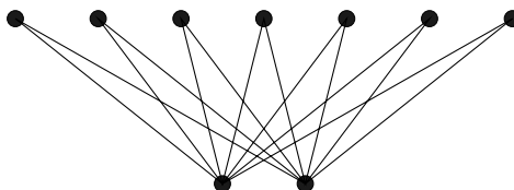
Figure 2.4: K_{2,7} , drawn vertically.
