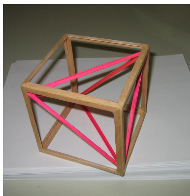
Figure 3.5: A tetrahedron in a cube, made from coffee stir sticks, 2003
