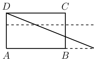
Figure 8.3: Rectangle into rectangle with given base
