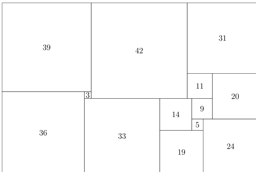
Figure 10.10: Mrs. Brooks' arrangement of a squared 112 \times 75 rectangle
