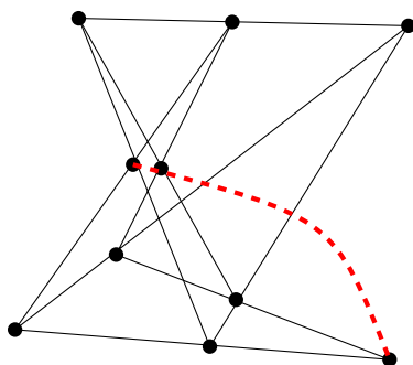
Figure 15.11: The only (10_3) configuration that is not geometric
