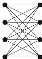
Figure 2.3: Standard drawing of K_{4,4} .
