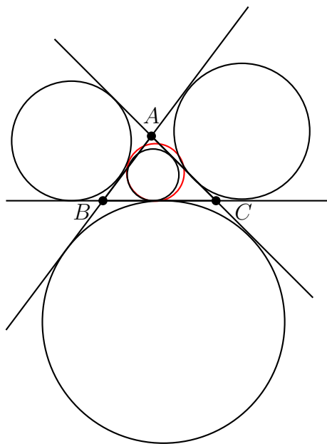
Figure 1.9: Feuerbach's theorem, nine-point circle in red
