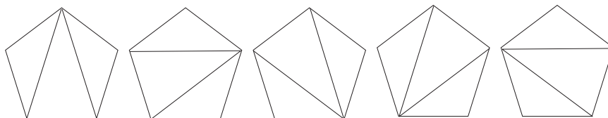
Figure 1.5: Five ways to triangulate a pentagon
