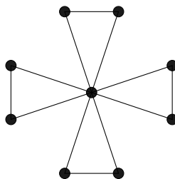
Figure 11.4: Friendship graph F_4
