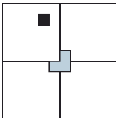
Figure 24.7: The idea behind Golomb's inductive step
