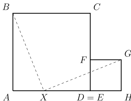
Figure 8.7: Thābit's dissection of two squares into one
