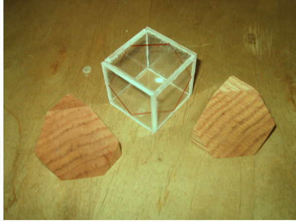
Figure 3.7: Bisecting a cube with a regular hexagon, DSG, 2003?
