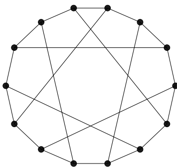
Figure 11.3: Heawood graph, 14 vertices; incidence graph for Fano plane
