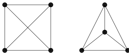
Figure 2.5: The standard drawing of K_4 and a plane drawing
