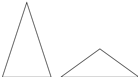
Figure 1.15: The two golden triangles
