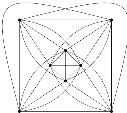
Figure 17.6: cr(K_8) \leq 18
