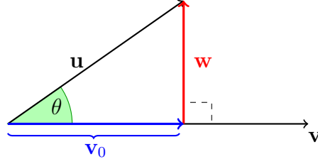
Figure 23.1: Projecting \mathbf{u} onto \mathbf{v}
