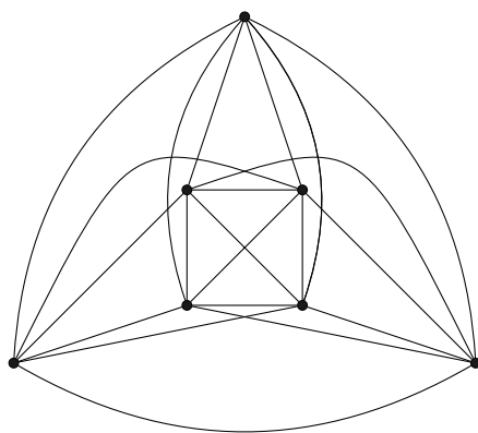
Figure 24.14: \text{cr}(K_7) \leq 9
