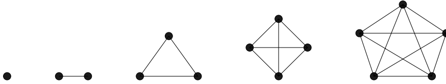
Figure 2.2: Small complete graphs: K_1 , K_2 , K_3 , K_4 , K_5
