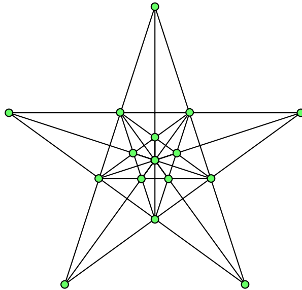
Figure 15.5: A 15 row solution to the ploughman's puzzle, given by Dudeney [271, p.140]
