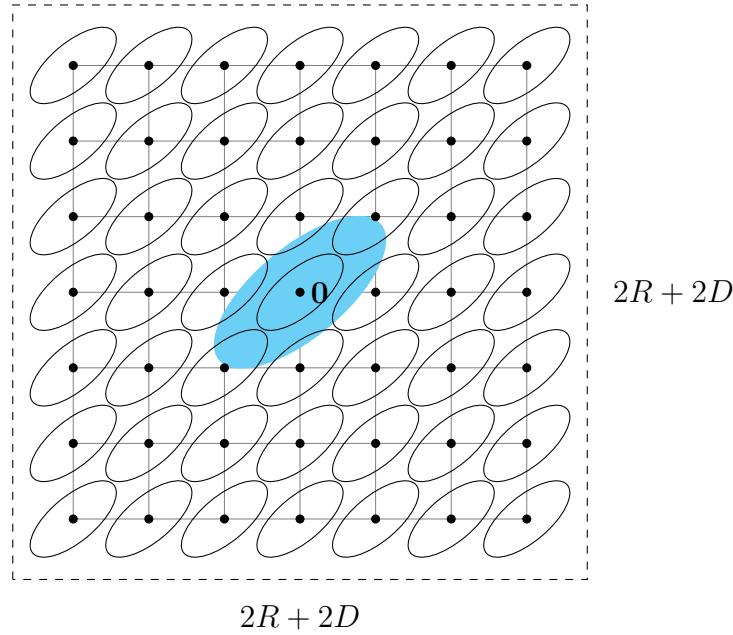
Figure 9.1: A step in the proof of Minkowski's theorem showing copies of C' , with R = 3 and C in cyan.
