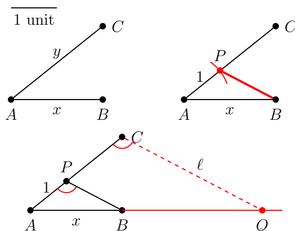
Figure 1.28: Multiplication
