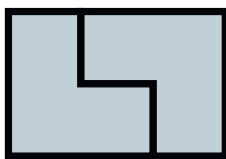
Figure 24.5: A 2 \times 3 configuration
