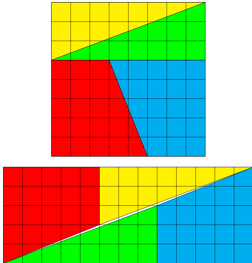
Figure 8.12: Top area is 8 \times 8 = 64 ; bottom is 13 \times 5 = 65 ?
