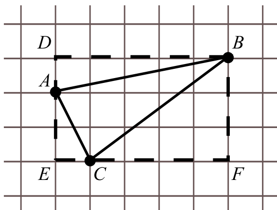
Figure 1.6: Finding area of arbitrary triangle
