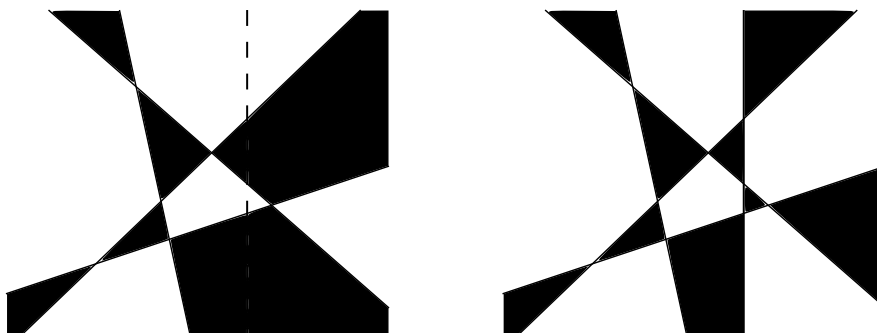
Figure 24.8: The new colouring after a line is added
