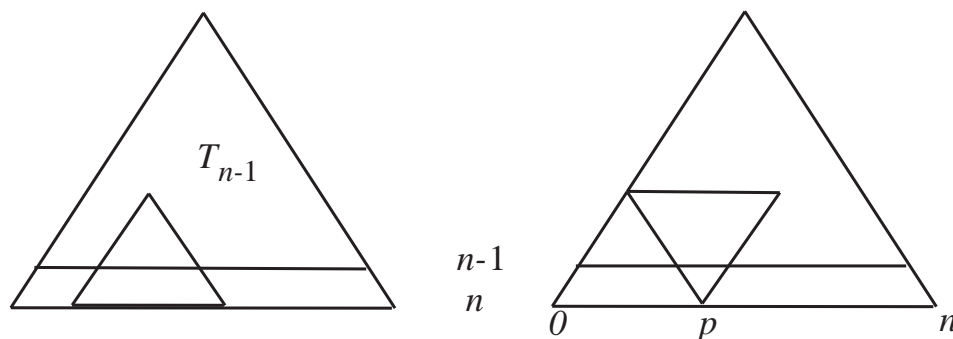
Figure 24.1: Counting triangles in T_n
