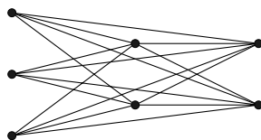
Figure 17.2: The graph K_{3,2,2}
