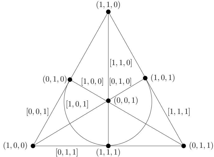
Figure 11.2: The Fano plane \text{PG}(2, 2) = \mathcal{P}(2) with homogeneous coordinates
