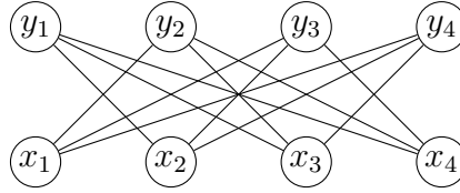
Figure 21.3: The standard example S_4 .
