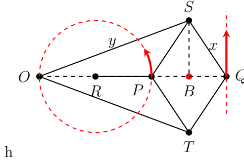
Figure 1.39: Peaucellier's linkage
