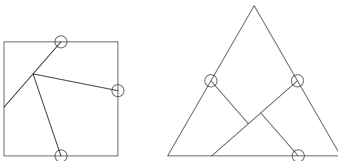
Figure 8.8: Hinged dissection of an equilateral triangle to a square, by DSG
