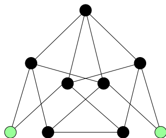
Figure 17.12: The 9 point unit distance graph used by de Grey
