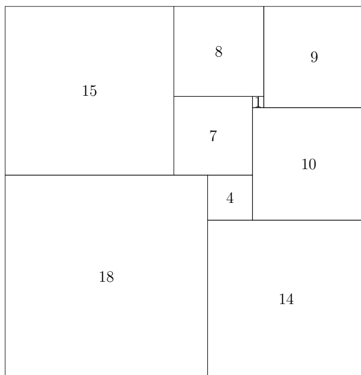
Figure 10.2: Moron's order 9 perfect squaring of a 32 \times 33 rectangle
