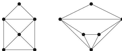
Figure 2.8: Isomorphic graphs with different plane drawings and different multigraph duals.
