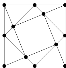
Figure 15.10: A (12_3) configuration
