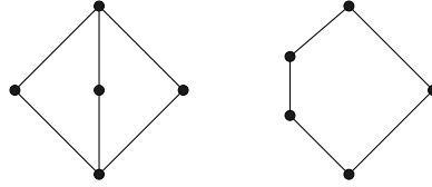
Figure 21.1: Lattices M_3 and N_5
