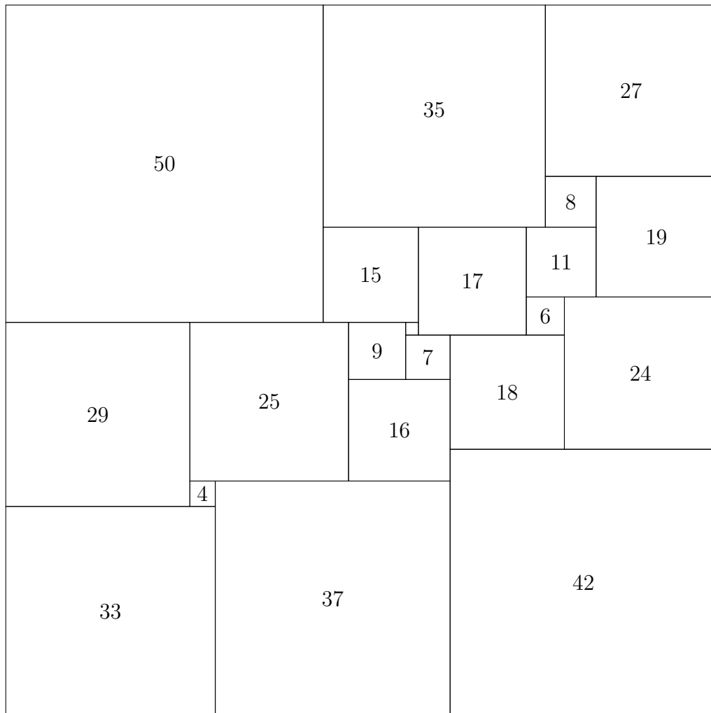
Figure 10.7: Duijvestijn's perfect squaring of 112 \times 112 with 21 unequal squares, where the unlabelled square is 2 \times 2
