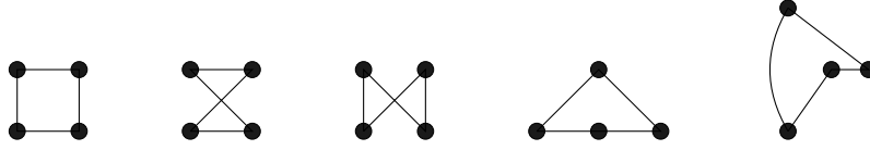
Figure 2.1: Five isomorphic graphs.
