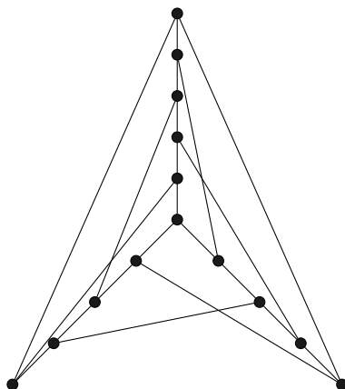
Figure 17.4: The Heawood graph with 3 crossings
