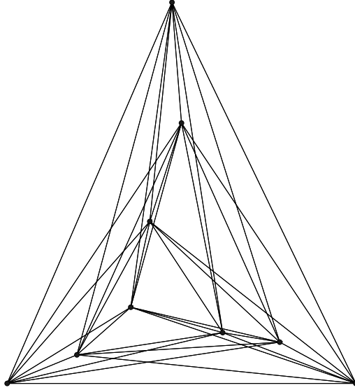
Figure 17.8: \overline{\text{cr}}(K_9) \leq 36 , drawing from [457, Fig. 7].
