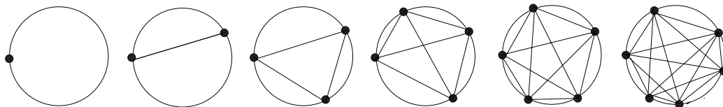
Figure 16.1: Cutting the cake
