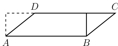
Figure 8.2: Parallelogram into rectangle
