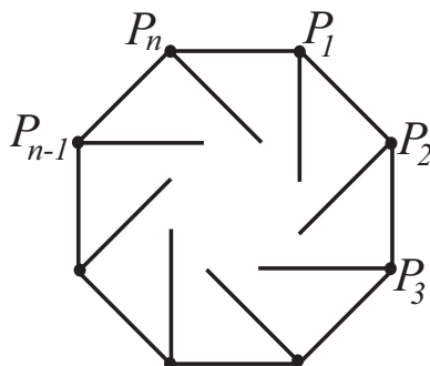
Figure 24.4: Making a smaller n -gon
