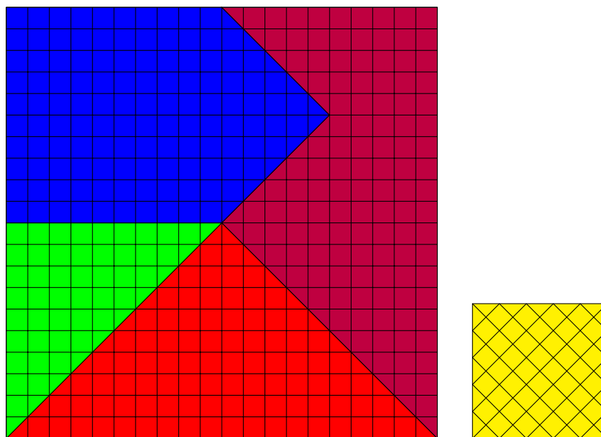
Figure 8.4: The Pythagorean-square puzzle: rearrange the five pieces into a square
