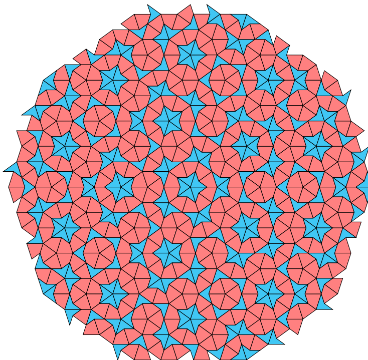
Figure 1.17: A Penrose tiling (based on code from StackExchange)
