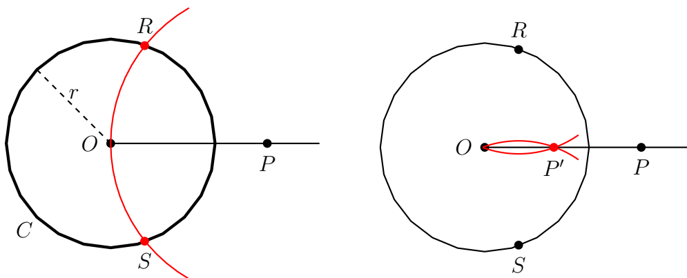
Figure 1.35: Inversion with respect to the circle C for P outside C
