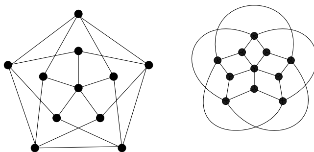
Figure 15.12: Drawings of the Grötzsch graph, 4-chromatic, girth 4, 11 vertices
