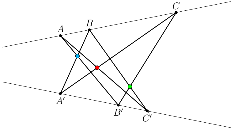
Figure 1.2: The Pappus configuration. The three coloured points are collinear.
