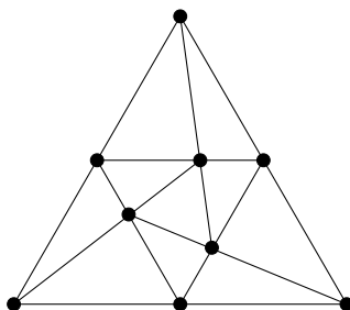
Figure 15.9: One of the two (9_3) configurations other than Pappus
