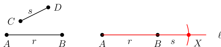
Figure 1.22: Addition
