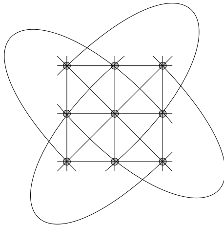
Figure 15.8: The Hesse (9_4, 12_3) configuration, \text{AG}(2, 3)
