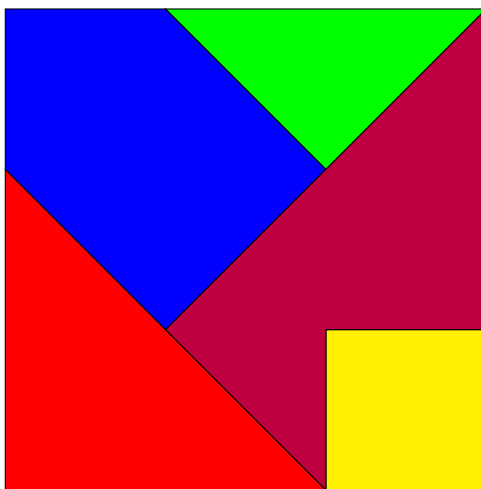
Figure 8.5: A Pythagorean-square puzzle solution
