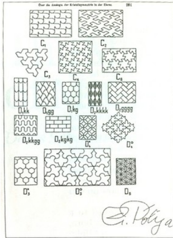
Figure 4.3: Polyá's 1924 sketch of 17 patterns for wallpaper groups
