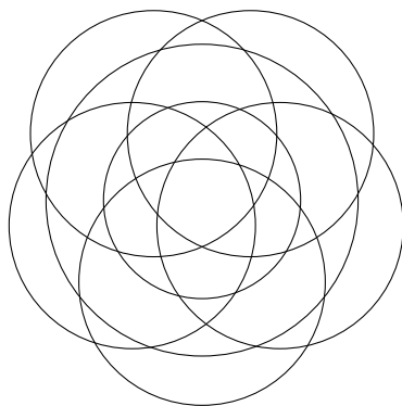
Figure 15.15: Koester's critical 4-chromatic graph given by 7 circles
