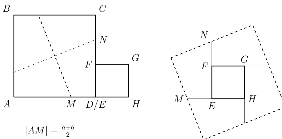
Figure 8.6: Perigal's dissection of two squares into one
