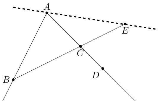
Figure 15.2: Lin’s proof of the Sylvester–Gallai theorem
