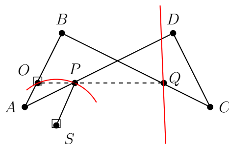
Figure 1.40: The first Hart's linkage with 5 rods
