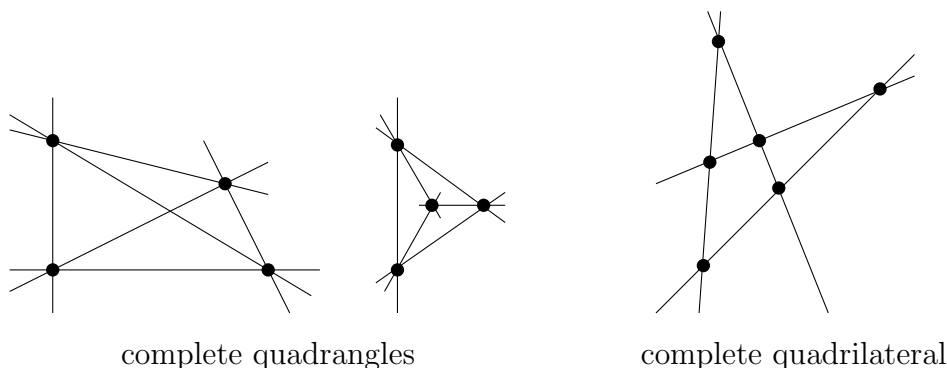
Figure 11.1: Two complete quadrangles (frames) and a complete quadrilateral
