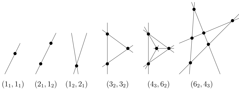
Figure 15.7: Some small configurations
