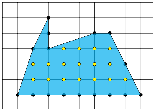
Figure 1.7: Pick's theorem: I(P) = 17 , B(P) = 16 ; area = 24.
