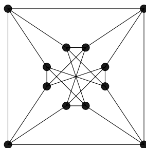
Figure 15.13: Chvátal's Graph, 4-chromatic, 4-regular, girth 4, 12 vertices
