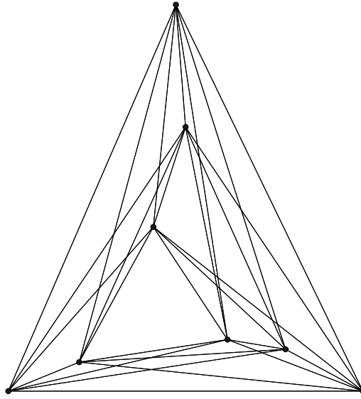
Figure 17.7: \overline{\text{cr}}(K_8) \leq 19 , drawing from [457, Fig. 6].
