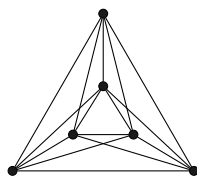
Figure 17.1: Drawing for \text{cr}(K_6) \leq 3
