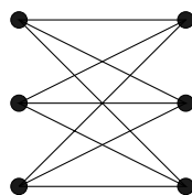
Figure 2.7: Standard drawing of K_{3,3}
