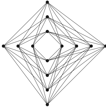
Figure 17.5: \text{cr}(K_{7,7}) \leq 81
