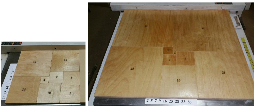
Figure 10.5: The two perfect squarings of (minimal) order 9 as puzzles.
