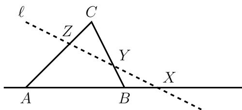
Figure 1.1: An example for Menelaus's theorem
