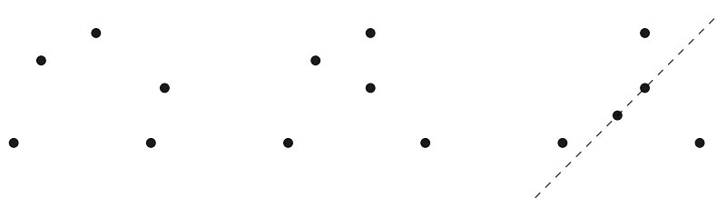
Figure 24.3: 5 points in general position
