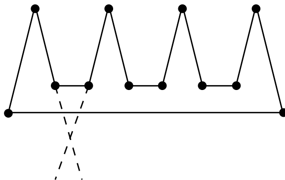
Figure 24.2: An art gallery with 12 vertices requiring 4 guards
