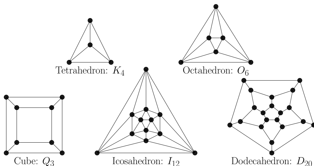
Figure 2.6: Planar graphs of the 5 Platonic Solids
