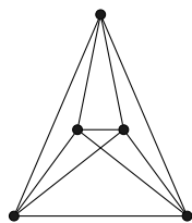
Figure 24.9: Drawing for \text{cr}(K_5) \leq 1
