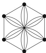
Figure 24.15: Is \text{cr}^*(K_6) = 1 ?
