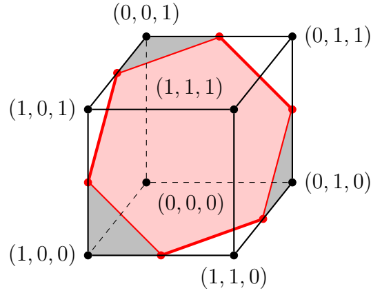
Figure 3.7: Bisecting a cube with a regular hexagon, DSG, 2003?
