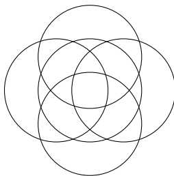
Figure 15.14: Koester's 4-chromatic graph given by 5 circles
