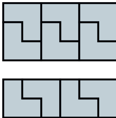
Figure 24.6: Ways to tile an n \times 6 board
