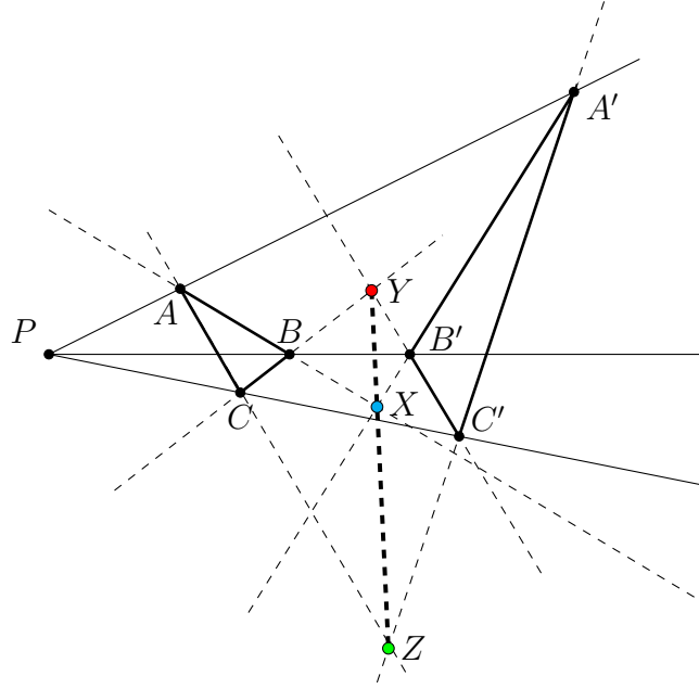
Figure 1.3: Desargues' configuration
