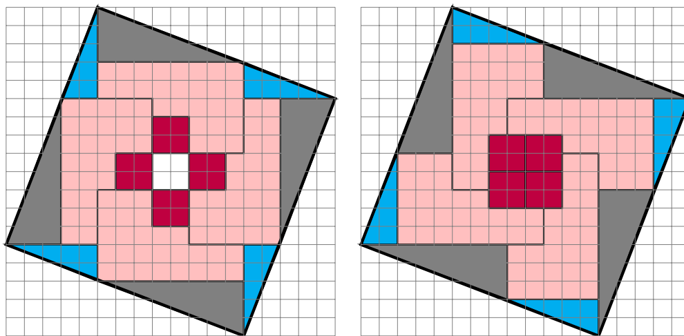
Figure 8.14: Gardner's missing tile puzzle: where did the white tile go?
