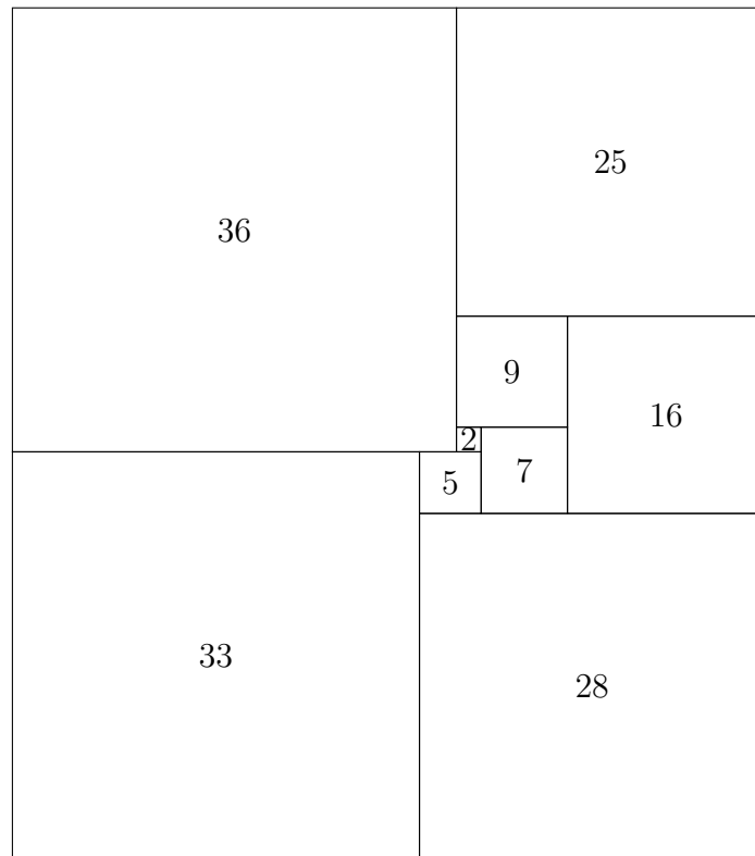
Figure 10.4: Order 9 perfect squaring by Brooks, Smith, Stone, and Tutte
