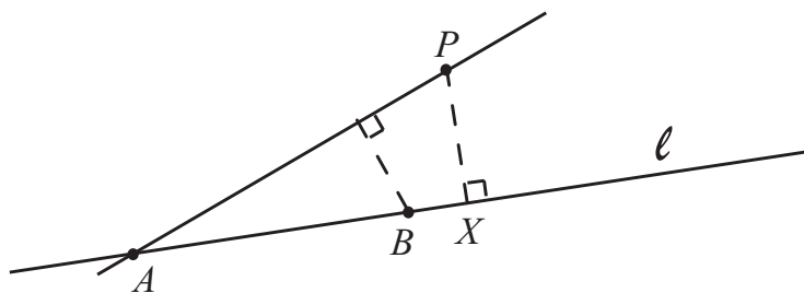
Figure 15.1: Kelly’s proof
