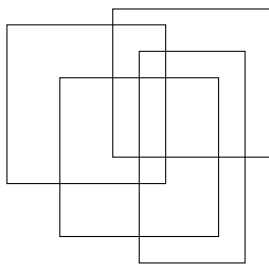
Figure 5.1: Four rectangles, any two of which intersect
