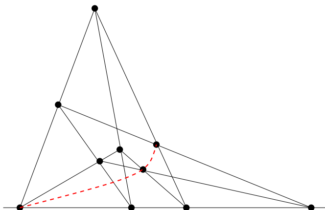
Figure 15.6: Killgrove's k -configuration
