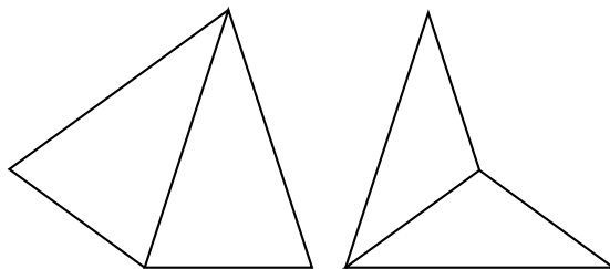
Figure 1.16: Kite and dart, the two Penrose tiles
