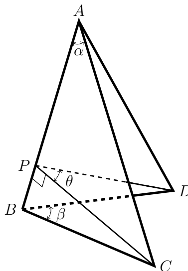
Figure 3.10: Dihedral angle \theta between isosceles triangles
