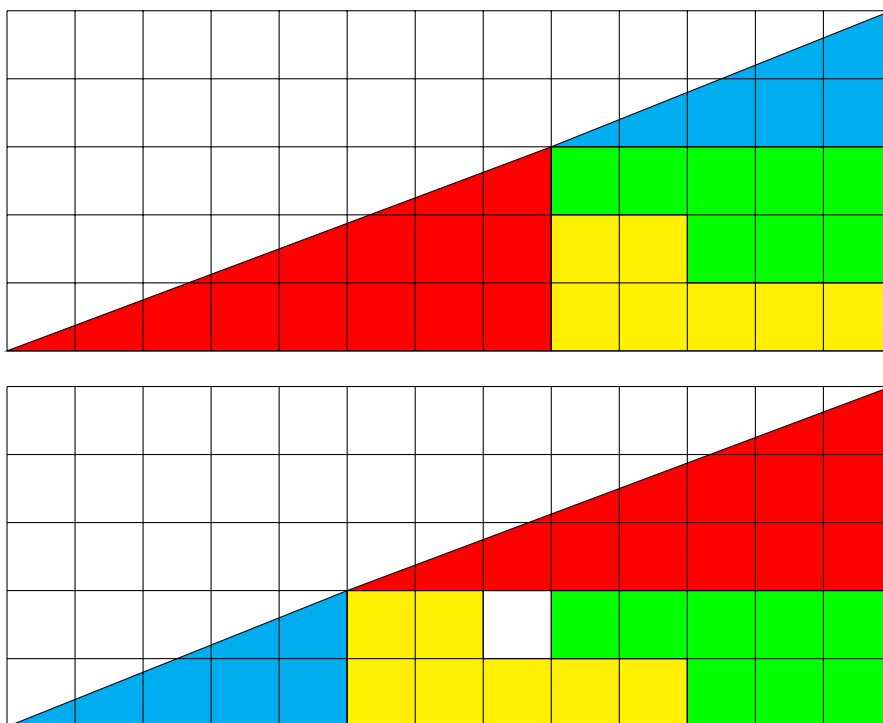
Figure 8.13: Curry’s paradox: where did the hole come from?
