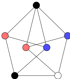
Figure 17.10: Moser’s unit-distance graph, not 3-colourable
