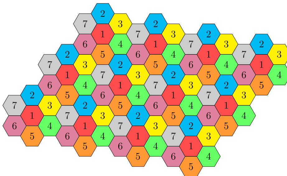
Figure 17.11: Isbell's 7-colouring of the plane
