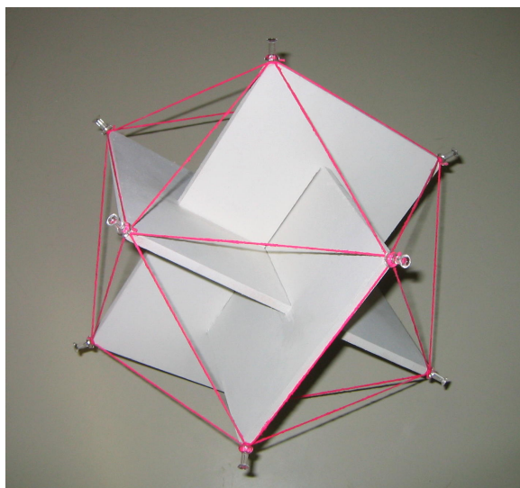
Figure 1.20: Three intersecting golden rectangles
