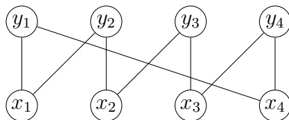
Figure 21.2: The crown poset C_4 .
