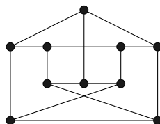
Figure 24.13: \text{cr}(\text{Petersen graph}) \leq 2
