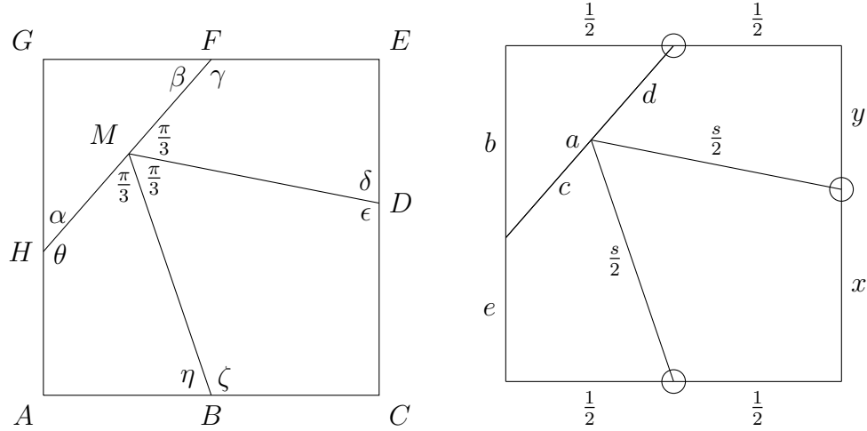
Figure 8.10: Labelling for square-to-triangle dissection
