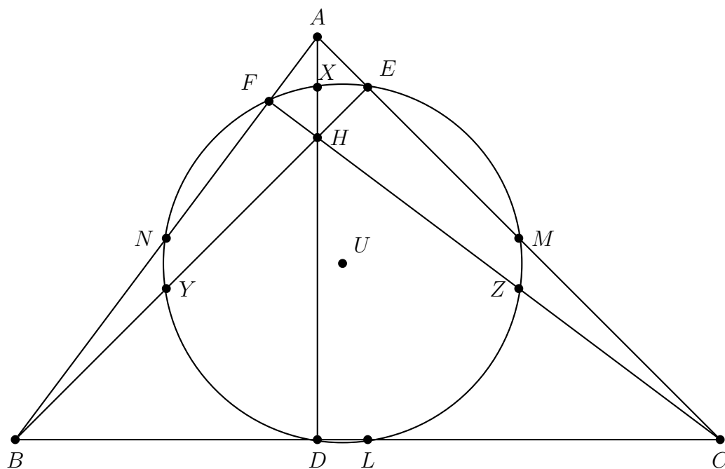
Figure 1.8: The nine-point circle for triangle \triangle ABC
