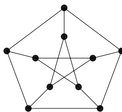
Figure 17.3: A standard drawing of the Petersen graph with 5 crossings
