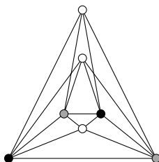
Figure 24.11: \text{cr}(K_{3,2,2}) \leq 2
