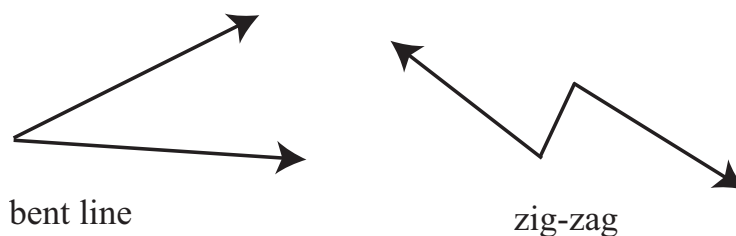
Figure 16.2: Partitioning the plane with other shapes
