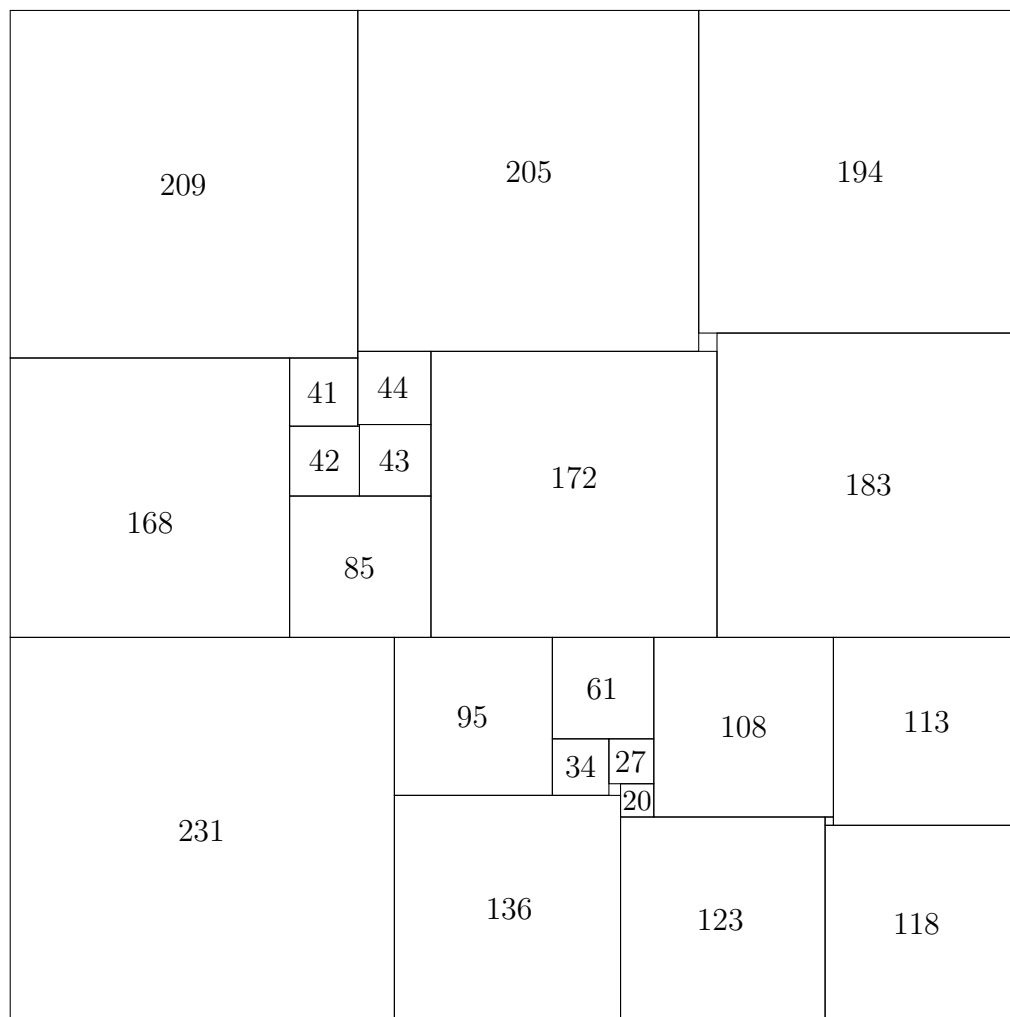
Figure 10.3: A compound perfect 608 \times 608 square of order 26 by Brooks, Smith, Stone, and Tutte (3 squares unlabelled, including a unit square at the corners of the 41, 42, 43, and 44 squares, the other two of sizes 5 and 11)
