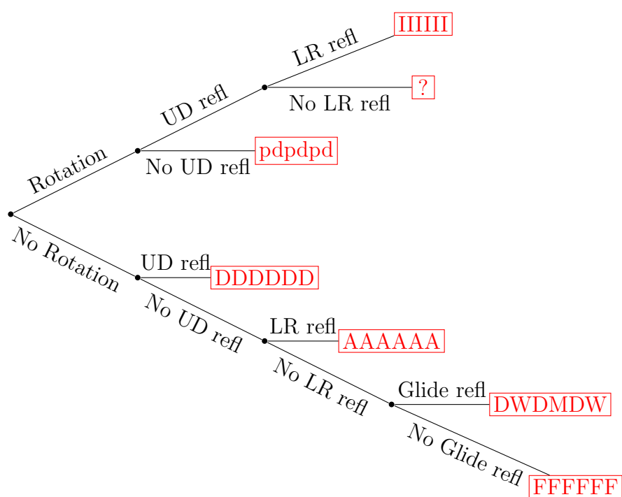
Figure 4.2: Frieze pattern flow chart
