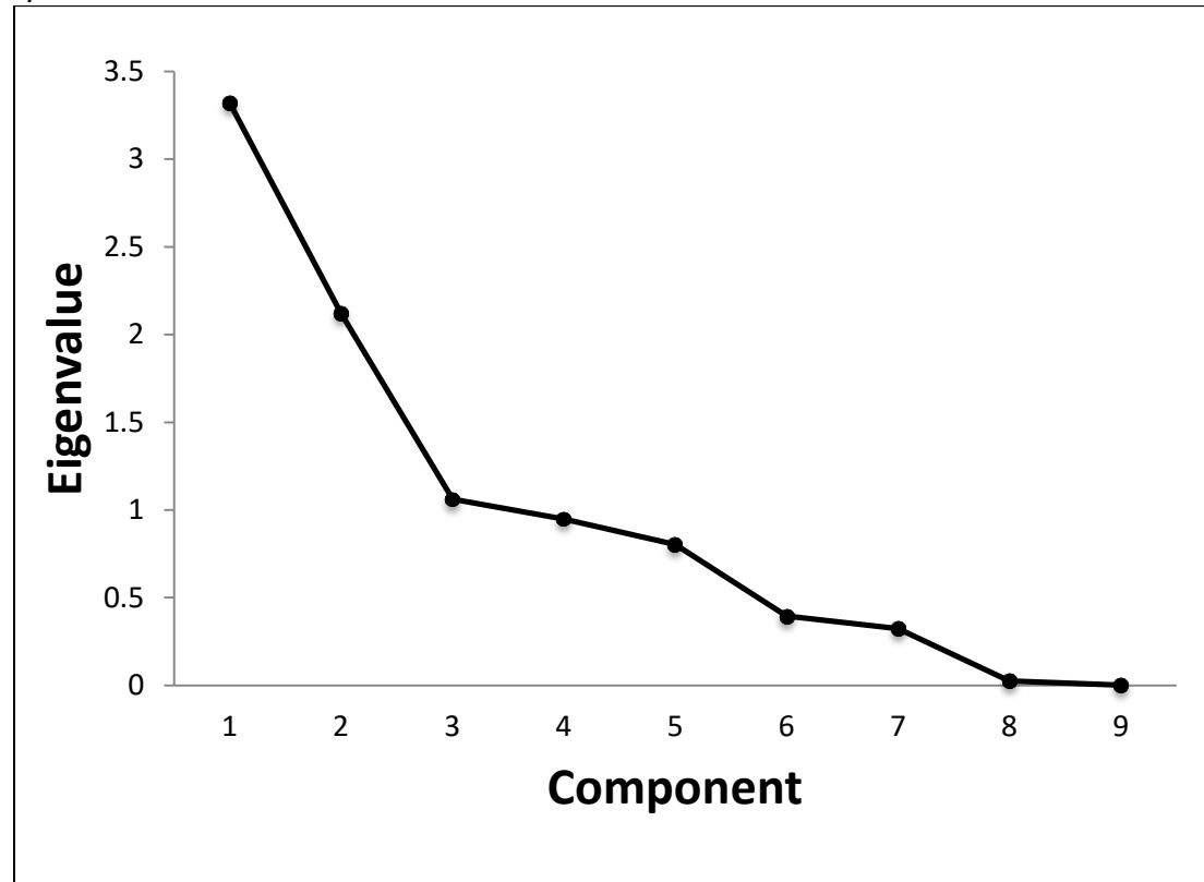
Figure B1. Scree plot for components in principal components analysis. Only components with eigenvalues greater than one were retained for further analysis.
