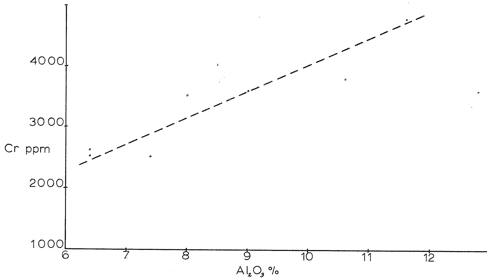
Fig. 4. Plot of chromium against \text{Al}_2\text{O}_3 .
