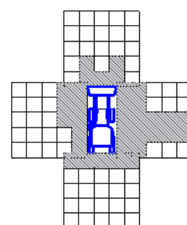
Figure 8 Visibility results for Tractor 1 at the kneeling worker height for a slumped sitting position.
