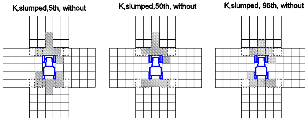
Figure 16 Visibility results for Tractor 2 at the kneeling worker level for a slumped sitting position.
