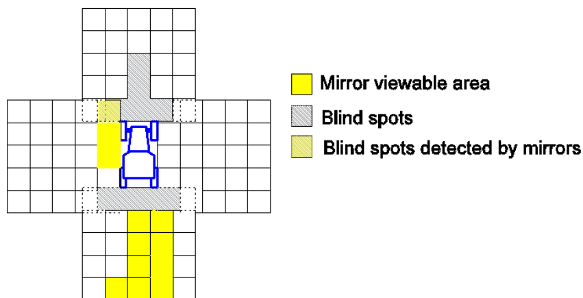
Figure 22 Mirrors detection area of Tractor 2.
