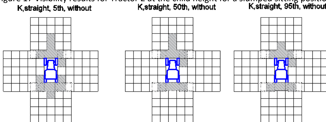
Figure 18 Visibility results for Tractor 2 at Kneeling worker height for a straight sitting position.
