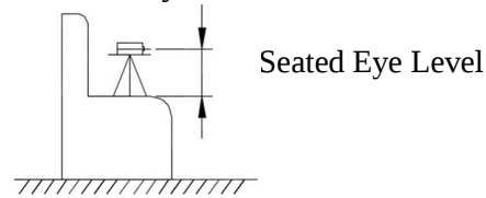
Figure 6 Camera set-up.
