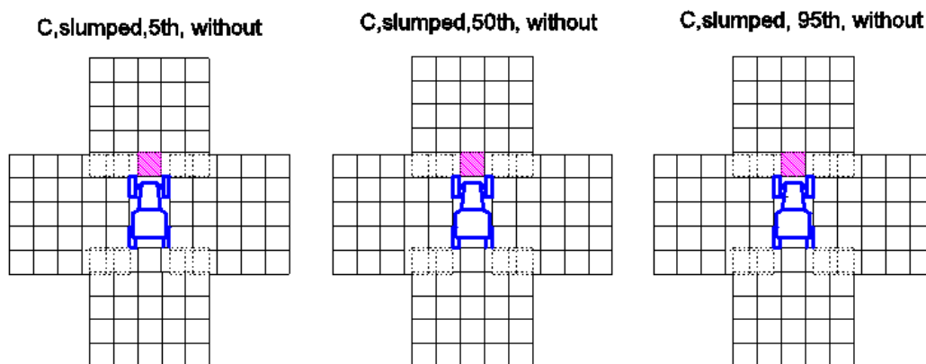
Figure 17 Visibility results for Tractor 2 at the child height for a slumped sitting position.
