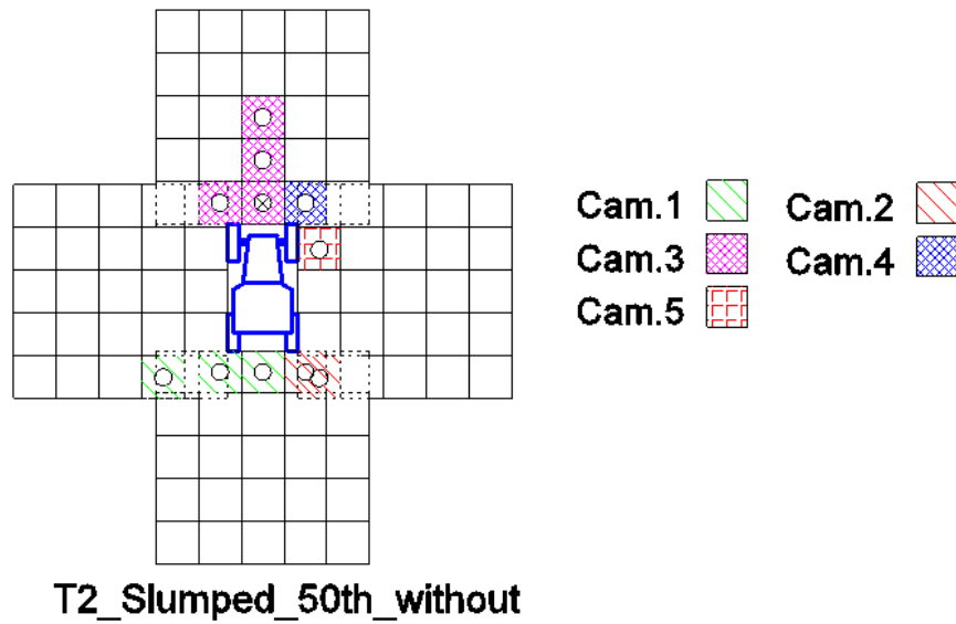
Figure 26 Detection zone for each cameras for Tractor 2.
