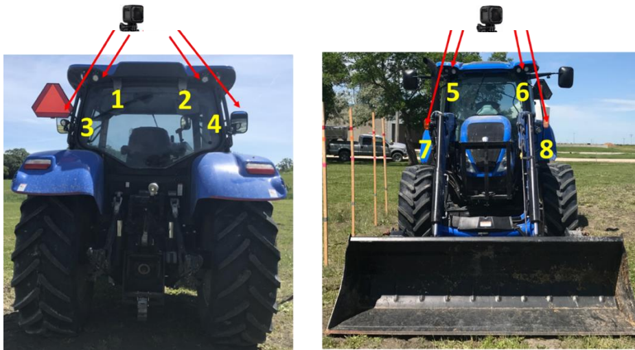
Figure 23 Locations of recommended cameras for Tractor 1.
