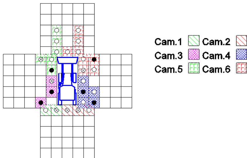
Figure 23 Locations of recommended cameras for Tractor 1.
