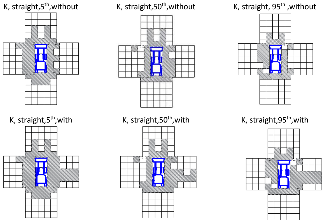
Figure 12 Visibility results for Tractor 1 at the kneeling worker height for a straight sitting position.
