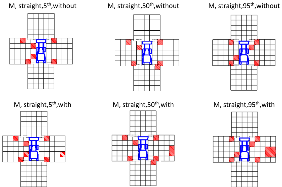
Figure 15 Visibility results for Tractor 1 at the man height for the straight sitting position.
