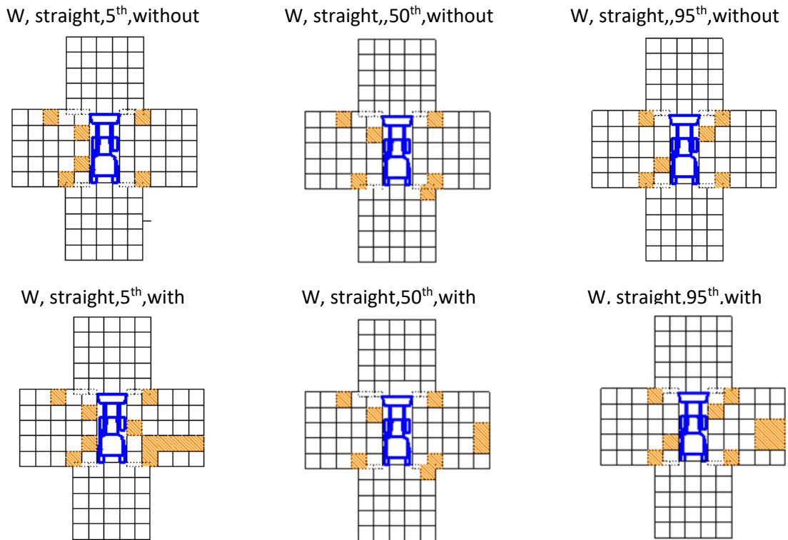
Figure 14 Visibility results for Tractor 1 at the woman level for a straight sitting position.
