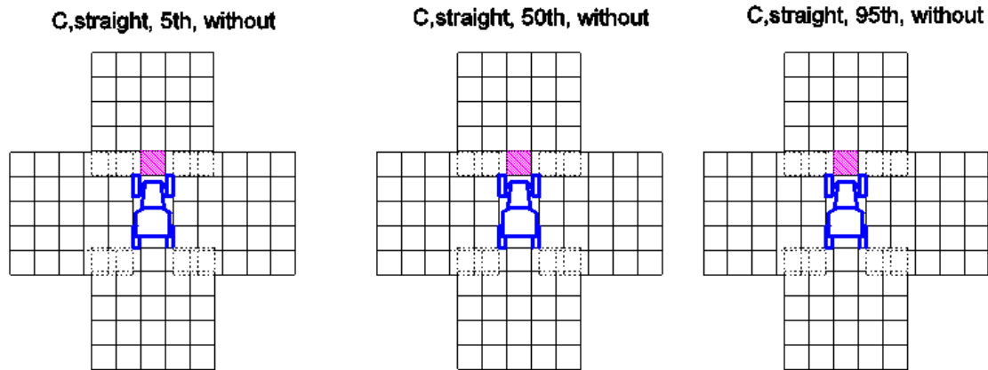
Figure 19 Visibility results for Tractor 2 at the child height for the straight sitting position.
