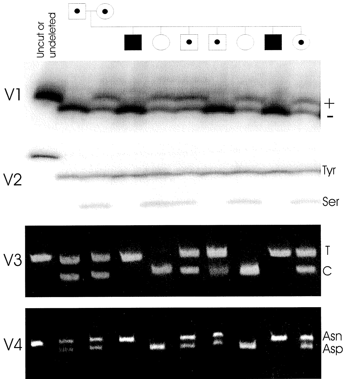
Figure 8: Segregation of the four LGMD2H variants. V1 is a simple size difference whereas the assays for V2-V4 are based on restriction fragment lengths. The nucleotide change in V2-V4 abolishes a restriction site in all cases leading to a larger fragment. Note a secondary control site is present on the V2 fragment leading to a larger uncut control. See text for descriptions of each assay.
