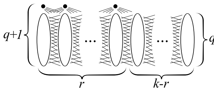
Figure 6.1: The Turán graph T(n, k)
