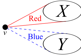
Figure 2.2: Proving the Erdős-Szekeres recursion
