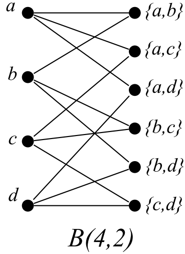
Figure 5.6: A sample graph of the form B(d, m) .
