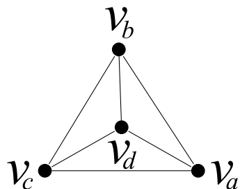
Figure 2.5: The ccw triangle (v_a, v_b, v_c) containing v_d .
