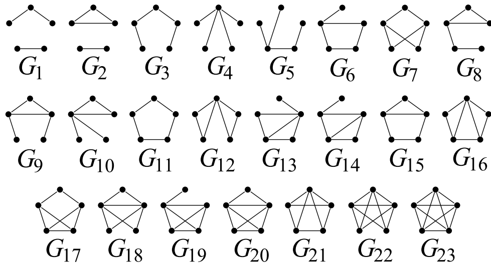
Figure 4.3: Graphs with exactly five vertices and no isolated vertices
