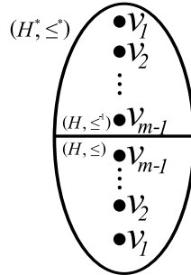
Figure 5.10: The graph (H^*, \leq^*)
