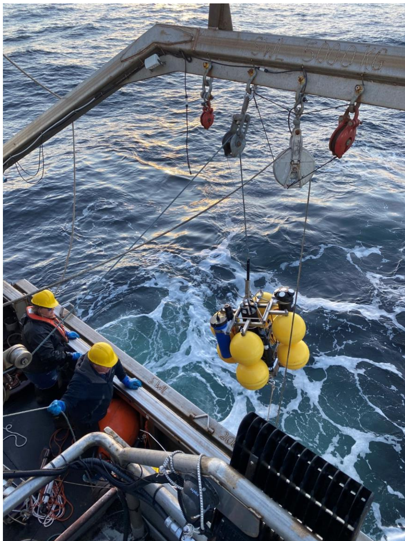
Figure 18. Mooring deployment from the stern of the William Kennedy using the A-frame.
