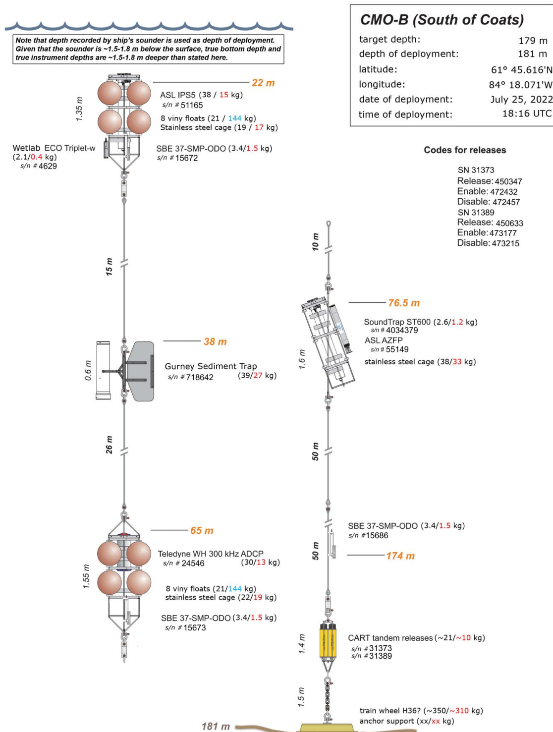
Figure 11. Configuration and instrument serial numbers for mooring CMO-B.
