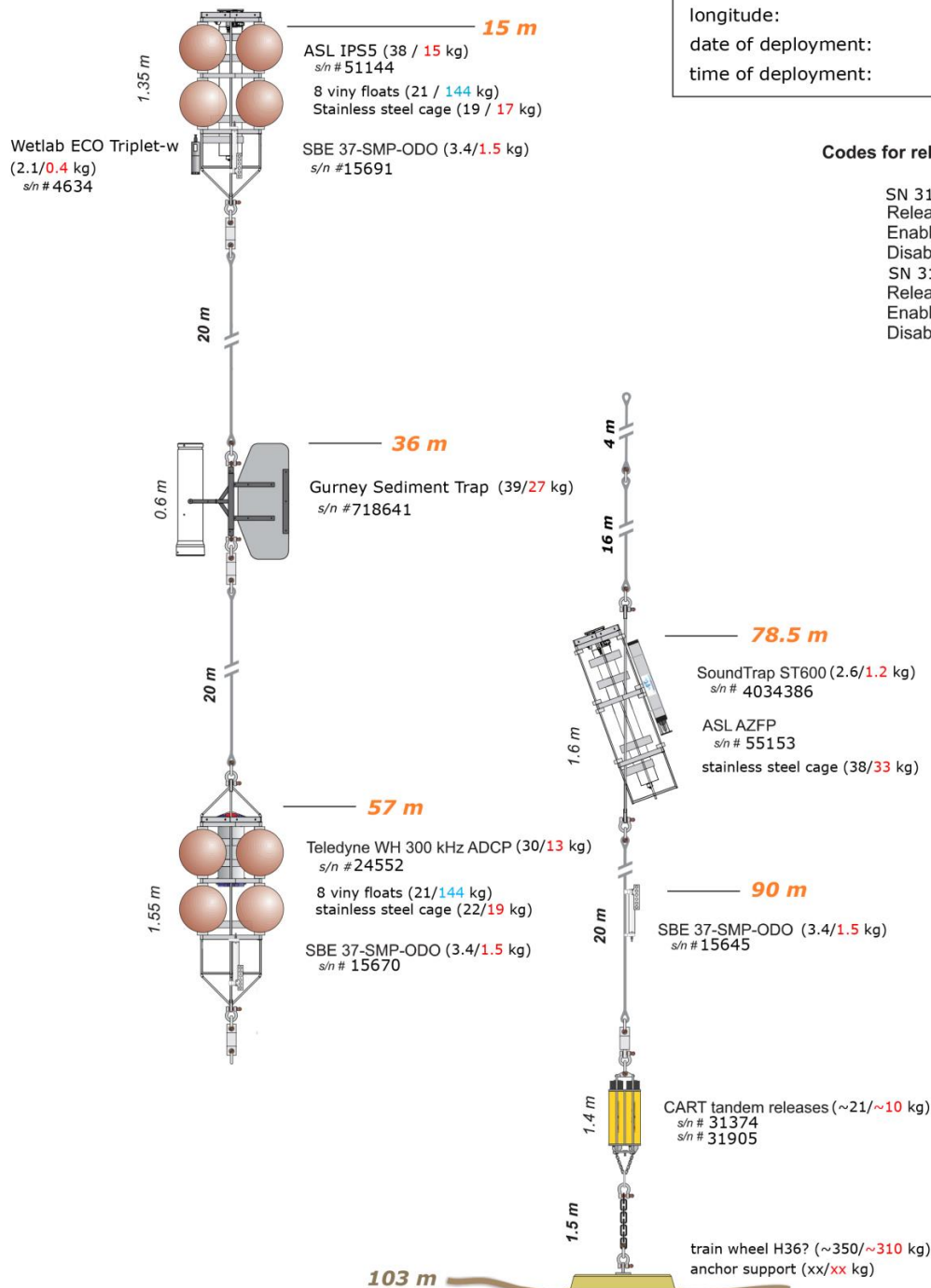
Figure 12. Configuration and instrument serial numbers for mooring CMO-A.
