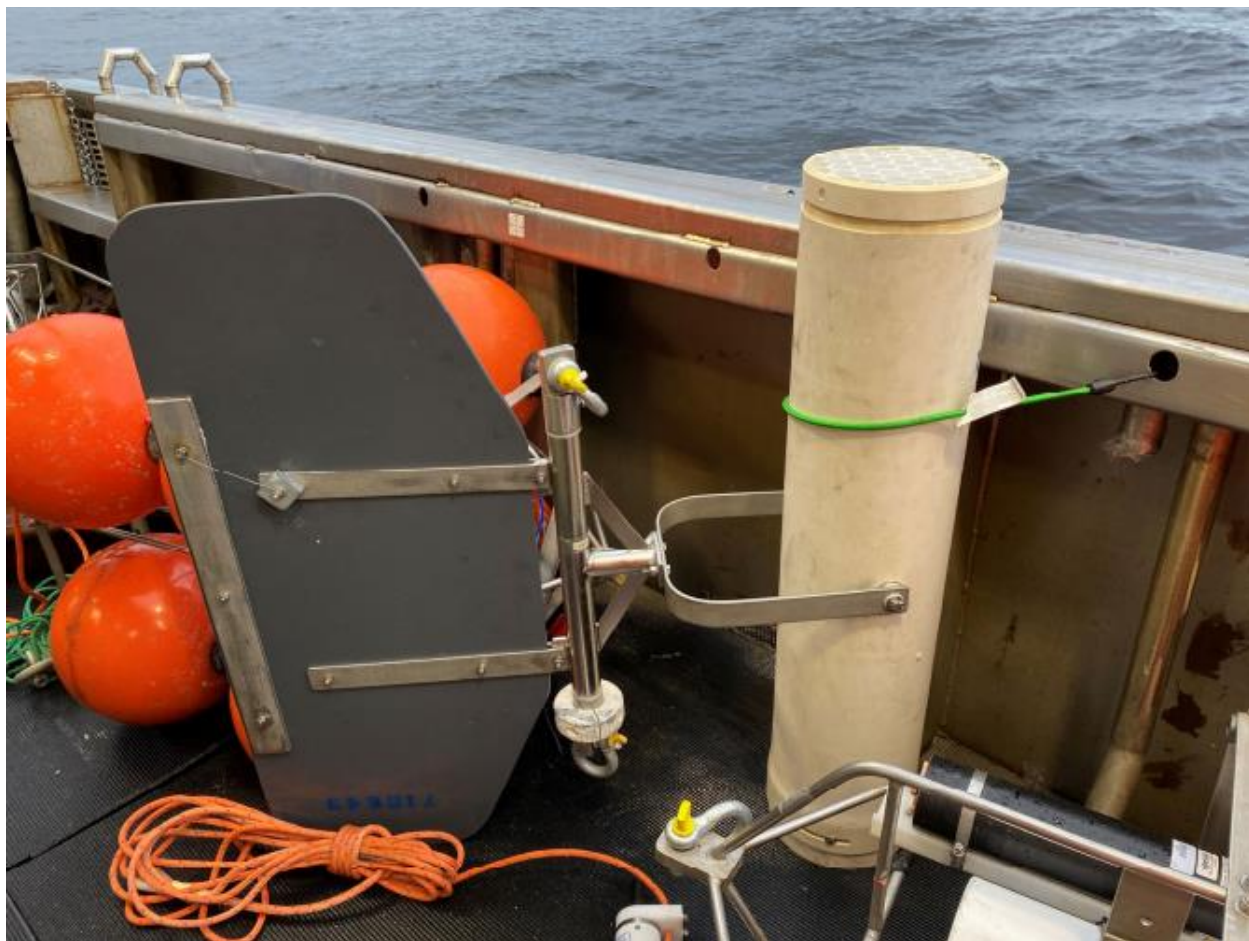
Figure 16. Baker-style sediment trap by Gurney Instruments, assembled on stern deck prior to deployment.
