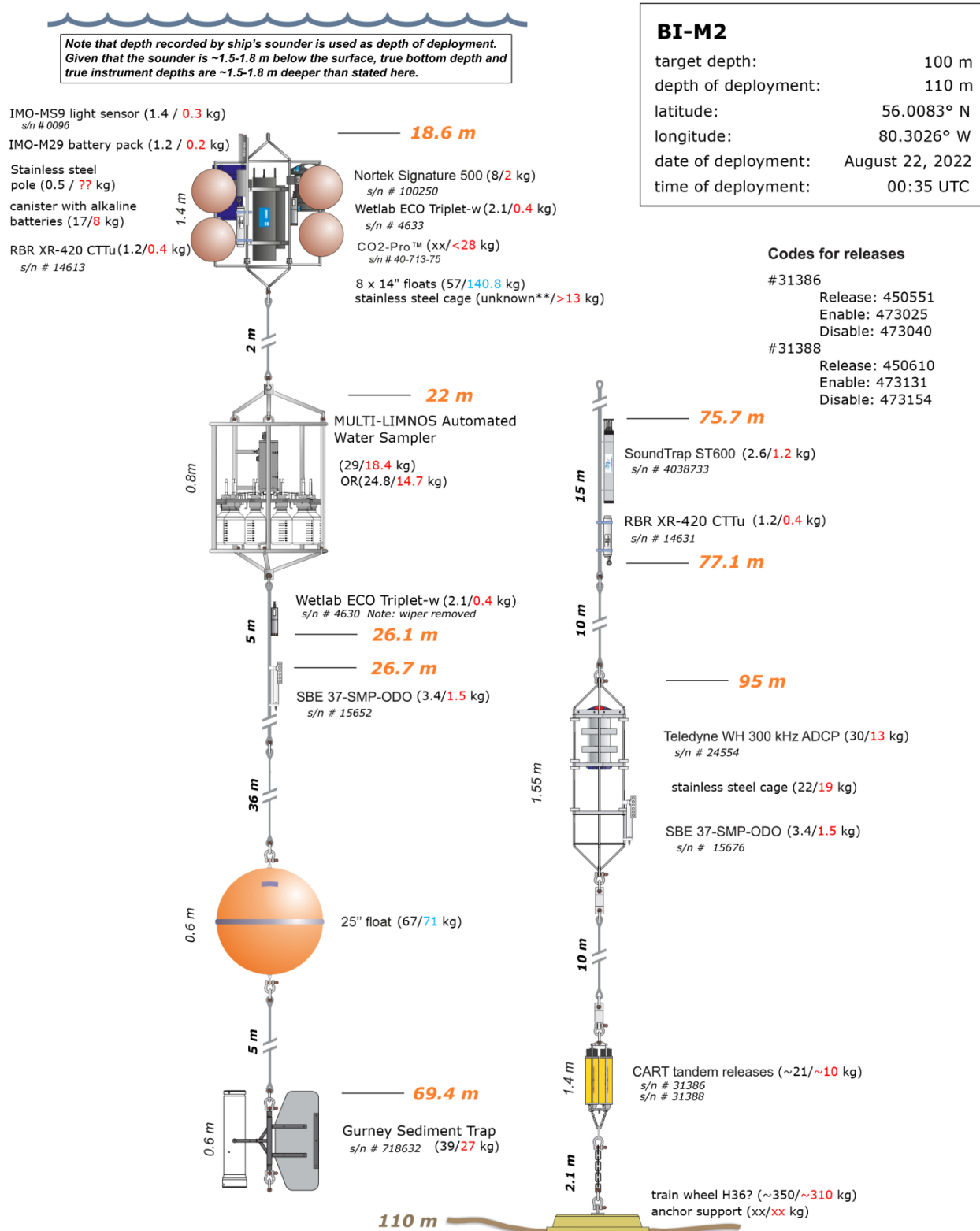
Figure 15. Configuration and instrument serial numbers for mooring BI-M2.
