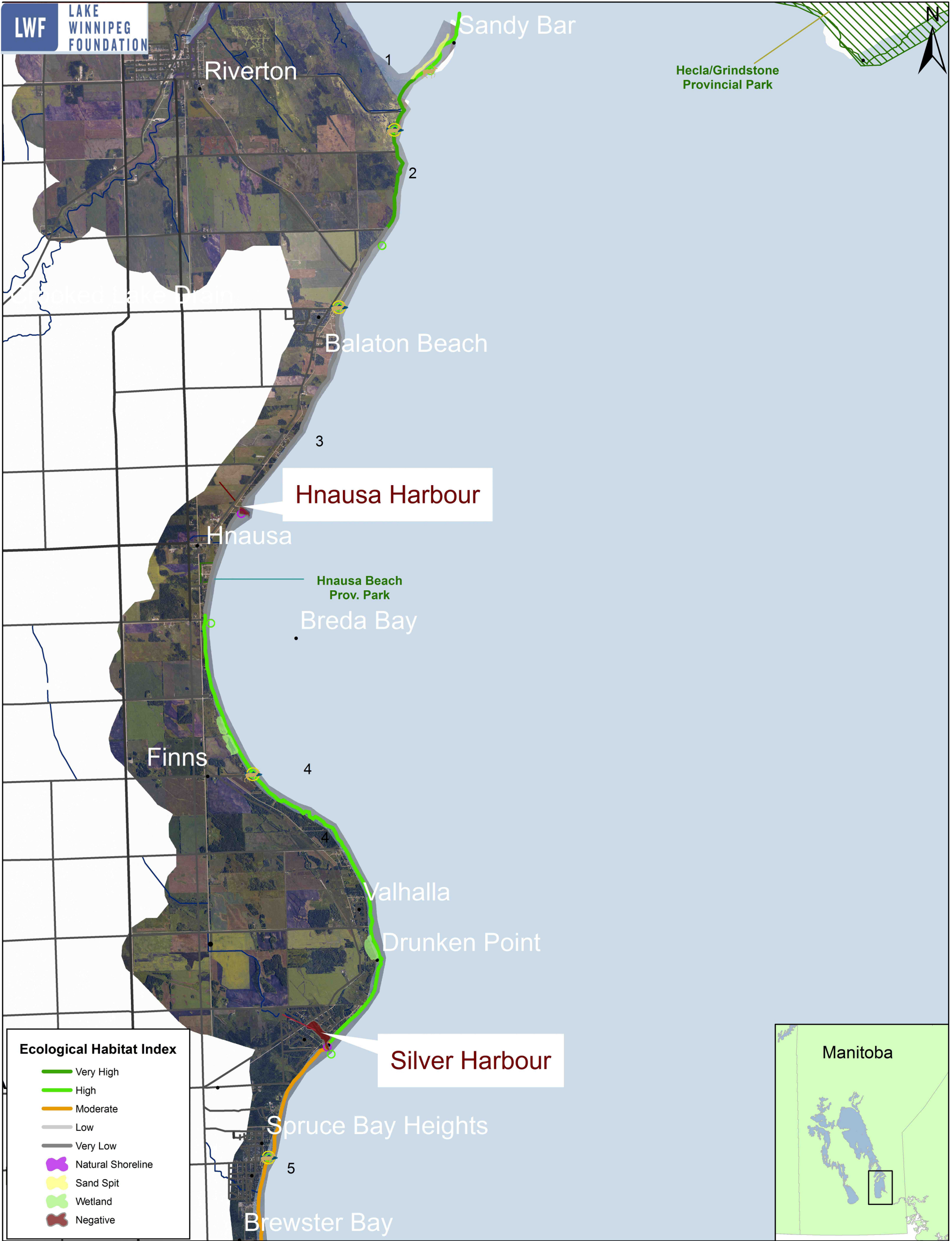
Lake Winnipeg South Basin, Segments 1 - 5 Sensitive Habitat Inventory and Mapping (SHIM): Composite Map With Ecological Habitat Index for Lake Shore Segments (Aerial Photo)
