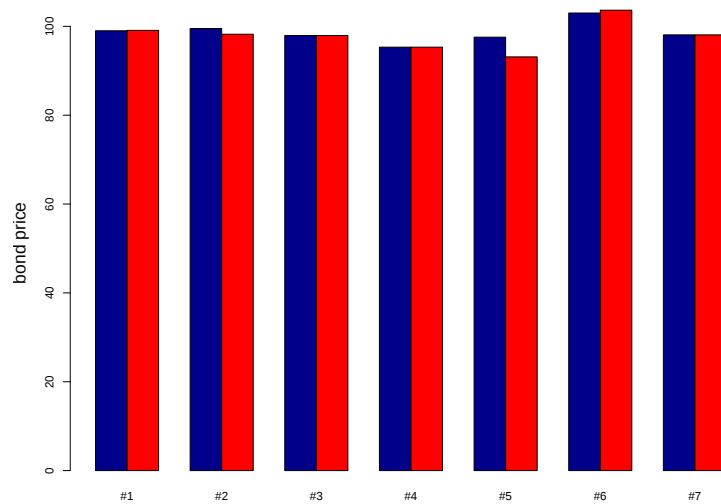
Figure 3.3: Calibration results for RBS. The blue bars represent bonds' market prices and the red bars represent bonds' dirty prices with \beta_{\text{RBS}}^* = (0.0210, 0.0170, 0.0676, 4.9448)^\top . The mean absolute error is 0.923.
