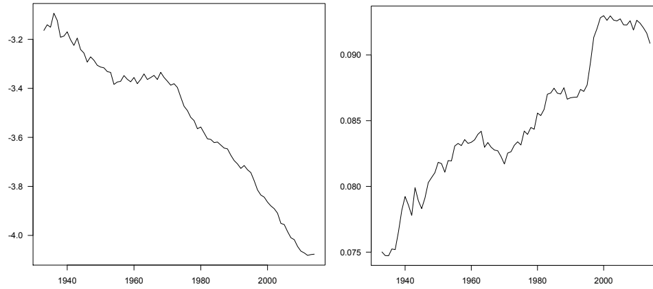
Figure 2.1: Historical values of \kappa_t^{(1)} (left panel) and \kappa_t^{(2)} (right panel) for US male population aged from 30 to 100, 1933–2014
