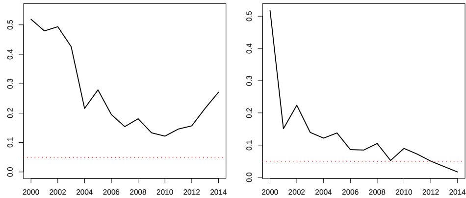
Figure 2.3: The various-horizon p -values of realized \kappa_t^{(1)} (left panel) and \kappa_t^{(2)} (right panel) in 2000–2014 based on the mortality indexes from 1933 to 1999. The red dotted line represents the 5% significance level.
