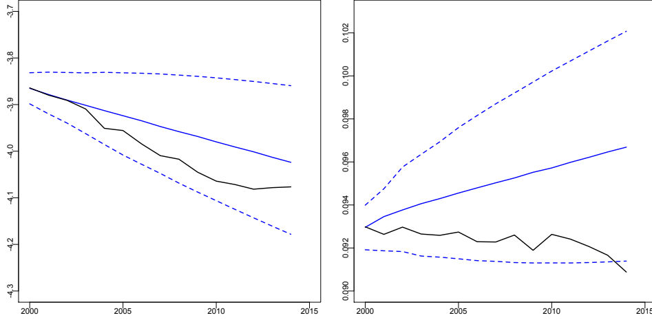
Figure 2.2: The 95% prediction interval and median line of \kappa_t^{(1)} (left panel) and \kappa_t^{(2)} (right panel) in 2000–2014 based on the mortality indexes from 1933 to 1999. The dashed lines represent lower and upper bounds of the confidence interval, the blue solid line represents the forecasted median, and the black continuous line represents the real outcome of the mortality index.
