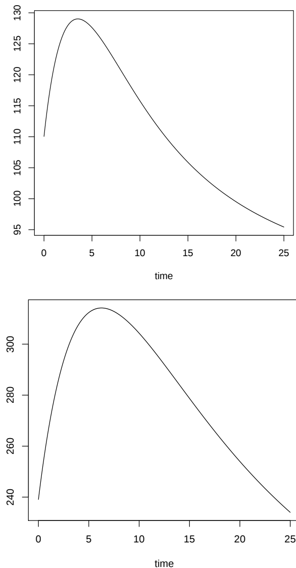
Figure 3.4: Estimated credit spread term structure of JPM (upper panel) and RBS (lower panel) on June 16, 2016
