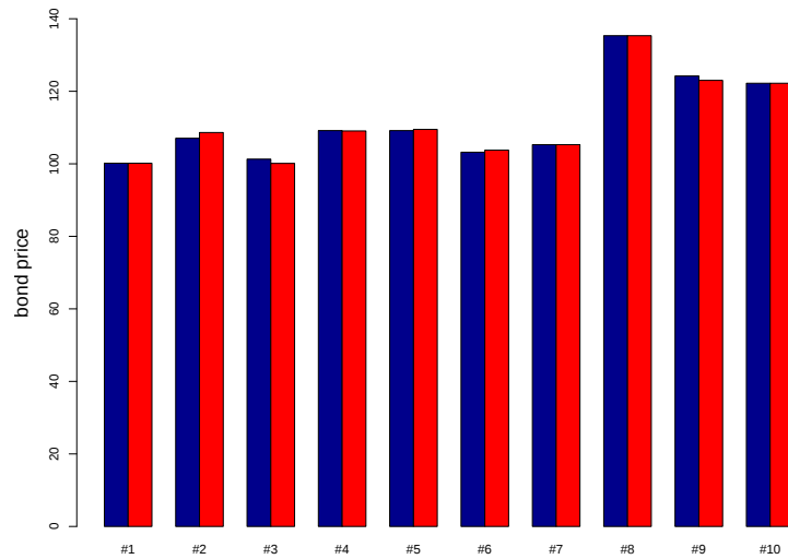
Figure 3.2: Calibration results for JPM. The blue bars represent bonds' market prices and the red bars represent bonds' dirty prices with \beta_{\text{JPM}}^* = (0.0125, 0.0050, 0.0181, 2.8895)^\top . The mean absolute error is 0.496.
