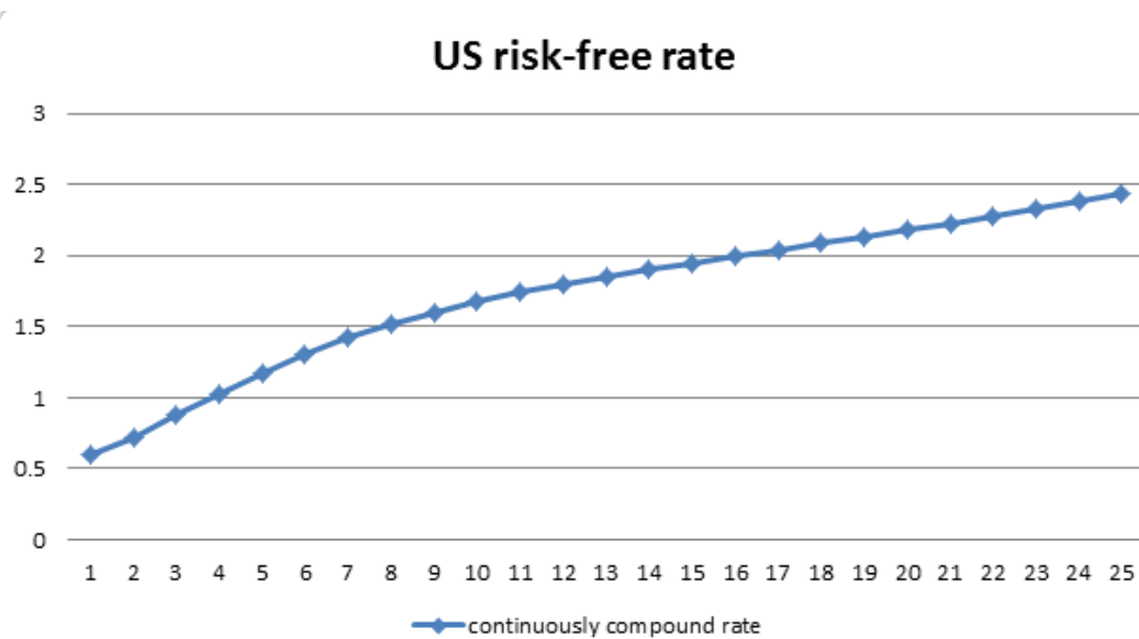
Figure 3.1: 25 year US Treasury zero yields on June 16, 2016
