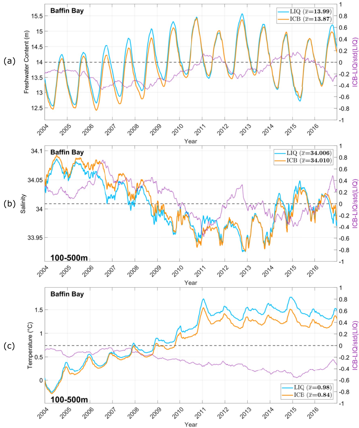
Figure 6. Baffin Bay averaged (a) Freshwater content; (b) Salinity at 100–500 m; and (c) Temperature at 100–500 m. The blue (orange) line shows LIQ (ICB) time series, and the dotted purple line shows their difference with respect to LIQ’s variability. The numbers indicated by \bar{x} are the corresponding simulation’s time average for the variable in question.
