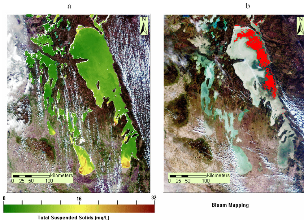
Figure 4. Products generated from MODIS data: a) total suspended solids concentration for May 17, 2006, and b) surface algal bloom distribution for September 20, 2006. The background is the composite true colour images; the TSS is colour coded; cloud over water body is masked with white colour.
