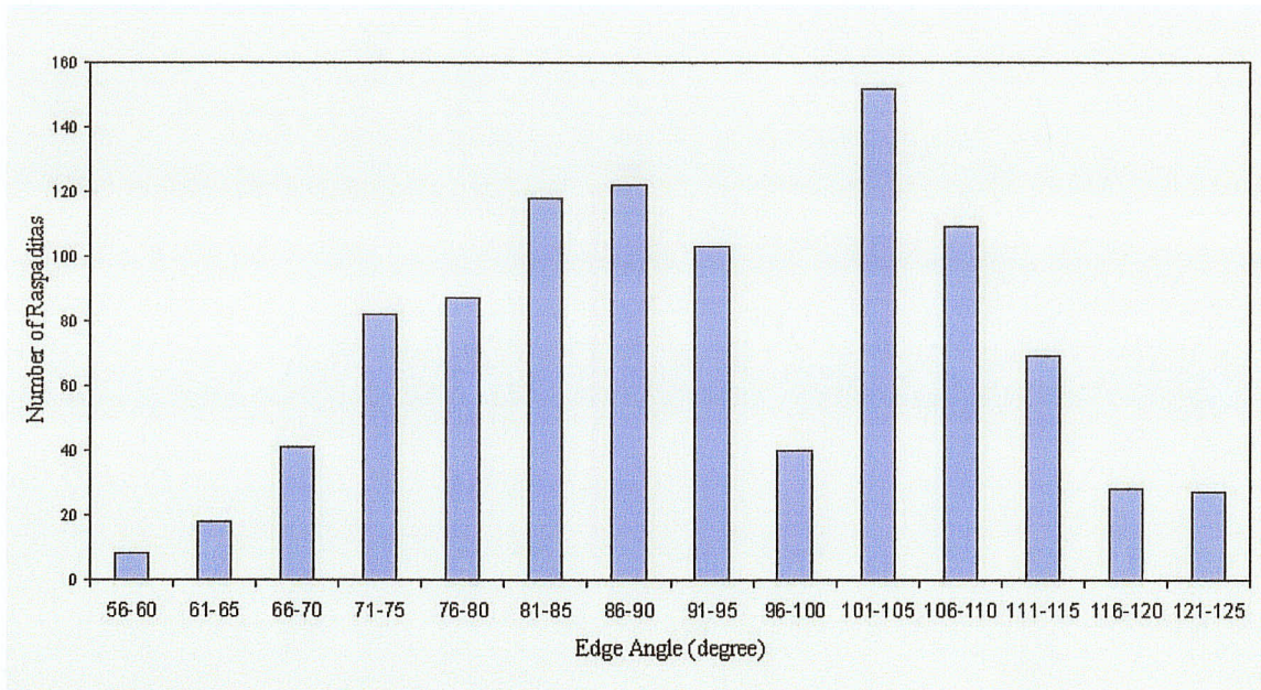
Figure 6.9 Histogram of raspadita edge angles.
