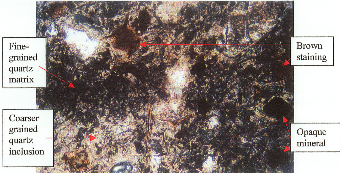
Figure 6.46: JD.09.04 sample 3, plane polarized light, 2.5x magnification. Note: The width of field of view is 5 mm across.
