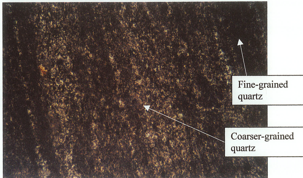
Figure 6.42: Drill RI1000.6 in plane polarized light under 2.5x magnification. Note: The width of field of view is 5 mm across.
