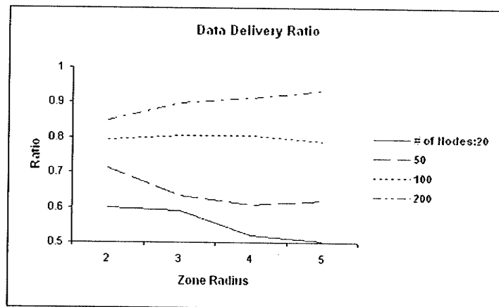
Figure 5.5: Delivery Ratio with Various Zone Radius
