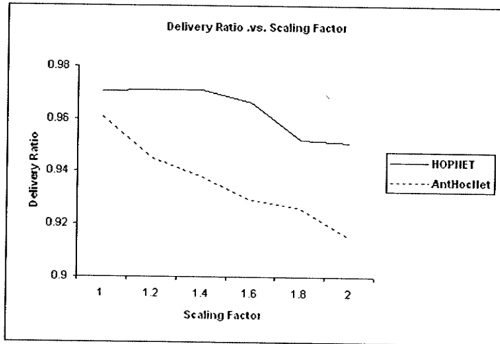
Figure 5.11: Data Delivery Ratio .vs. Scale of the Problem
