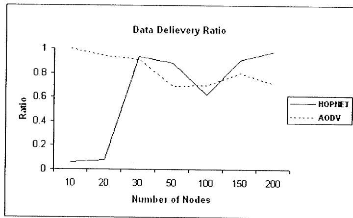
Figure 5.2: Delivery Ratio
