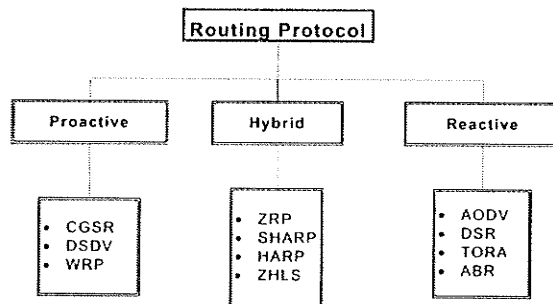
Figure 2.1: Routing Protocols
