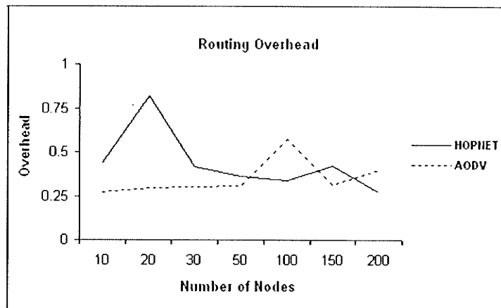
Figure 5.3: Overhead
