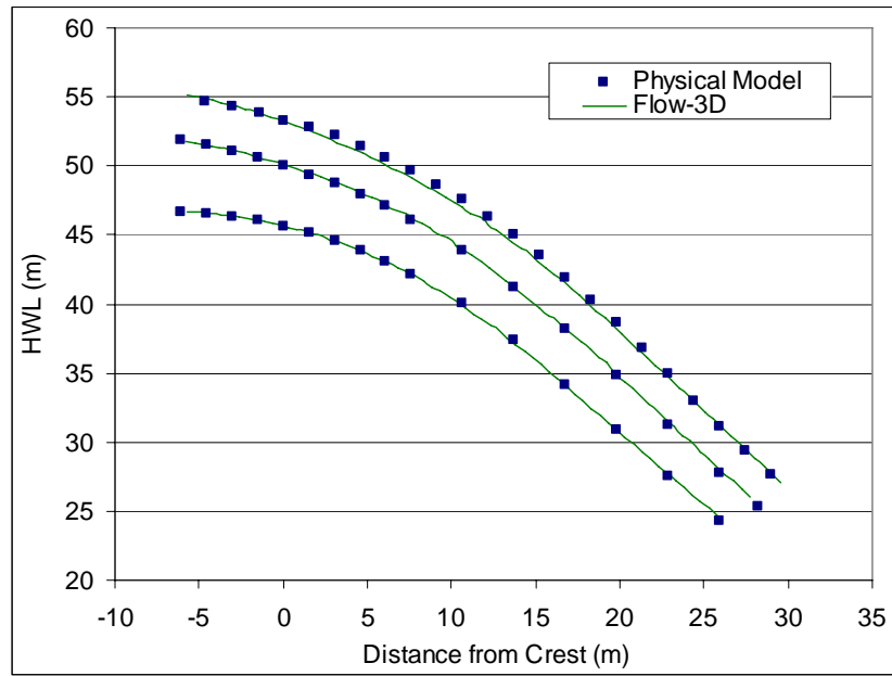
Figure 4.8 Comparison of measured physical model water surface profiles for the Conawapa-like spillway to data obtained with Flow-3D for 3 different headwater levels.
