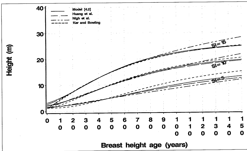
Figure 4.13. Model [4.2], Nigh et al. (2002), Huang et al. (1994) and Ker and Bowling (1991) height –age curves for black spruce plotted against breast height age for site indices 5, 10 and 15 m.
