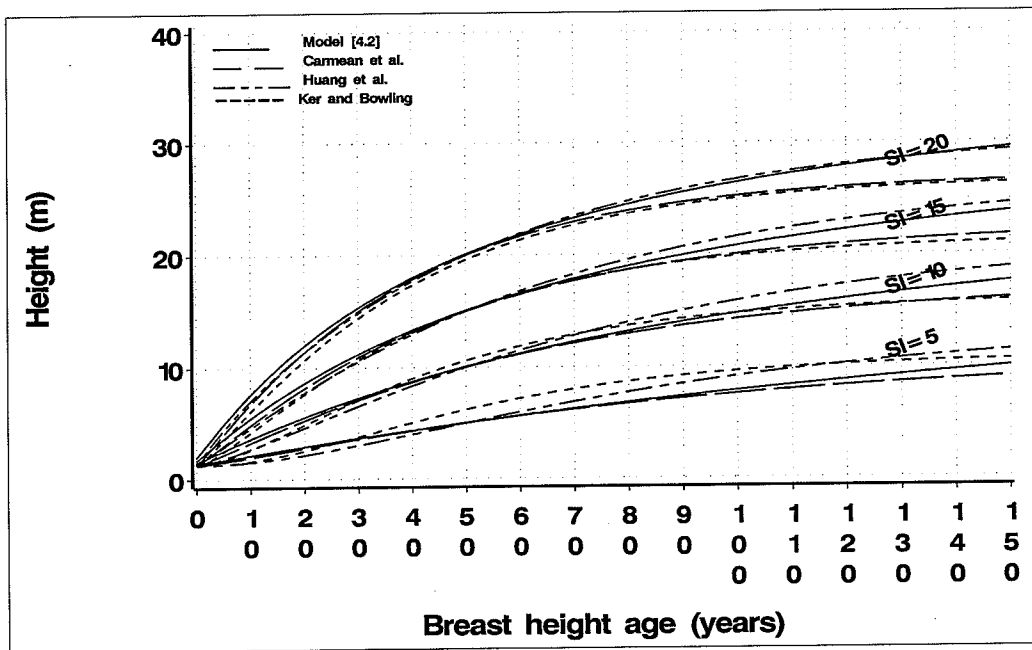
Figure 4.14. Model [4.2], Huang et al. (1994), Ker and Bowling (1991) and Carmean (2001) height –age curves for jack pine plotted against breast height age for site indices 5, 10, 15 and 20 m.
