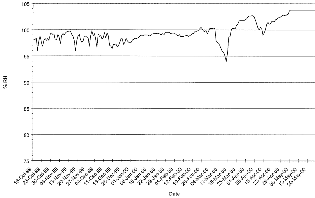
Figure 17: Mean daily relative humidity in Microwave Cave from Oct 16, 1999 to May 28, 2000.
